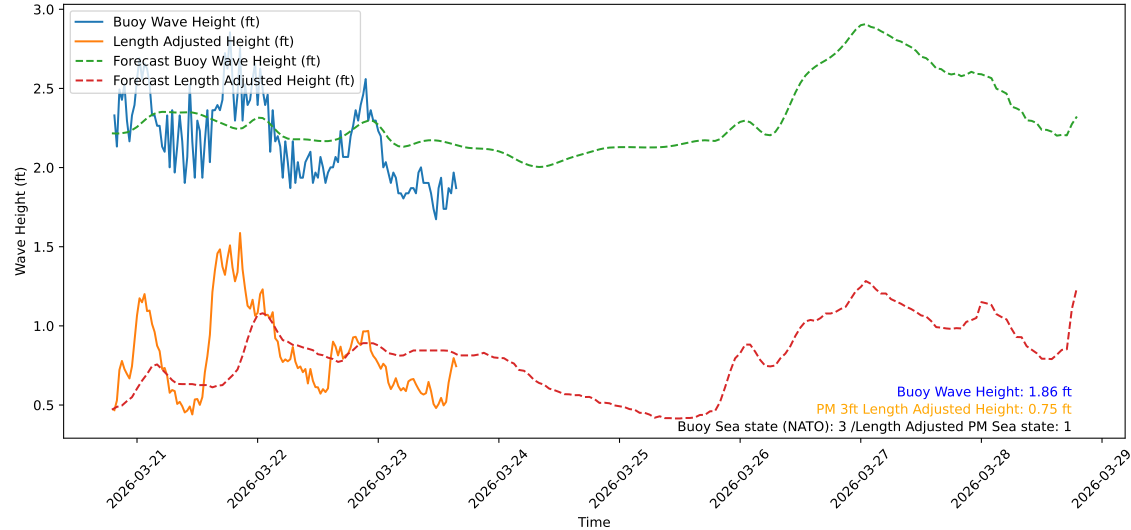
Wave Heights over Time for Red Beach at 2026-03-23 19:20:47
