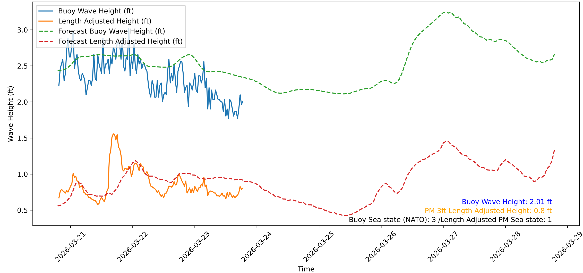
Wave Heights over Time for Oceanside Harbor at 2026-03-23 19:20:31
