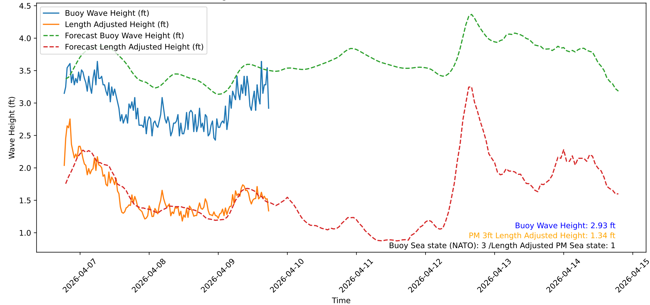
Wave Heights over Time for Oceanside Harbor at 2026-04-09 18:40:31
