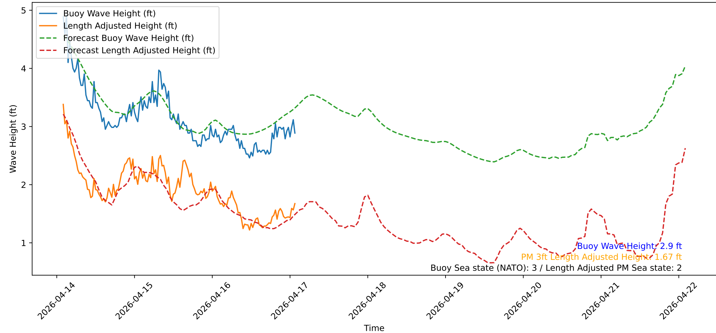
Wave Heights over Time for Green Beach at 2026-04-17 02:11:14
