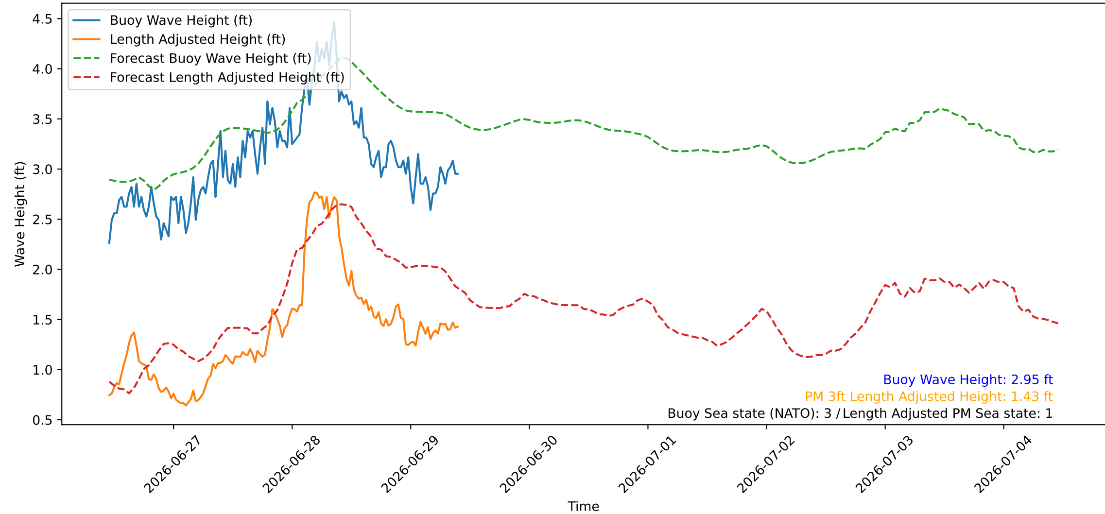
Wave Heights over Time for Red Beach at 2026-06-29 10:30:45
