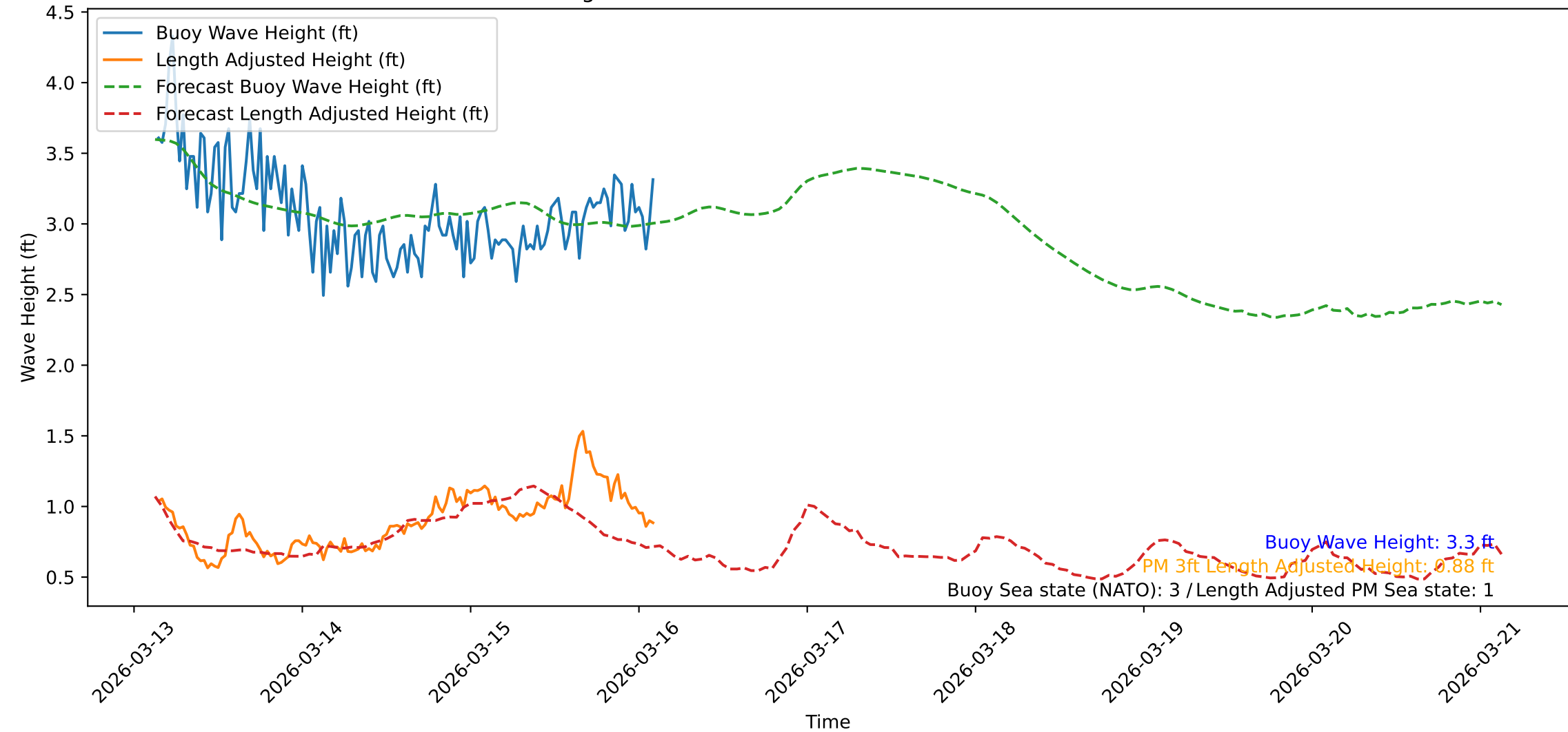
Wave Heights over Time for Red Beach at 2026-03-16 03:01:19
