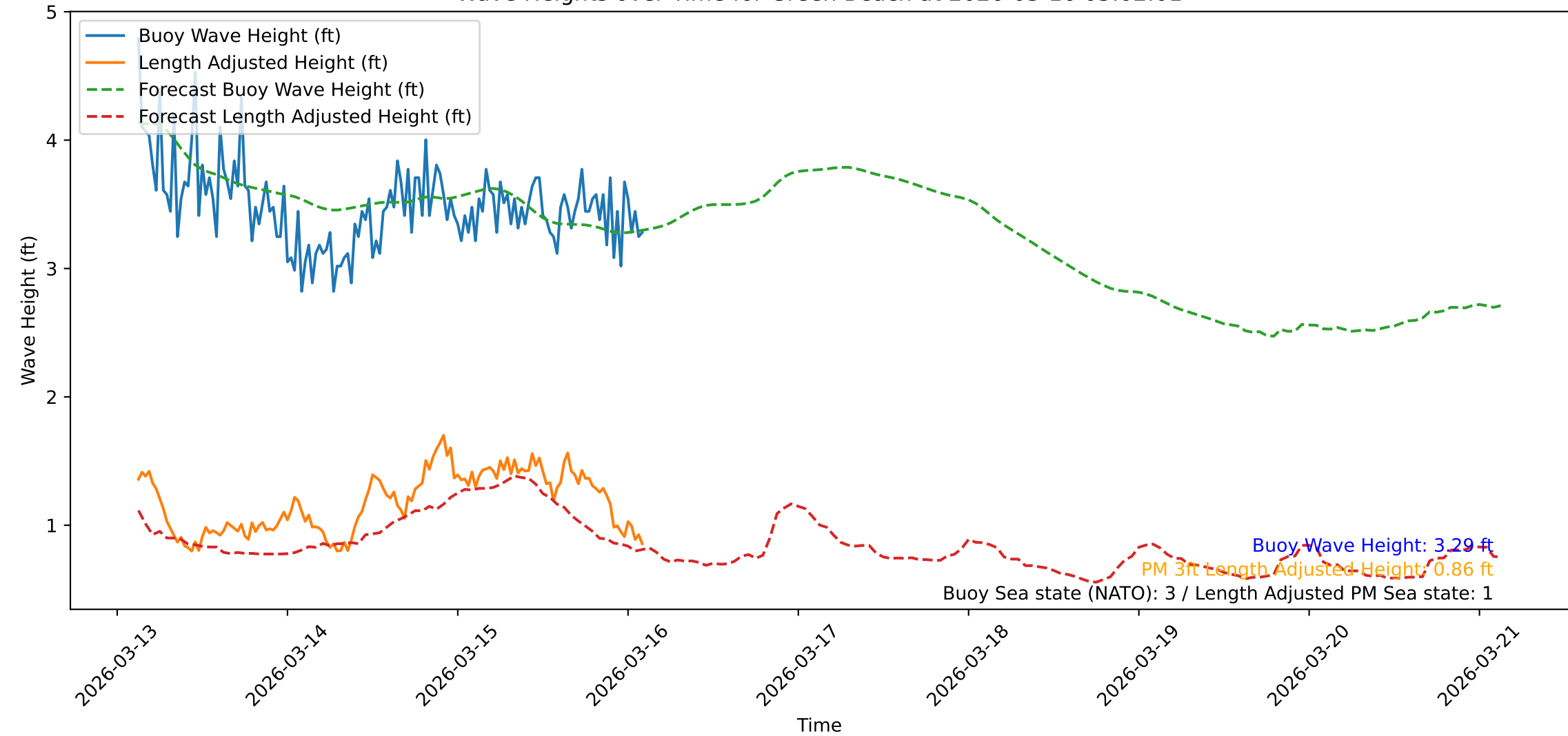
Wave Heights over Time for Green Beach at 2026-03-16 03:02:01
