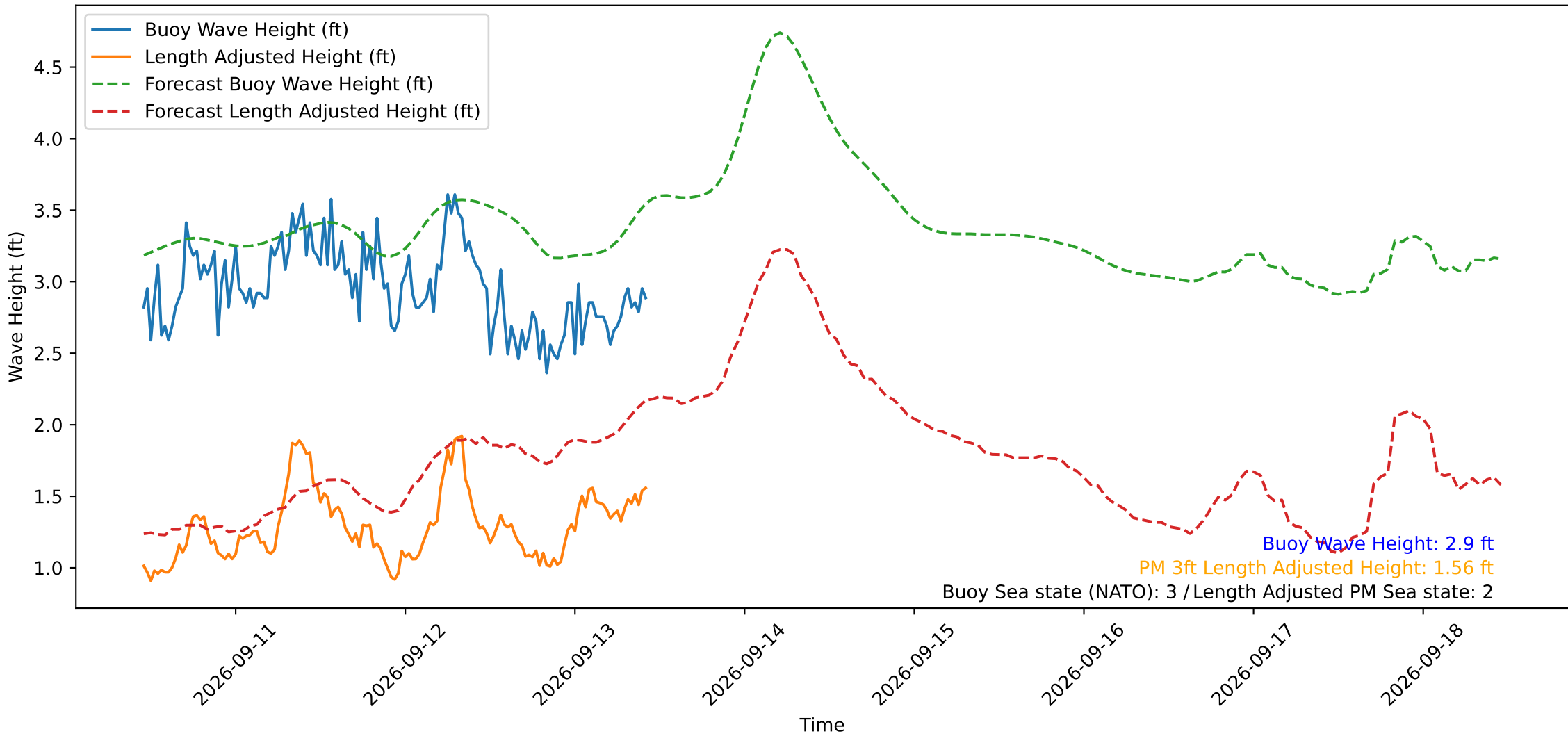
Wave Heights over Time for Green Beach at 2026-09-13 10:41:11
