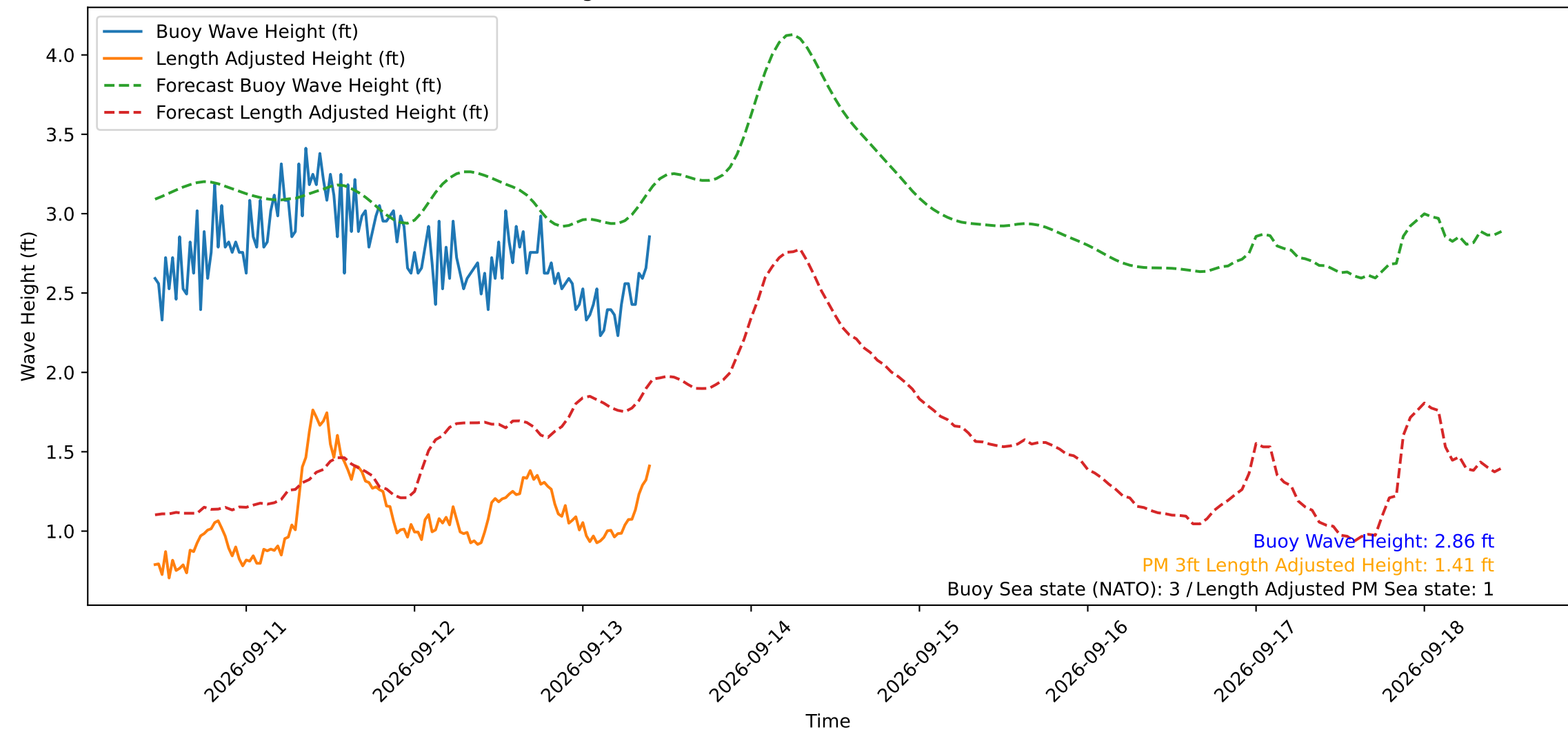
Wave Heights over Time for Red Beach at 2026-09-13 10:40:49
