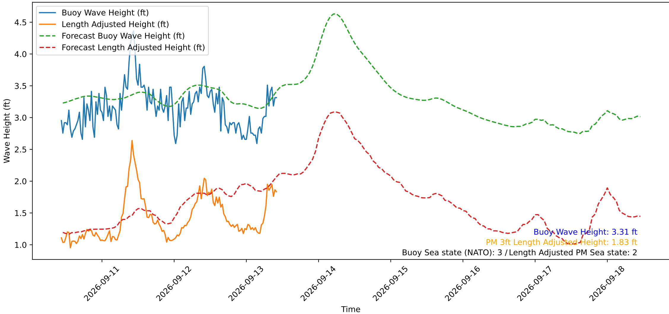
Wave Heights over Time for Oceanside Harbor at 2026-09-13 10:40:29
