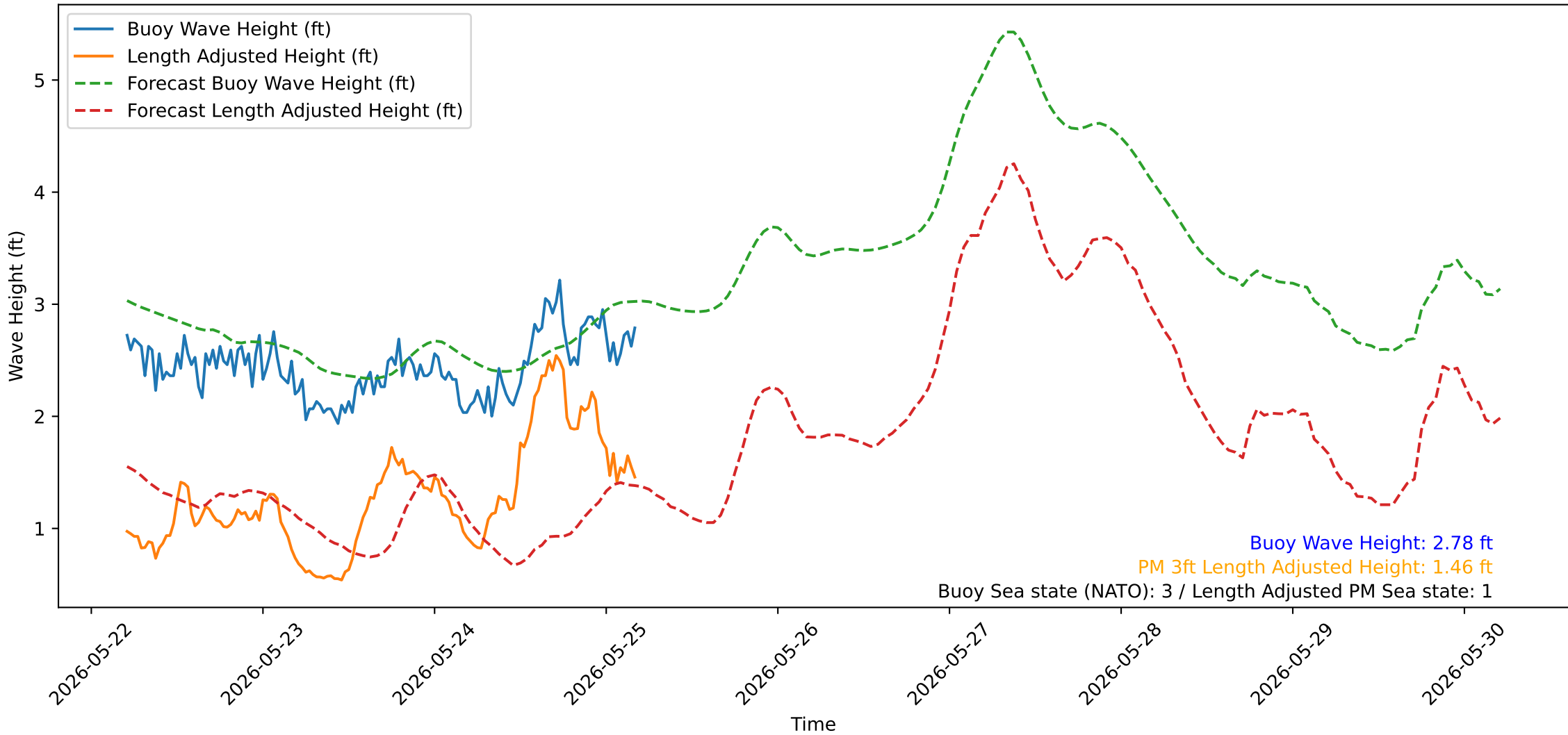
Wave Heights over Time for Red Beach at 2026-05-25 04:50:51
