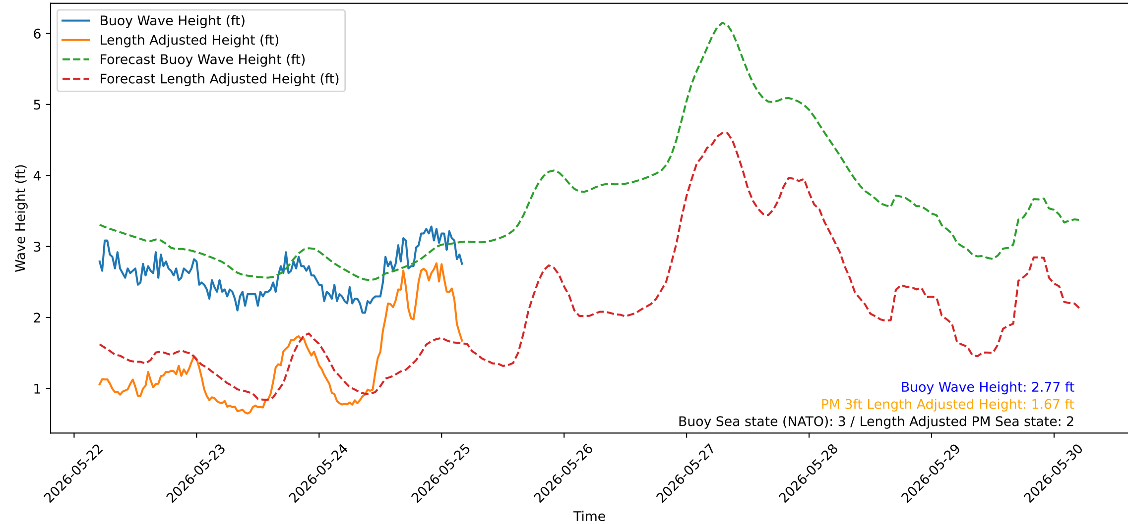
Wave Heights over Time for Green Beach at 2026-05-25 04:51:14
