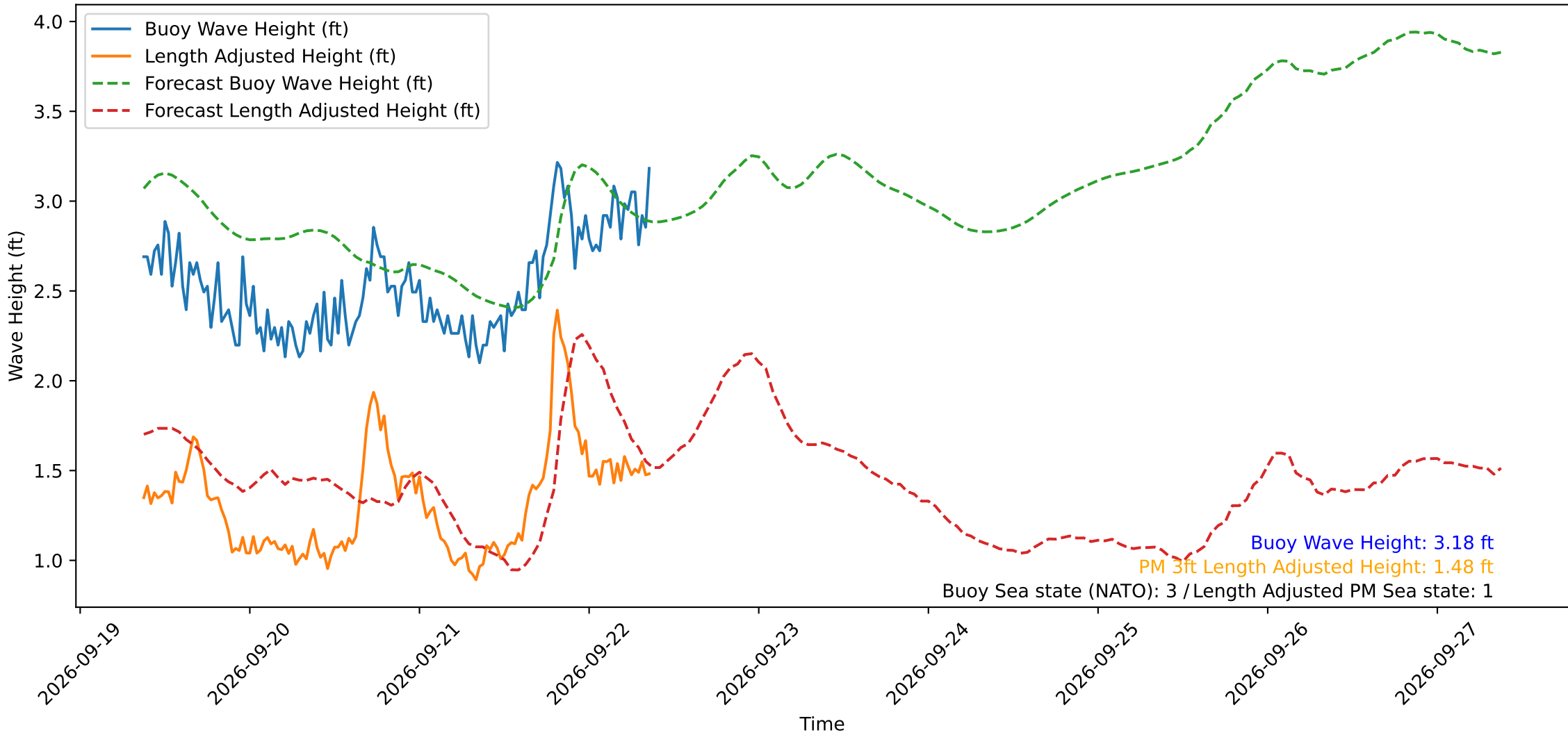
Wave Heights over Time for Oceanside Harbor at 2026-09-22 09:10:29
