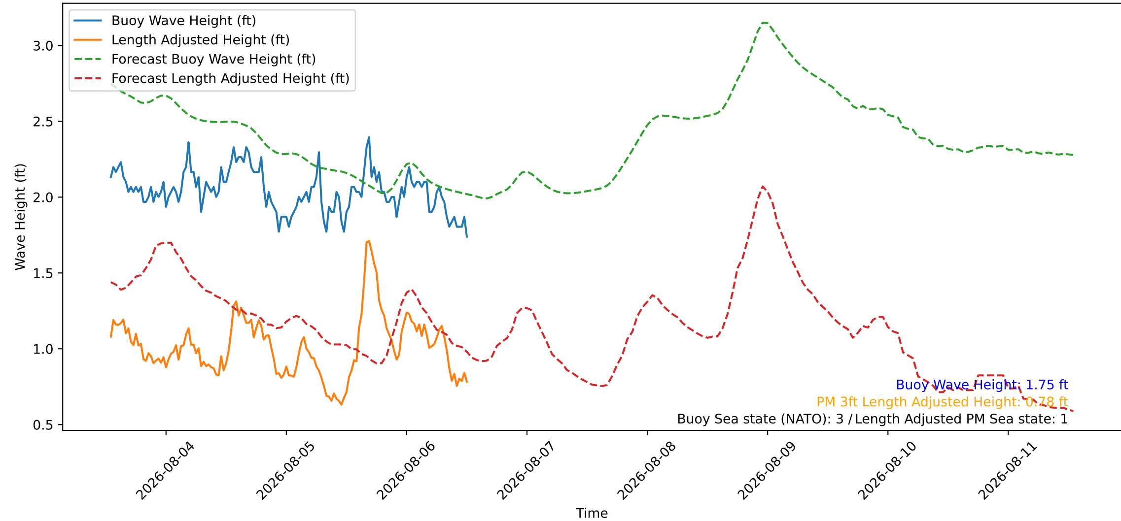
Wave Heights over Time for Red Beach at 2026-08-06 12:40:45
