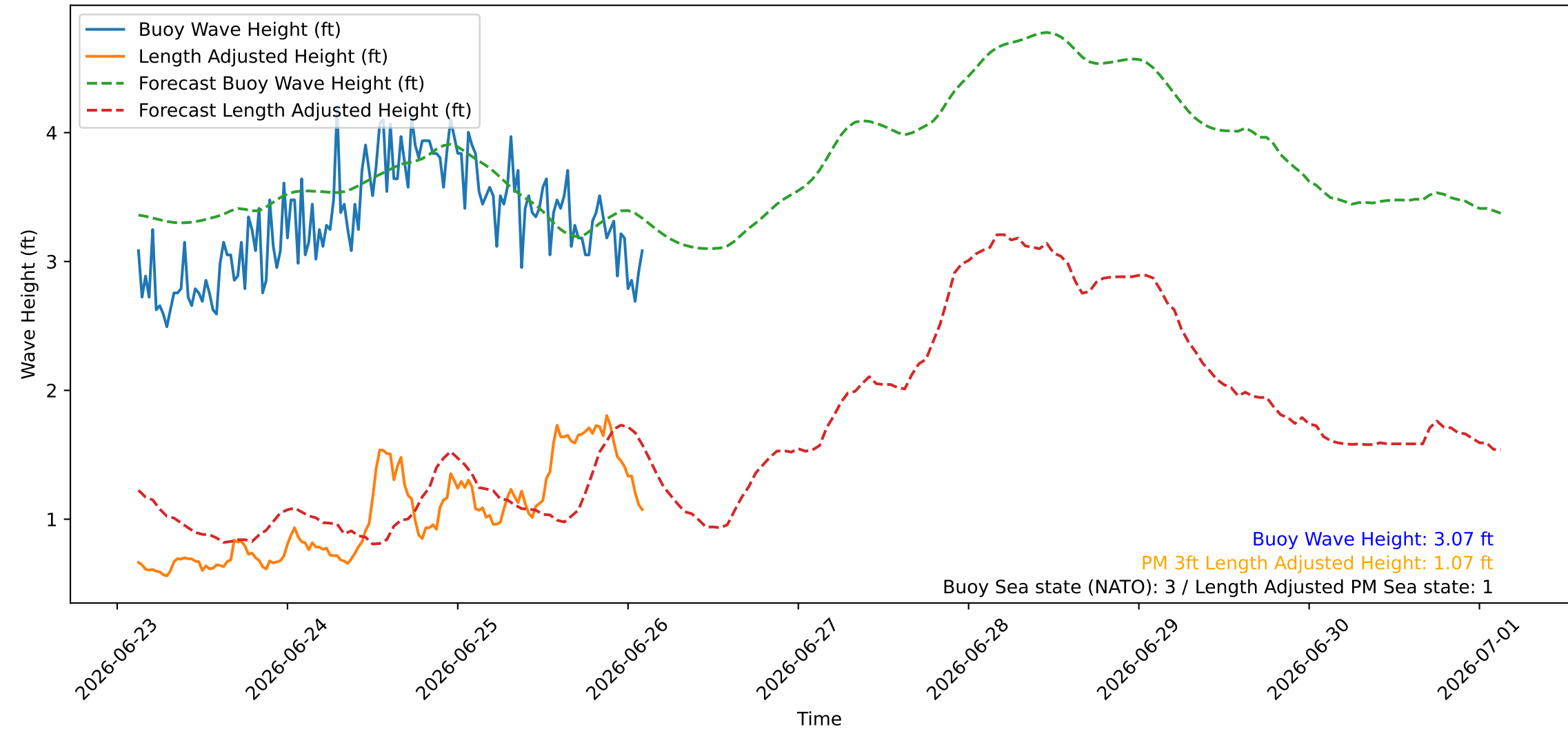
Wave Heights over Time for Green Beach at 2026-06-26 02:51:09
