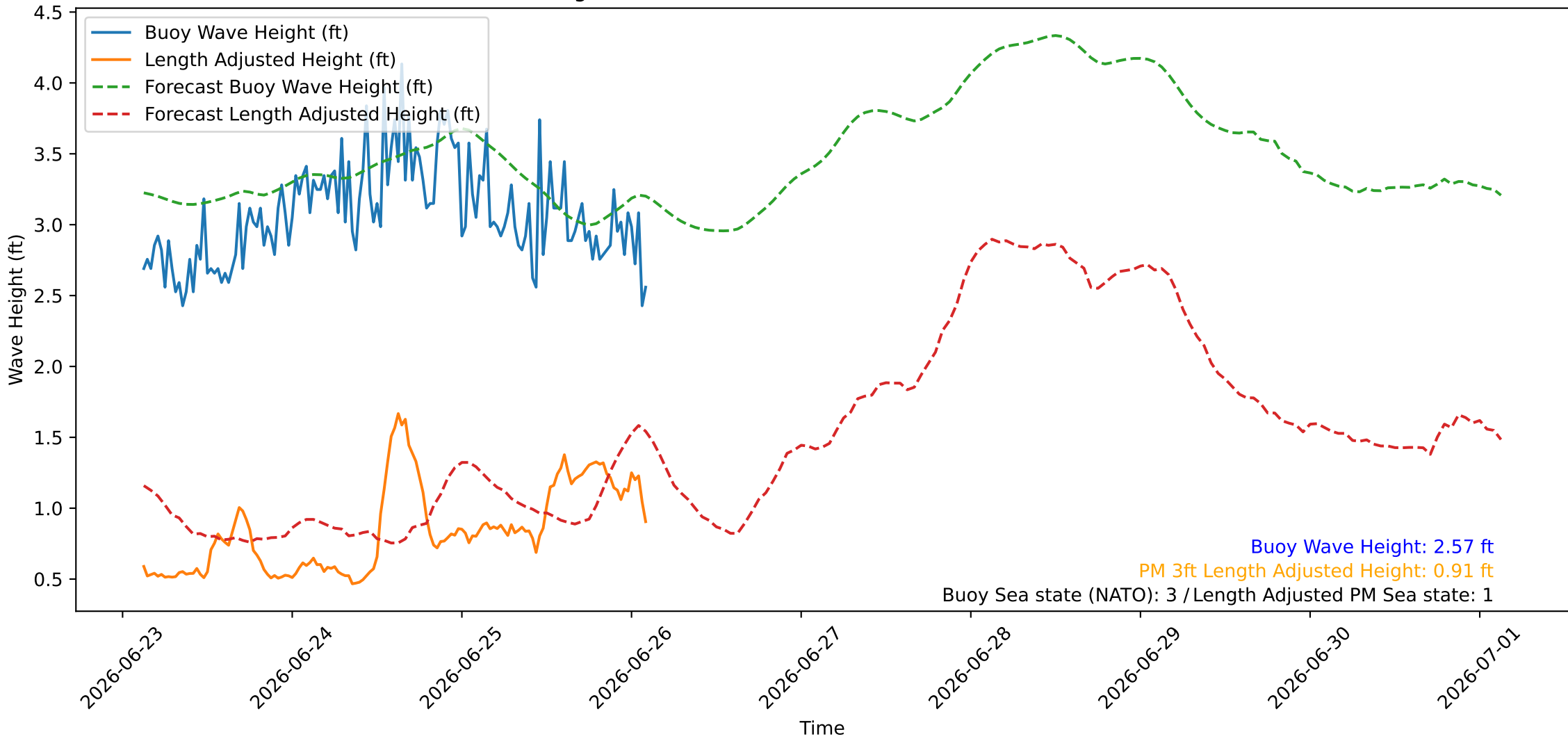
Wave Heights over Time for Red Beach at 2026-06-26 02:50:46
