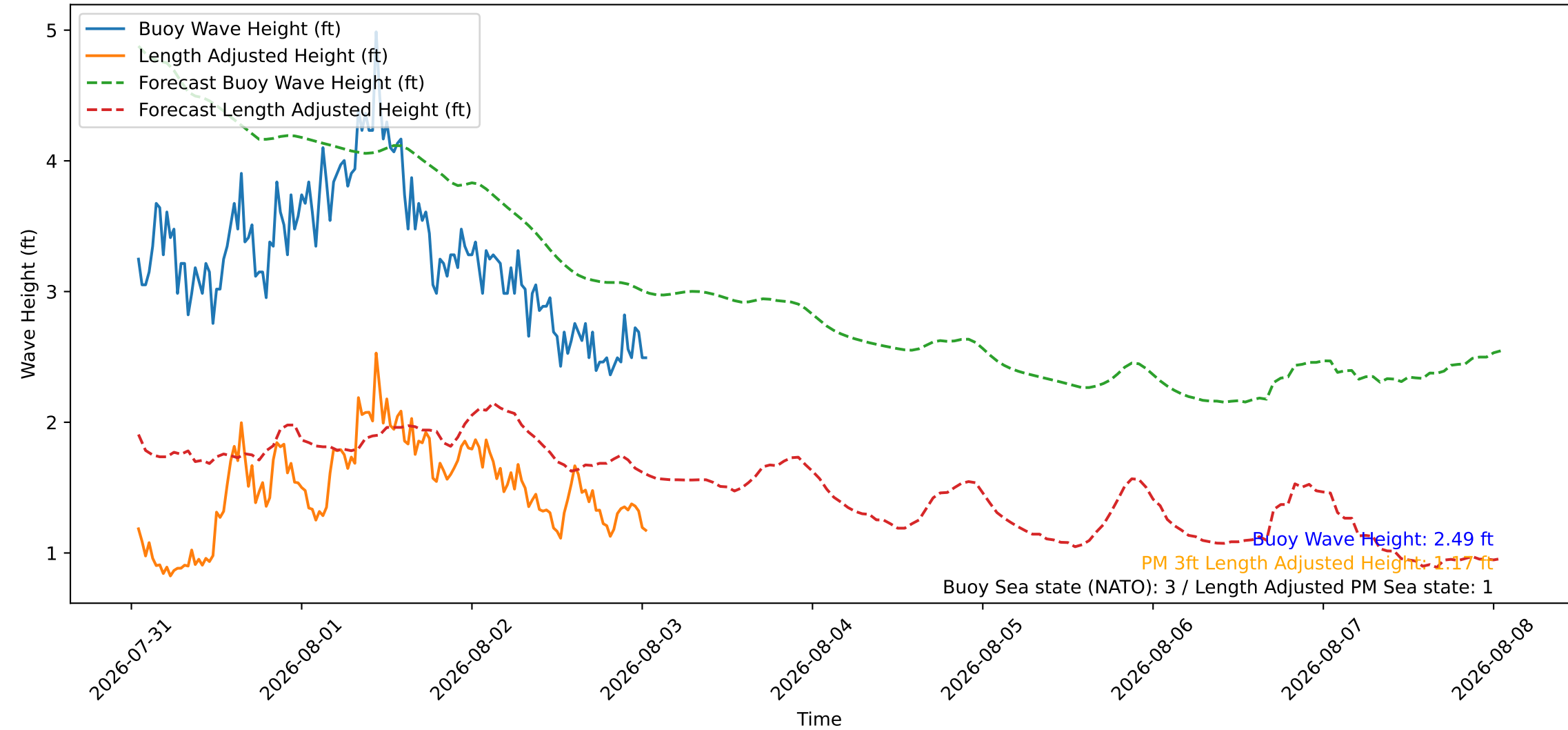
Wave Heights over Time for Green Beach at 2026-08-03 01:11:08
