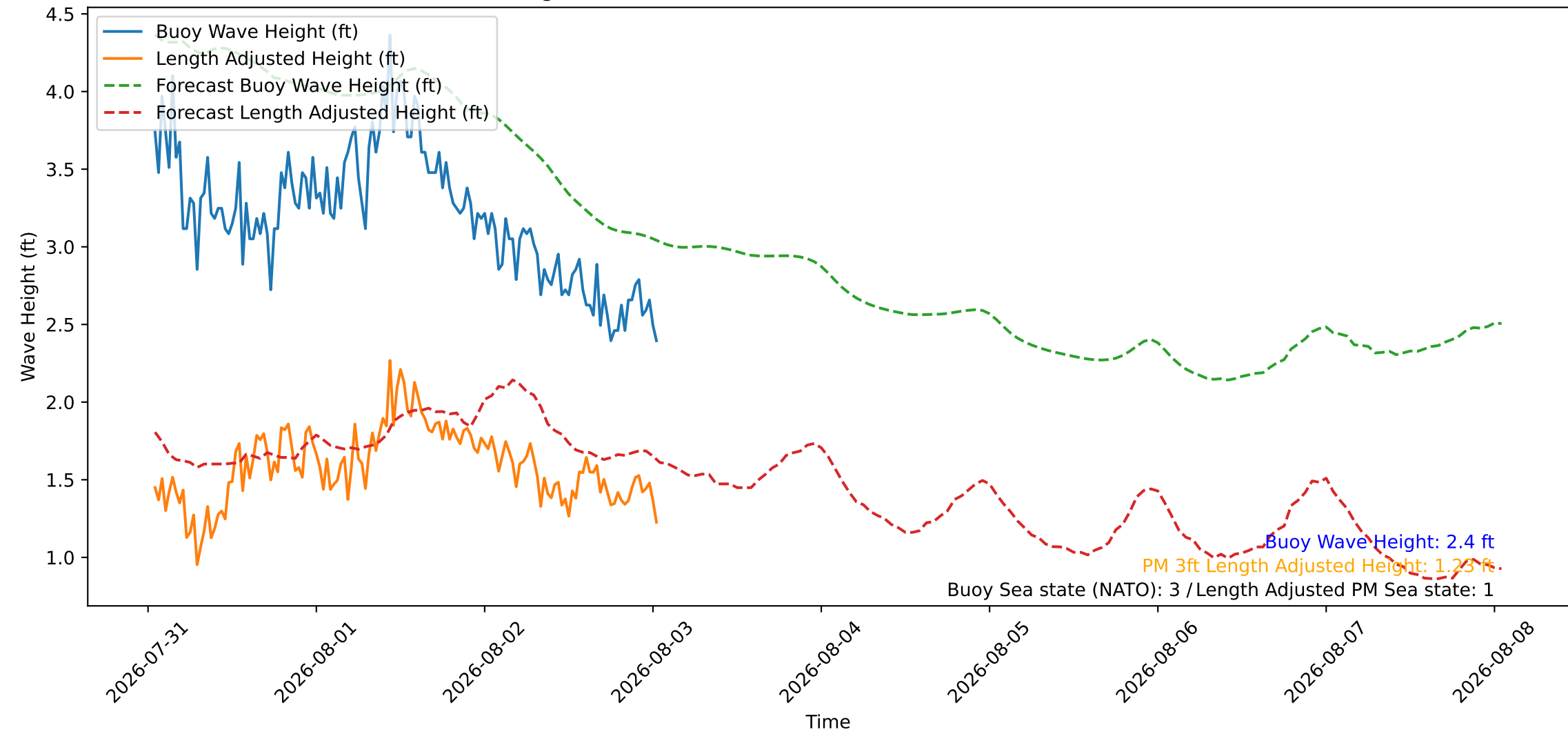
Wave Heights over Time for Oceanside Harbor at 2026-08-03 01:10:26
