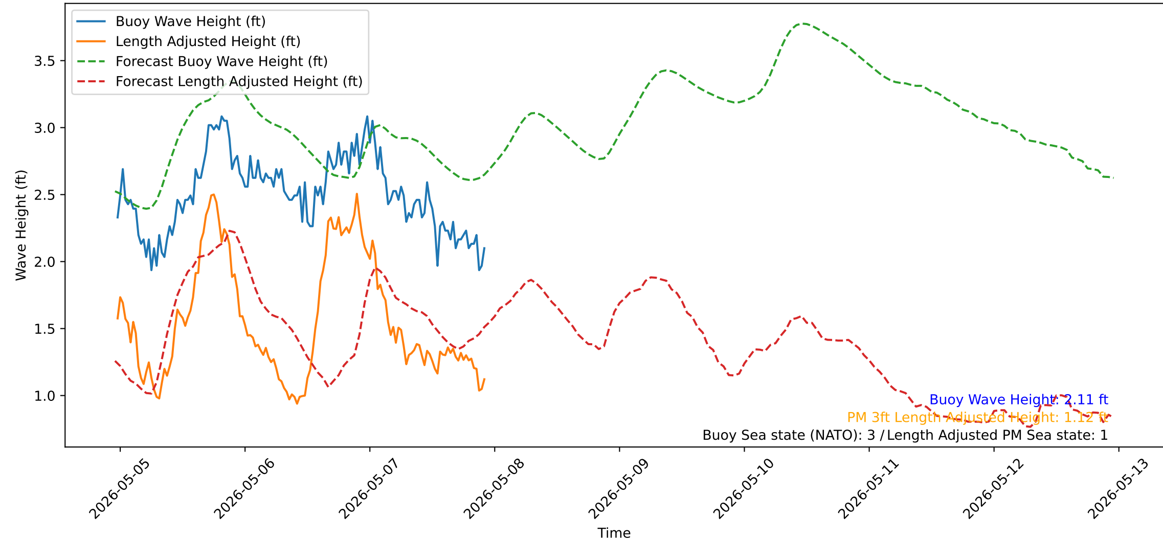
Wave Heights over Time for Red Beach at 2026-05-07 23:00:51
