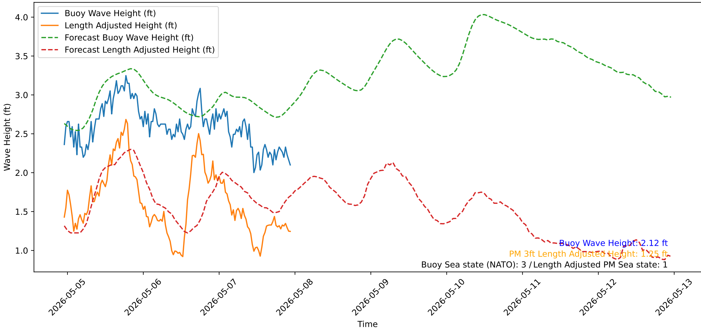
Wave Heights over Time for Oceanside Harbor at 2026-05-07 23:00:31
