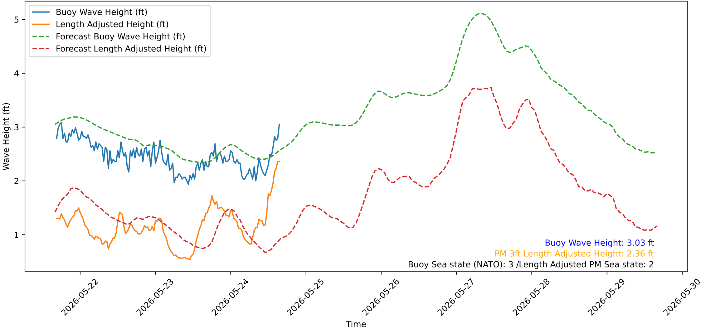
Wave Heights over Time for Red Beach at 2026-05-24 16:10:52
