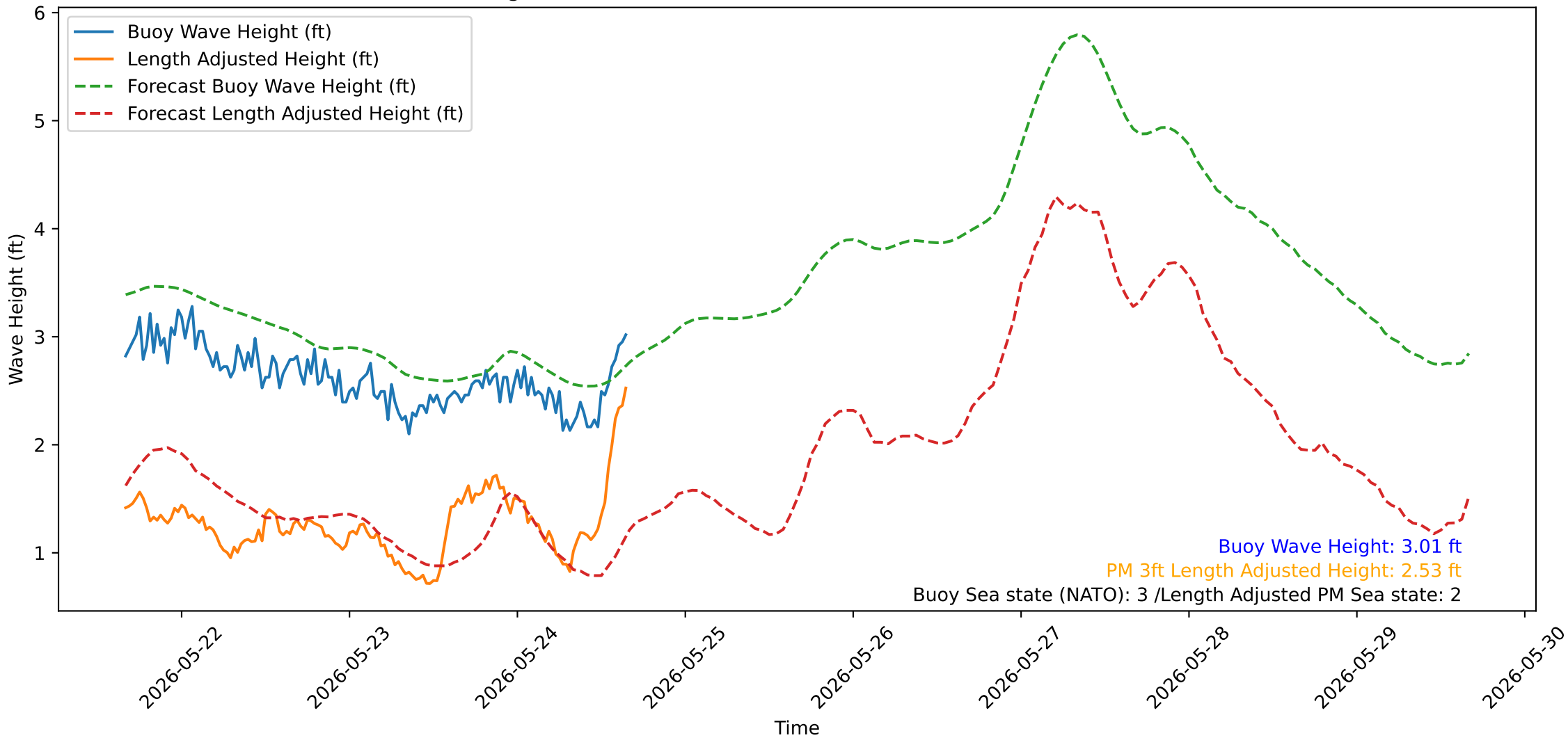
Wave Heights over Time for Oceanside Harbor at 2026-05-24 16:10:32
