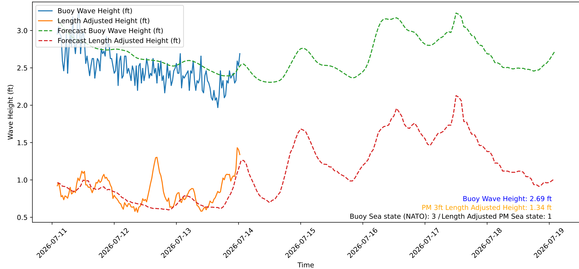
Wave Heights over Time for Red Beach at 2026-07-14 01:30:46
