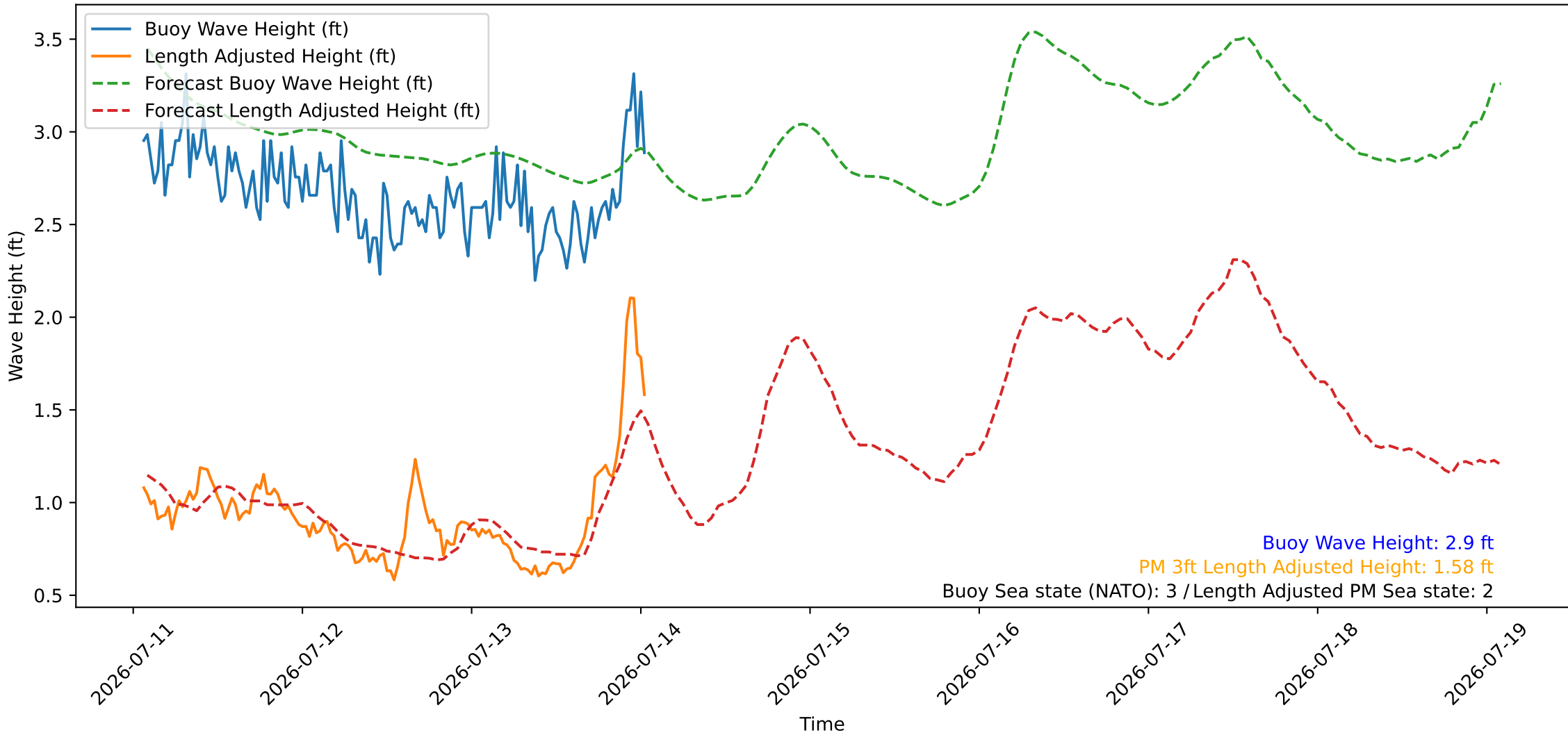
Wave Heights over Time for Green Beach at 2026-07-14 01:31:09
