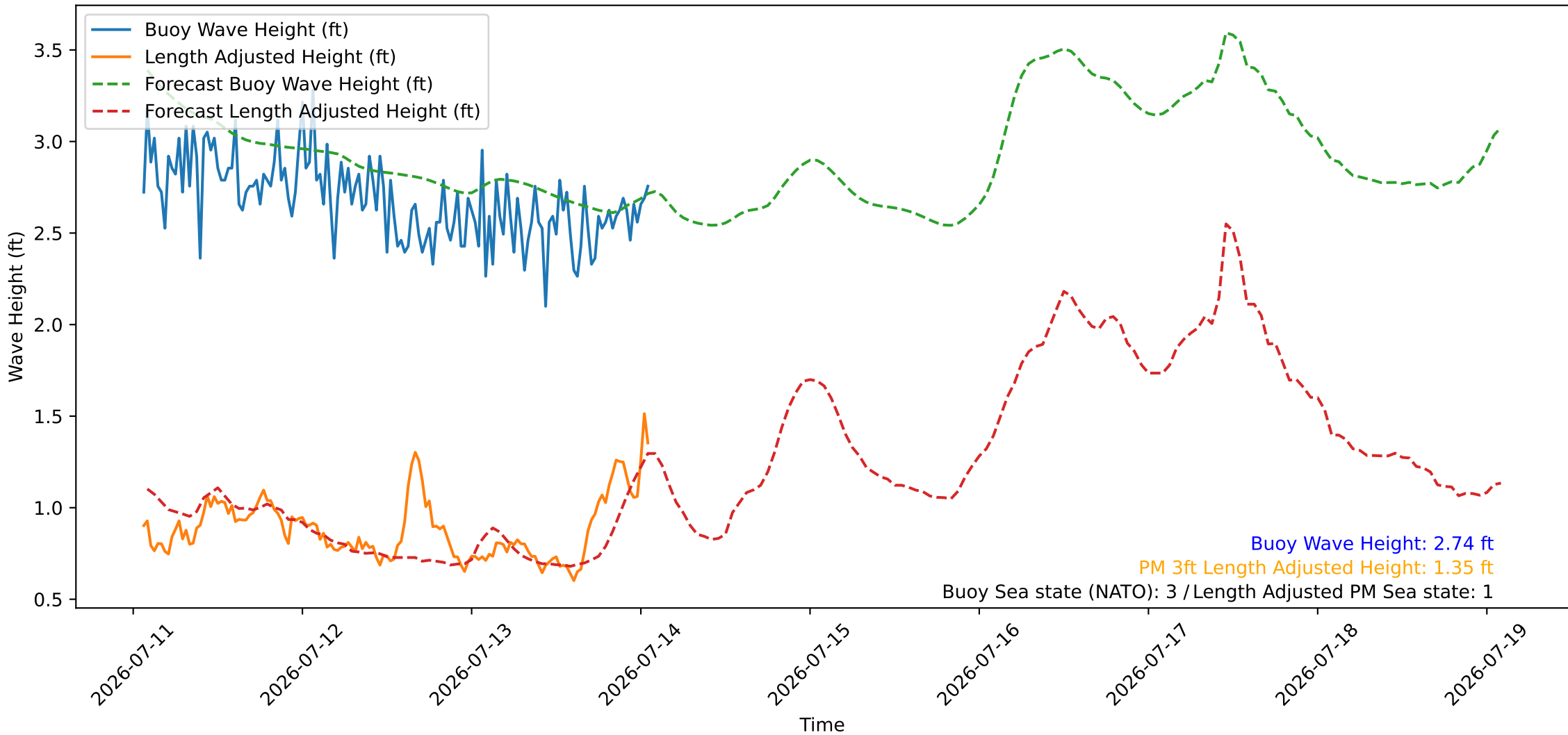
Wave Heights over Time for Oceanside Harbor at 2026-07-14 01:30:27
