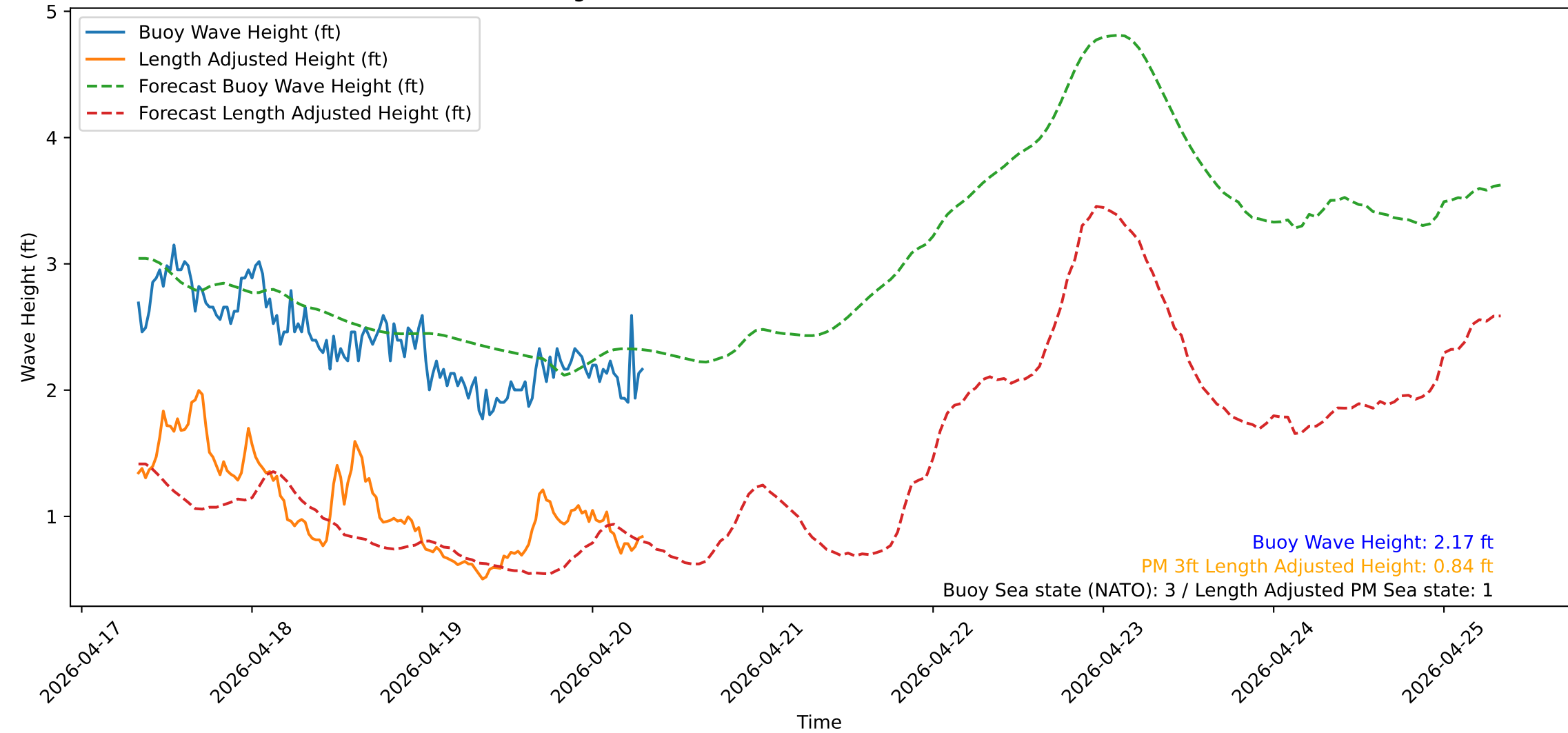
Wave Heights over Time for Red Beach at 2026-04-20 07:50:52
