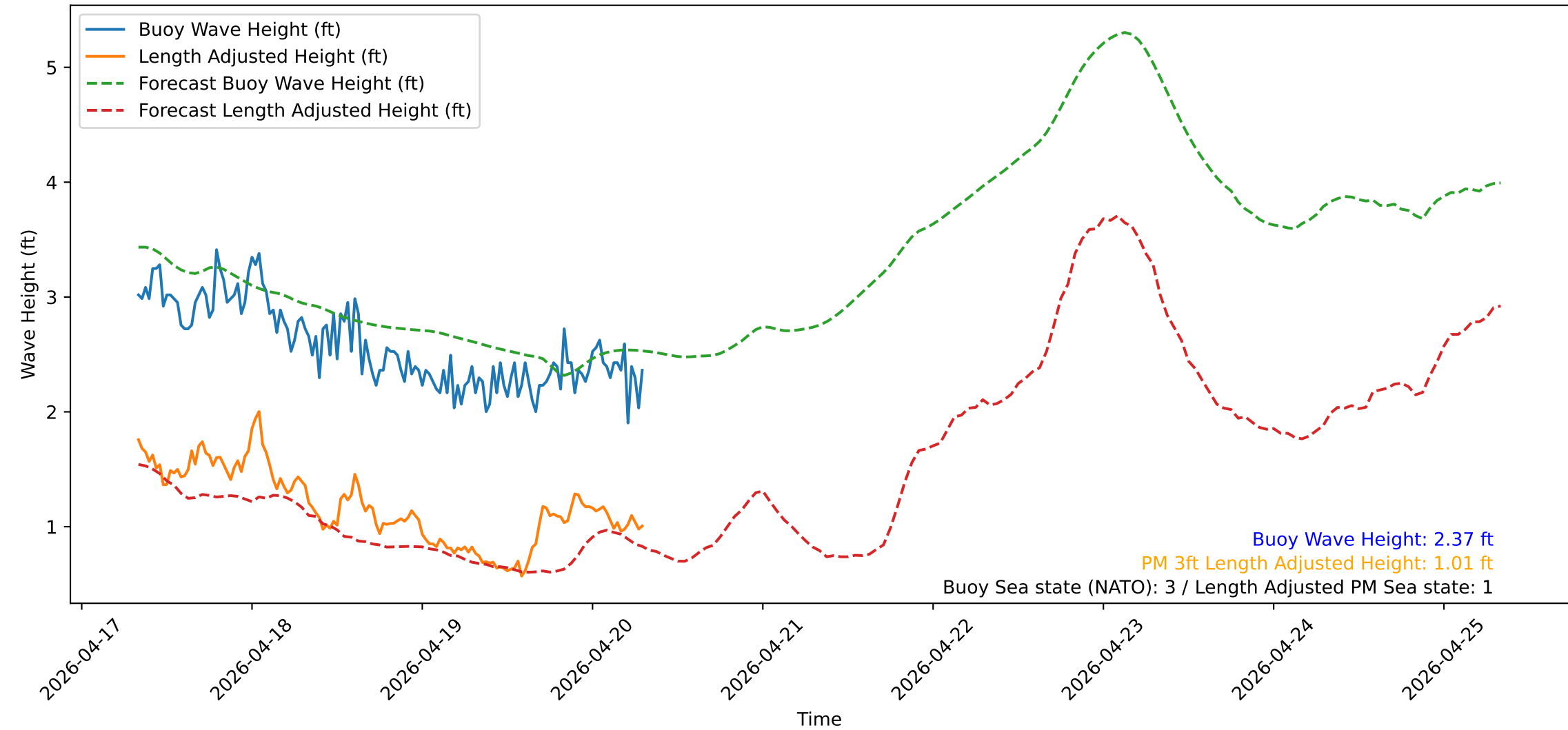
Wave Heights over Time for Oceanside Harbor at 2026-04-20 07:50:31
