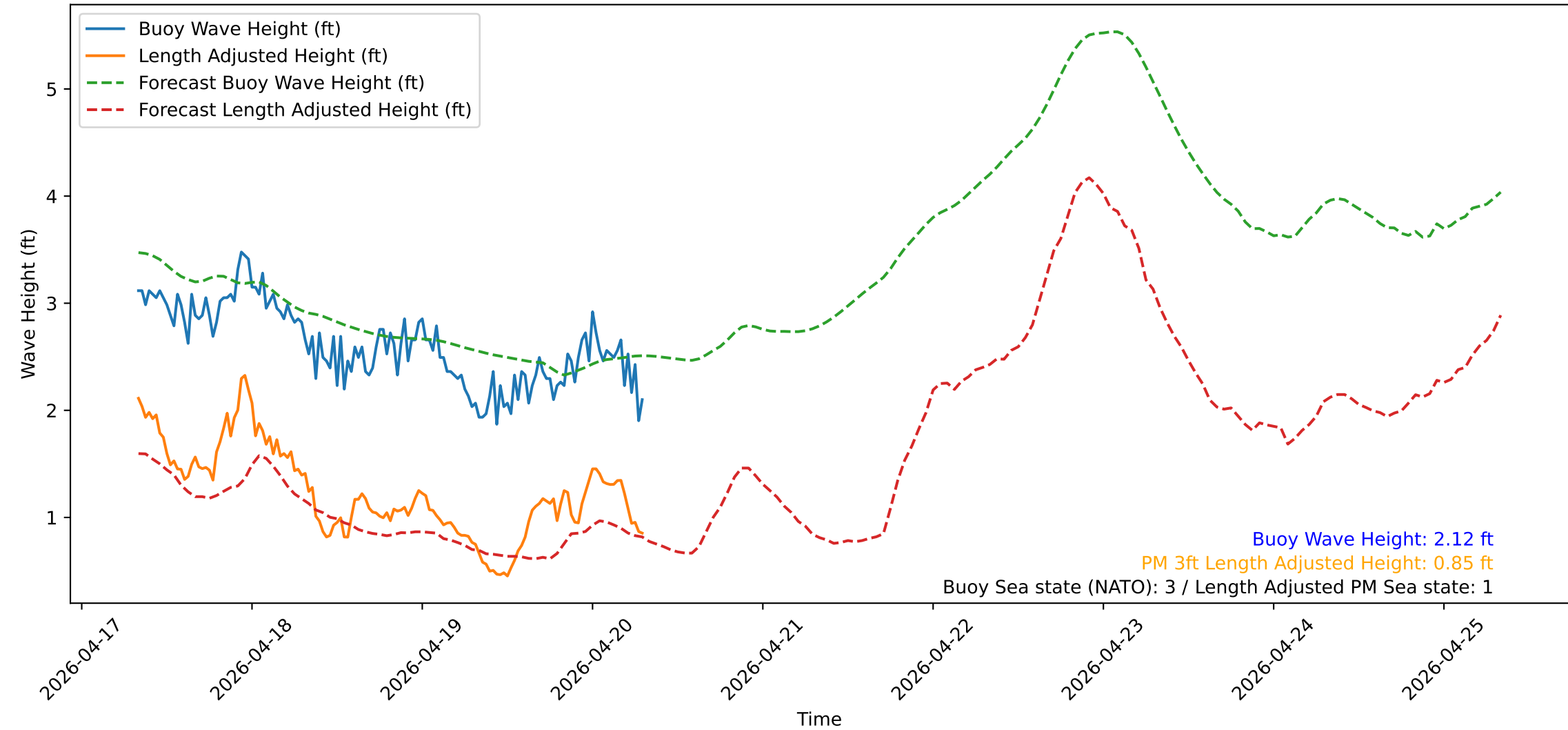
Wave Heights over Time for Green Beach at 2026-04-20 07:51:14
