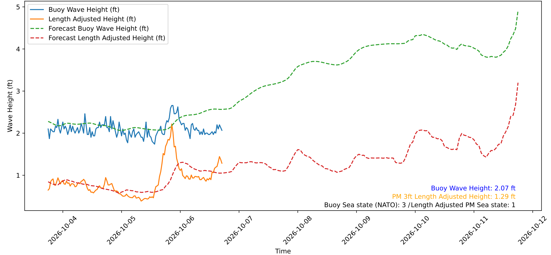
Wave Heights over Time for Red Beach at 2026-10-06 17:50:51
