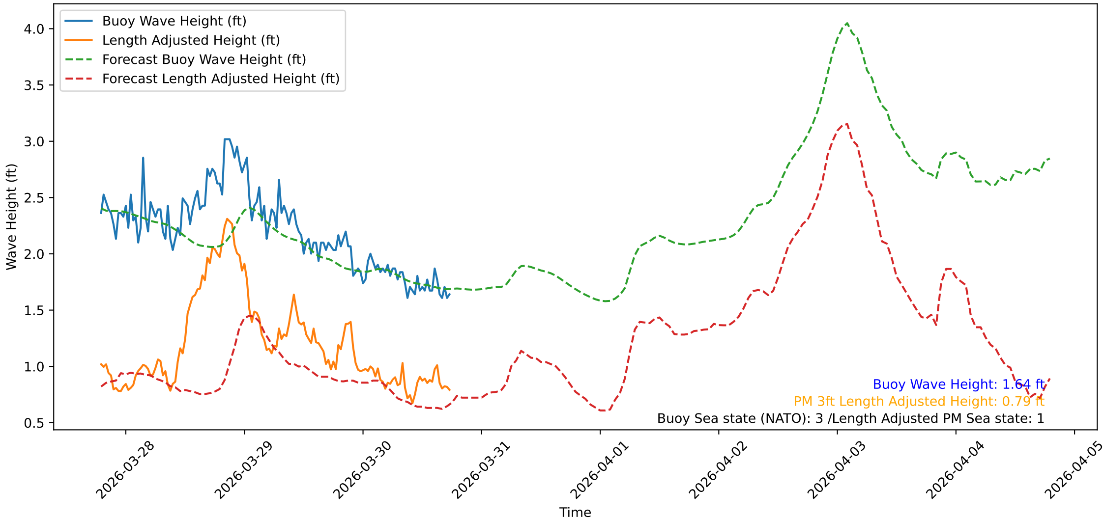
Wave Heights over Time for Red Beach at 2026-03-30 18:30:48
