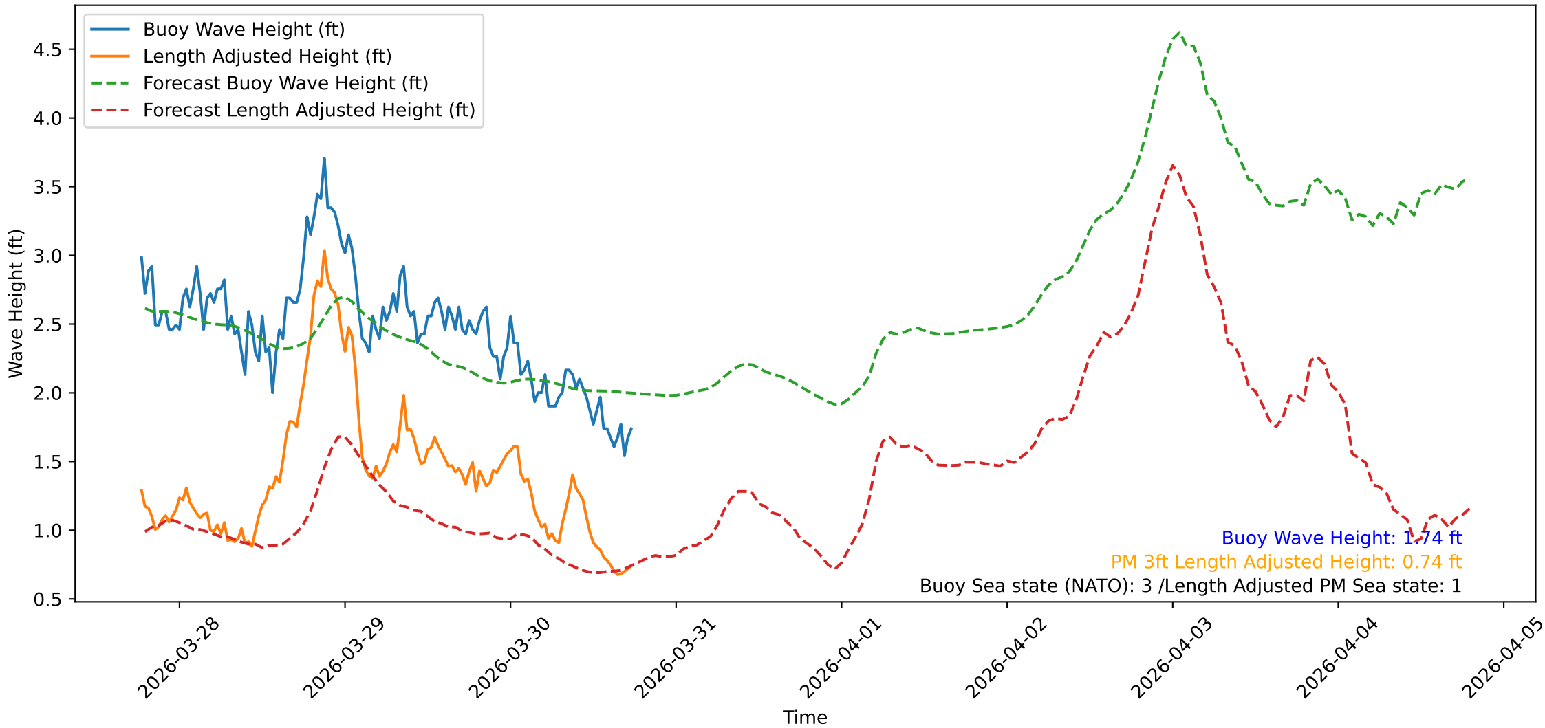
Wave Heights over Time for Green Beach at 2026-03-30 18:31:10
