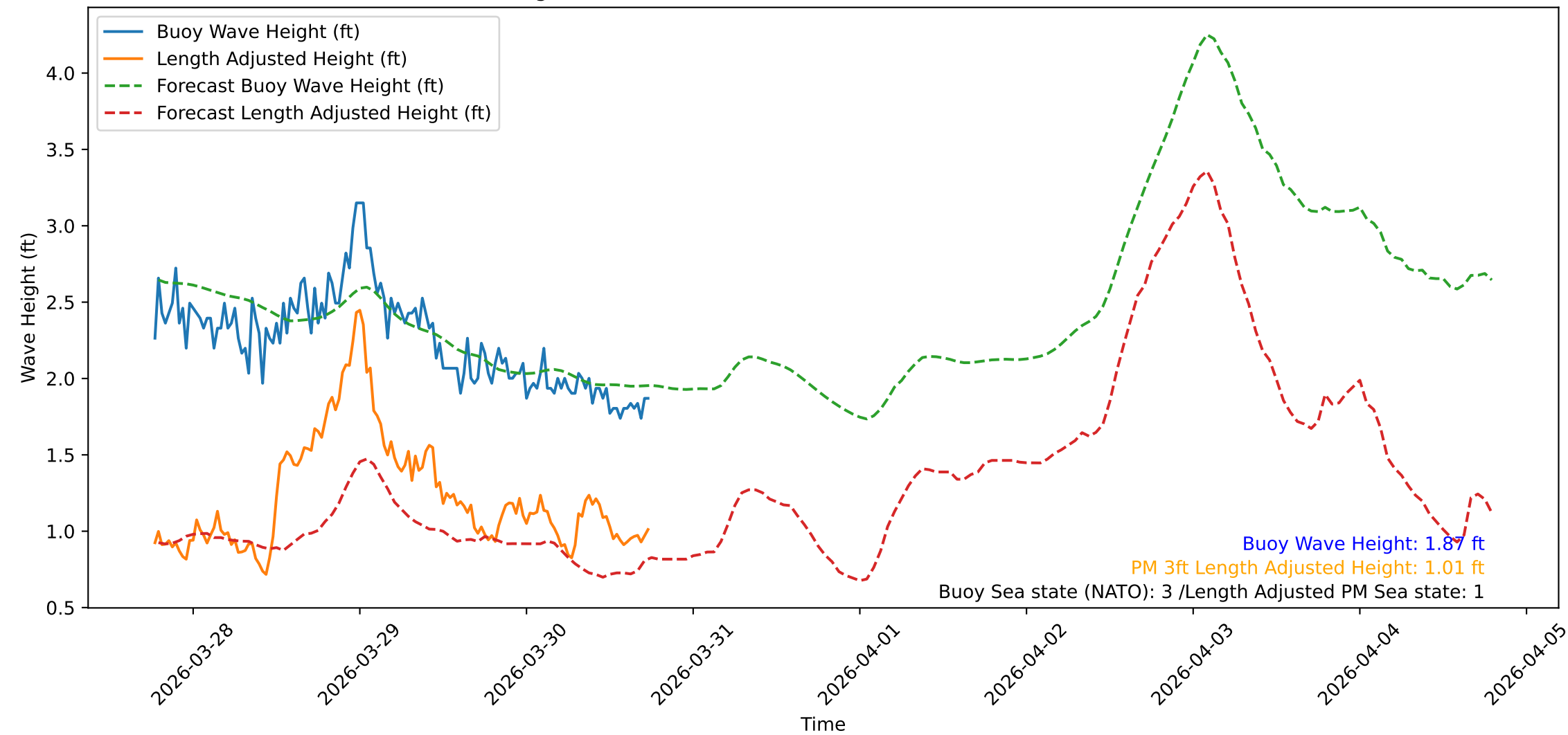
Wave Heights over Time for Oceanside Harbor at 2026-03-30 18:30:32
