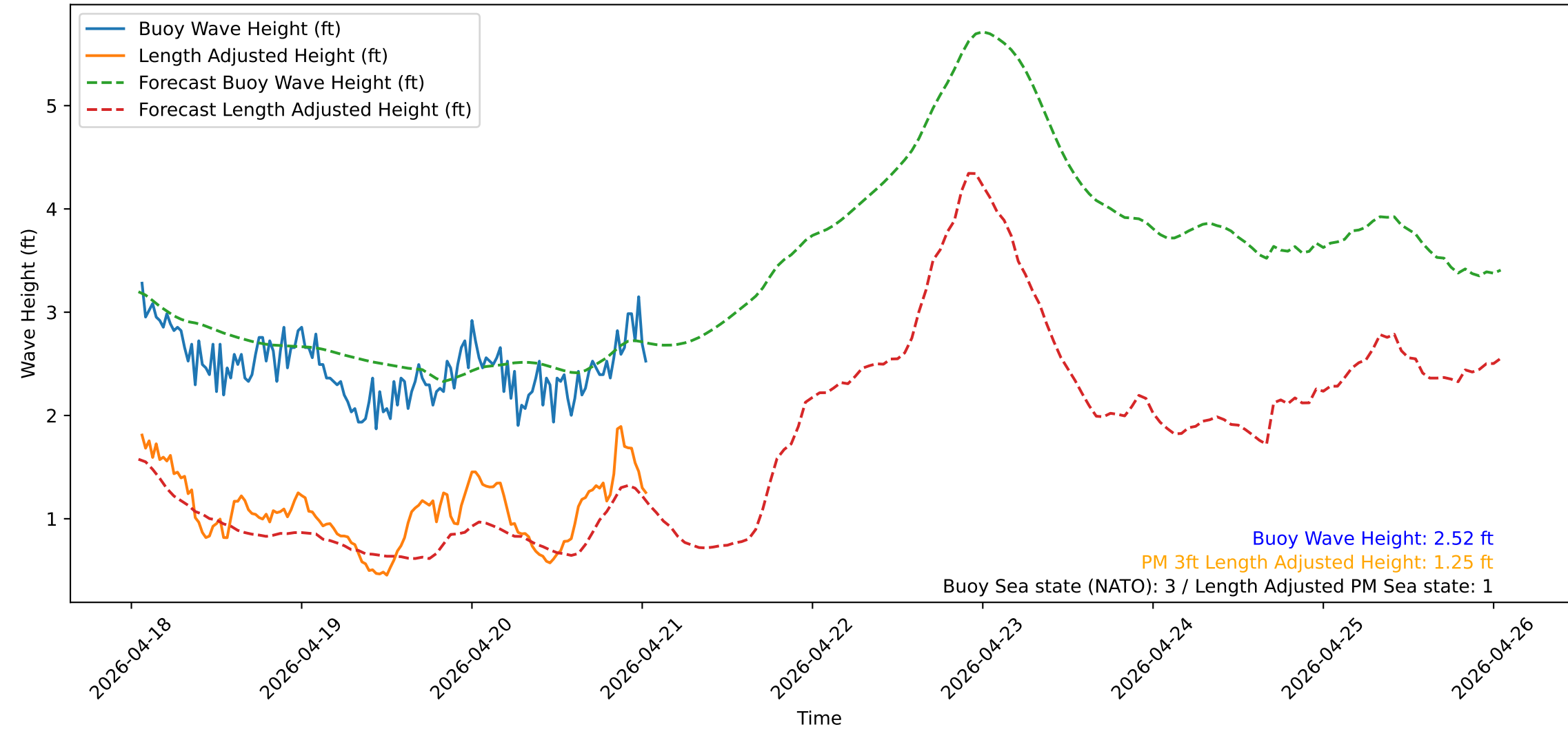
Wave Heights over Time for Green Beach at 2026-04-21 01:21:13
