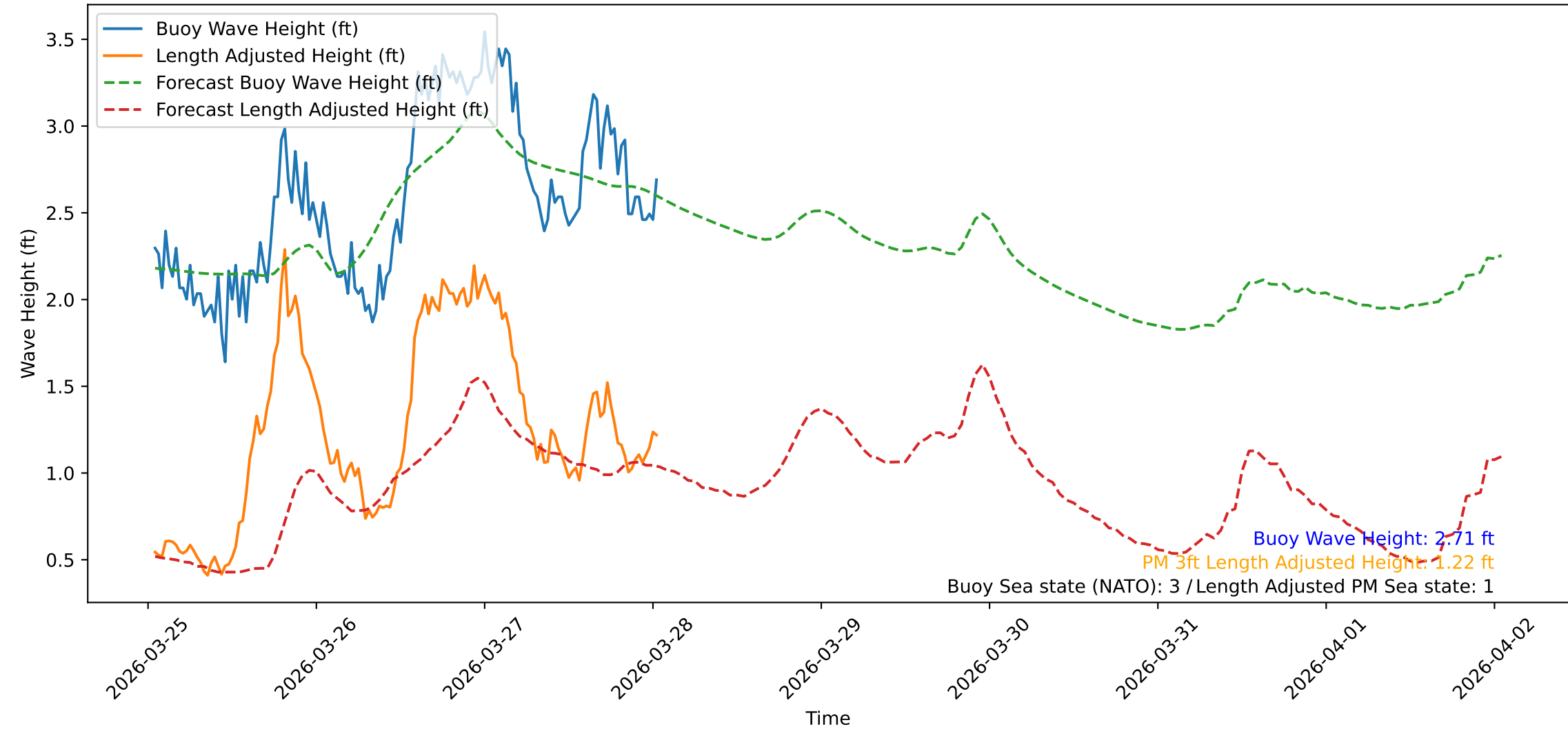
Wave Heights over Time for Green Beach at 2026-03-28 01:11:09
