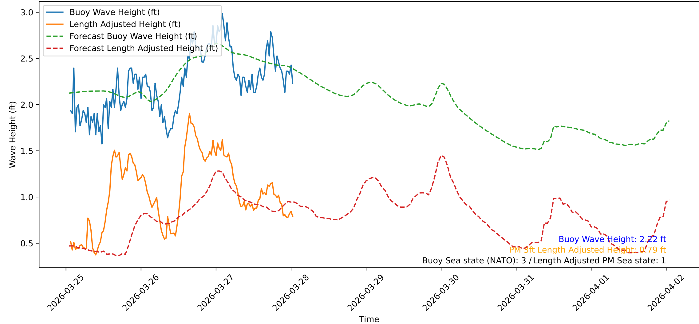
Wave Heights over Time for Red Beach at 2026-03-28 01:10:47
