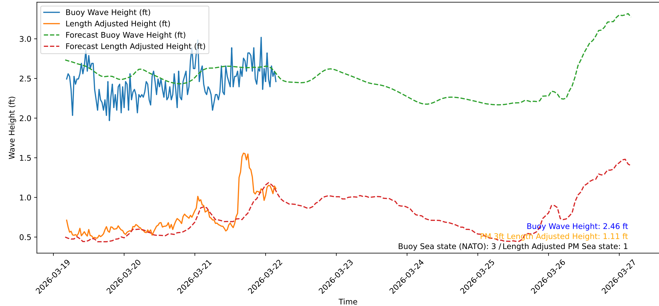
Wave Heights over Time for Oceanside Harbor at 2026-03-22 04:20:31
