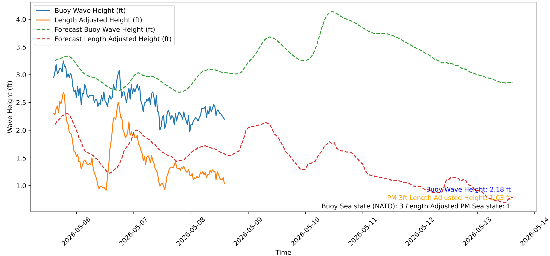
Wave Heights over Time for Oceanside Harbor at 2026-05-08 14:40:31
