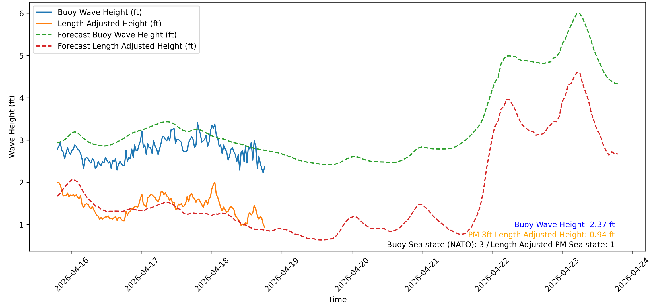
Wave Heights over Time for Oceanside Harbor at 2026-04-18 18:50:31
