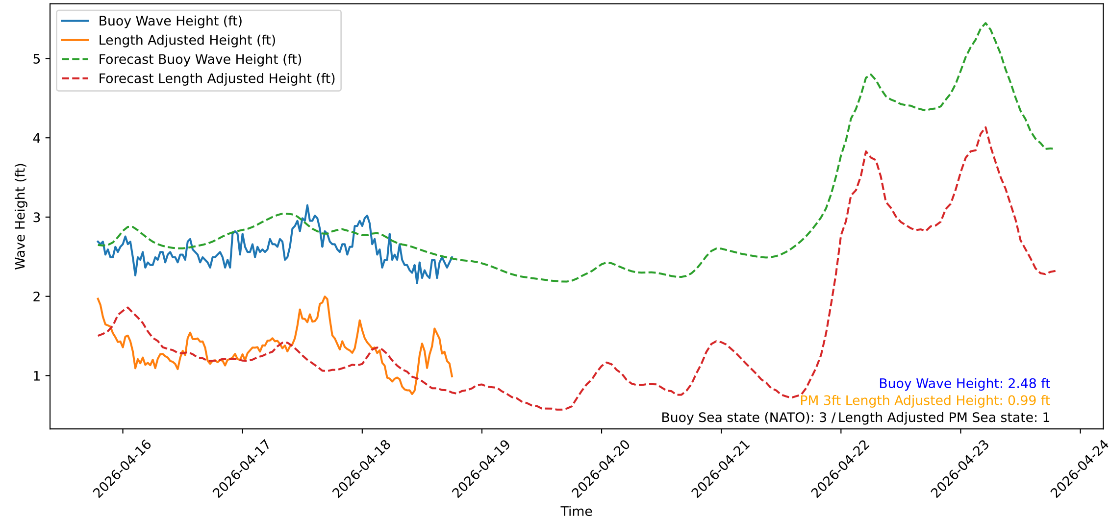
Wave Heights over Time for Red Beach at 2026-04-18 18:50:51
