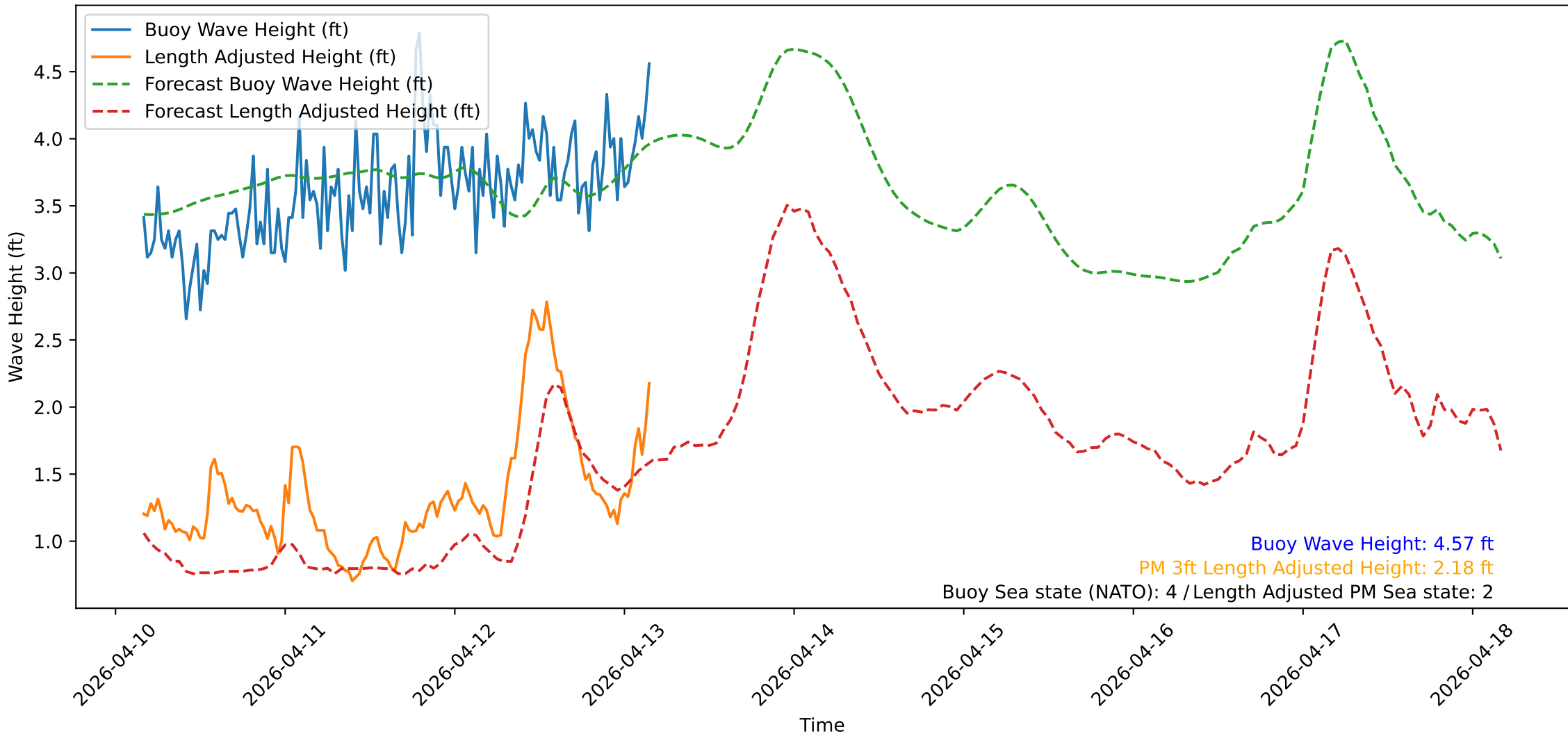
Wave Heights over Time for Oceanside Harbor at 2026-04-13 04:10:31
