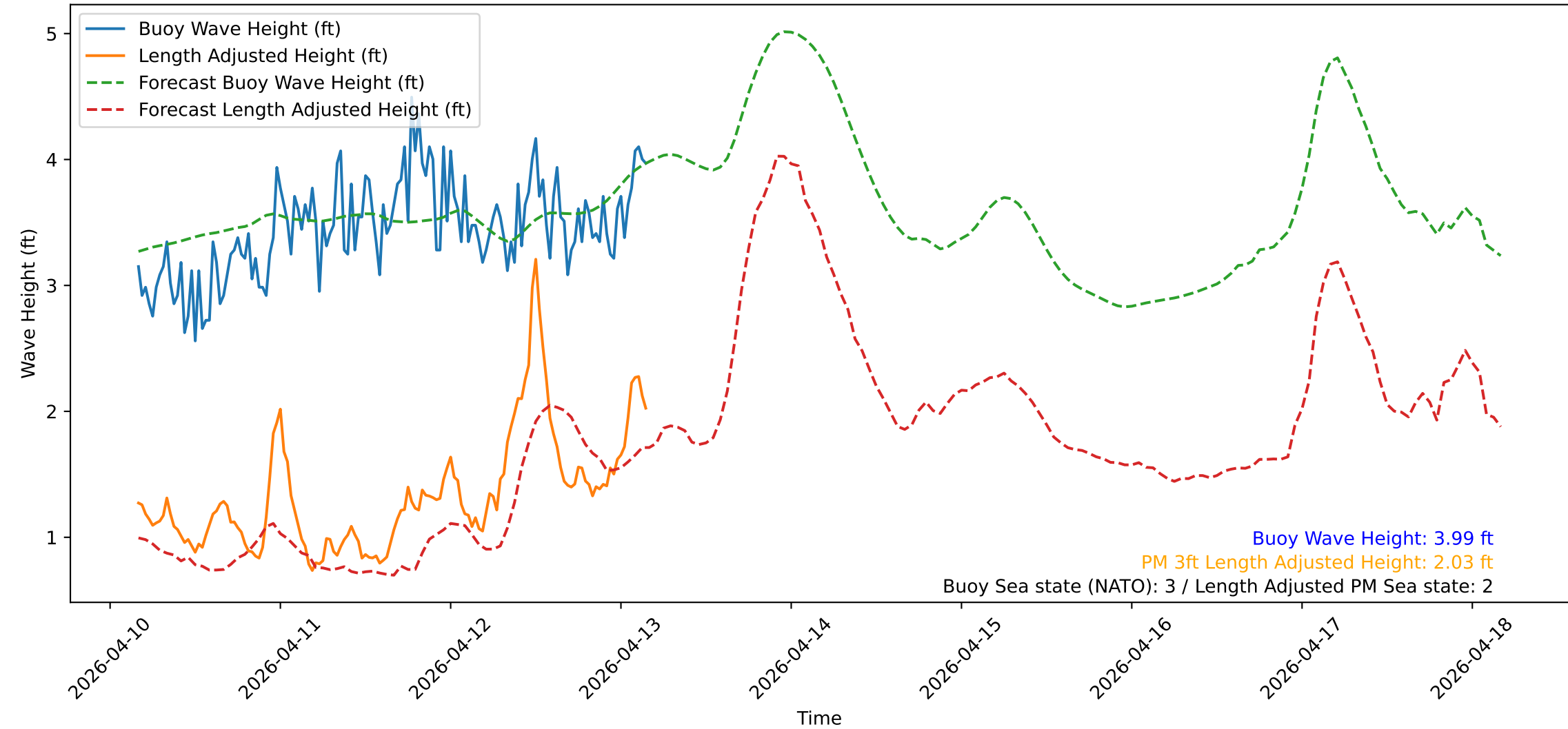
Wave Heights over Time for Green Beach at 2026-04-13 04:11:12
