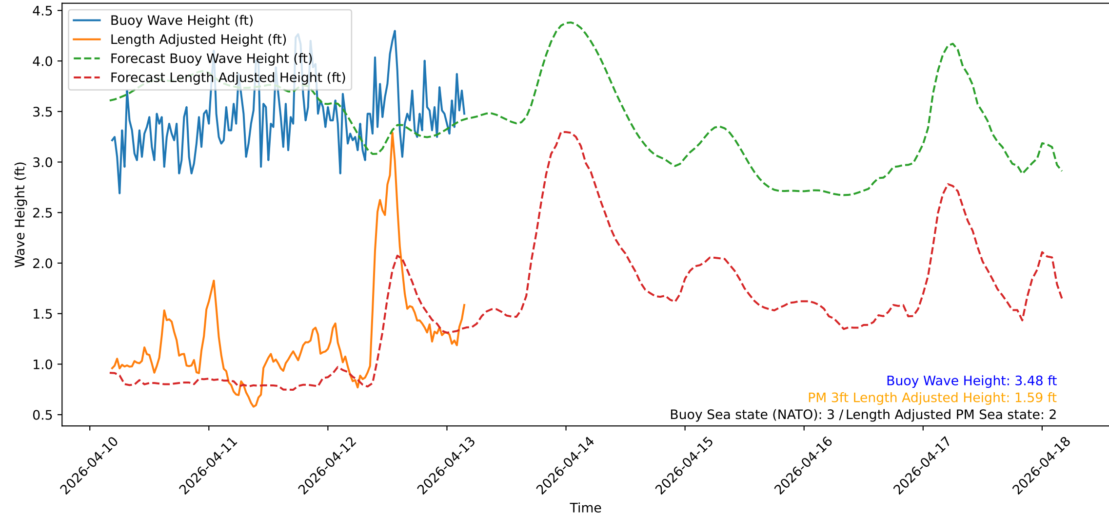
Wave Heights over Time for Red Beach at 2026-04-13 04:10:50
