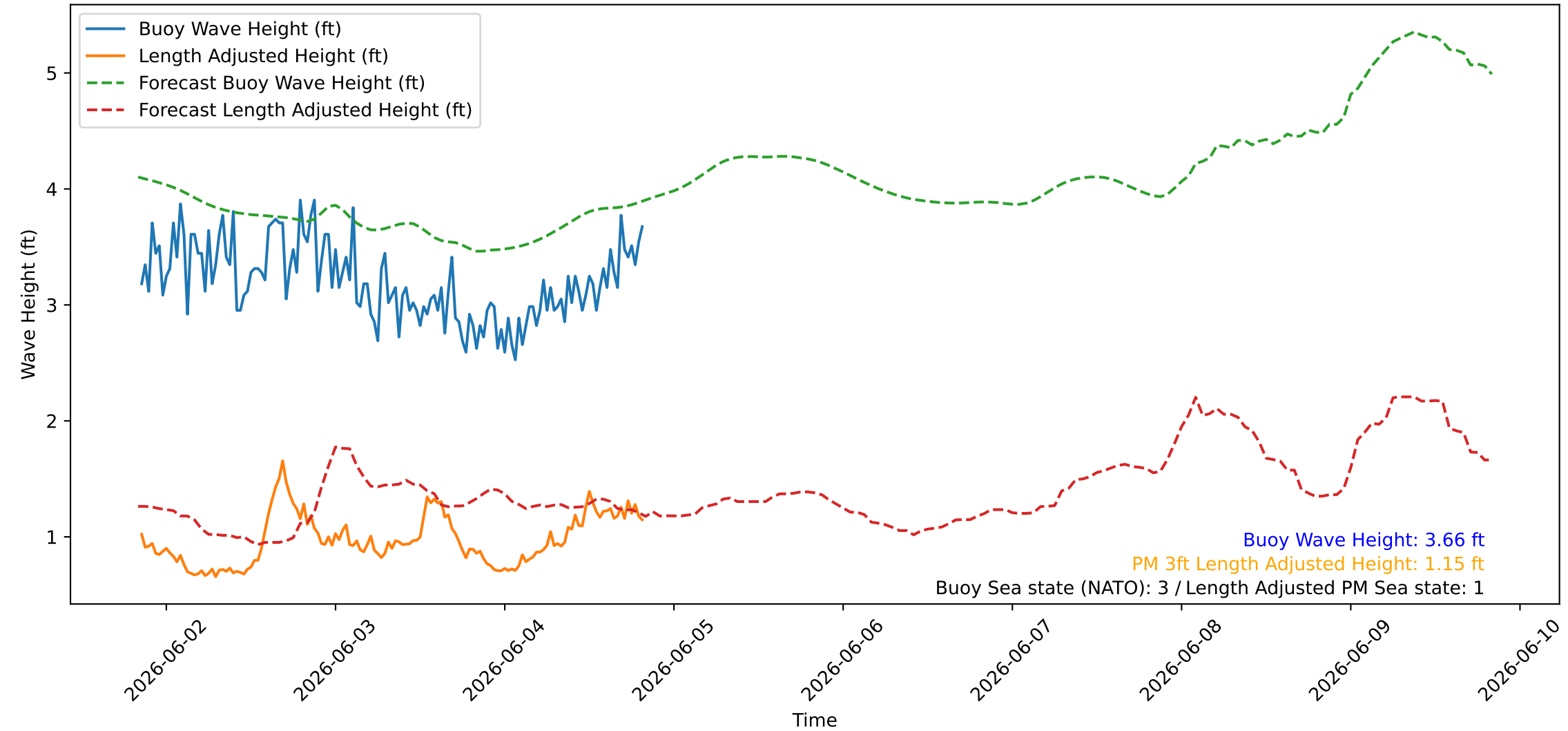
Wave Heights over Time for Red Beach at 2026-06-04 20:20:46
