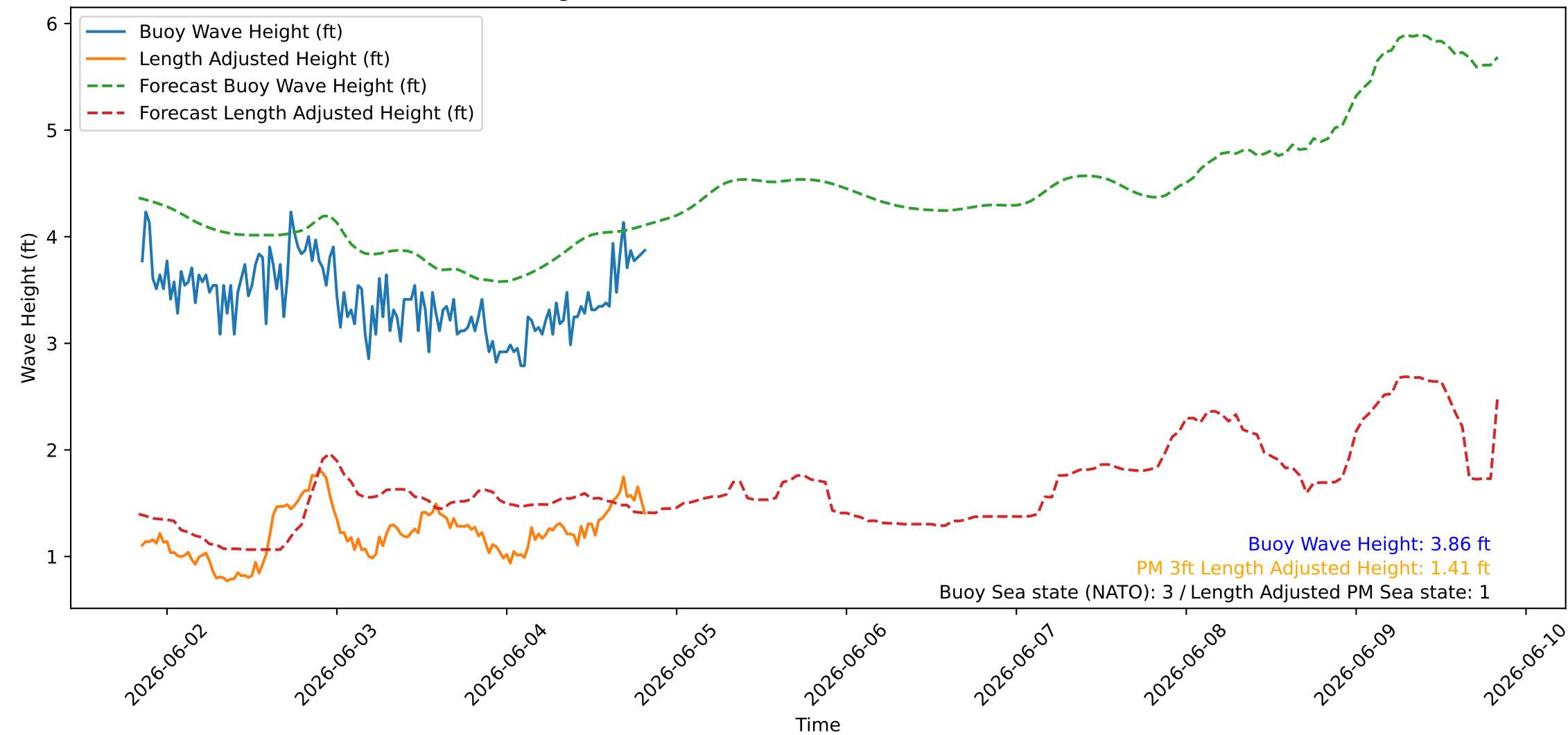
Wave Heights over Time for Green Beach at 2026-06-04 20:21:08
