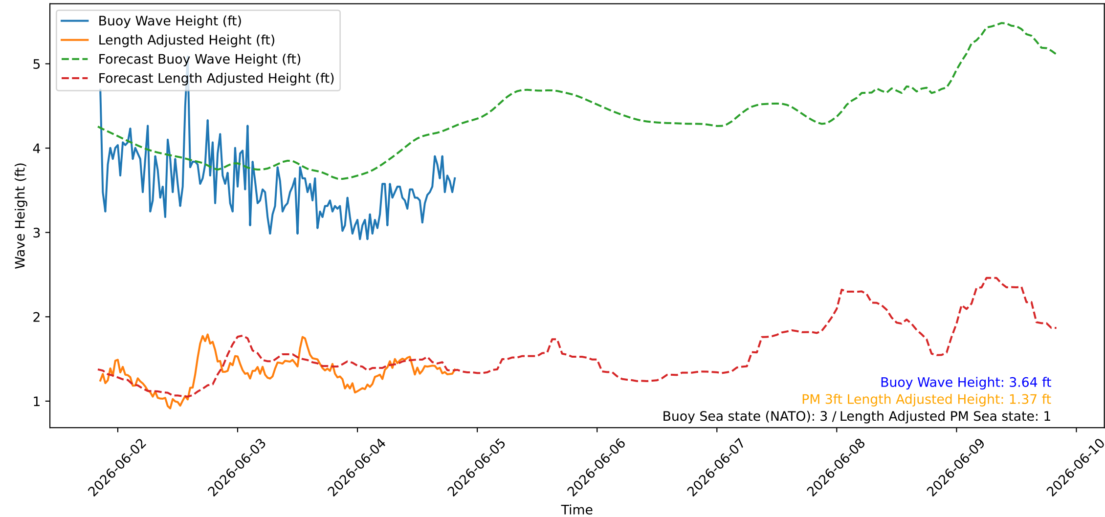
Wave Heights over Time for Oceanside Harbor at 2026-06-04 20:20:25
