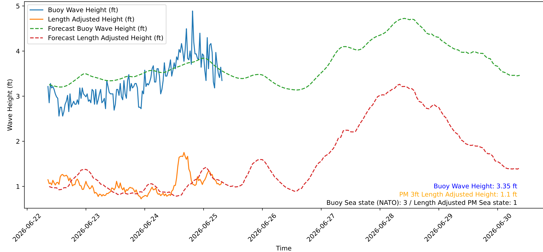
Wave Heights over Time for Oceanside Harbor at 2026-06-25 08:30:26
