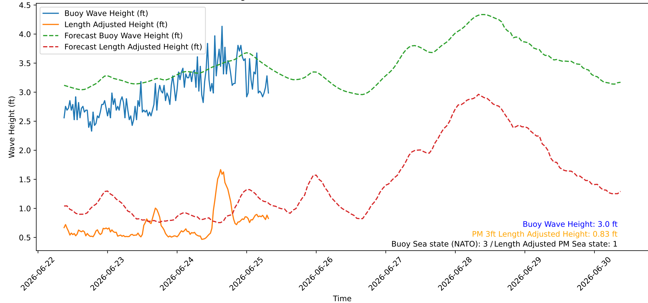
Wave Heights over Time for Red Beach at 2026-06-25 08:30:45
