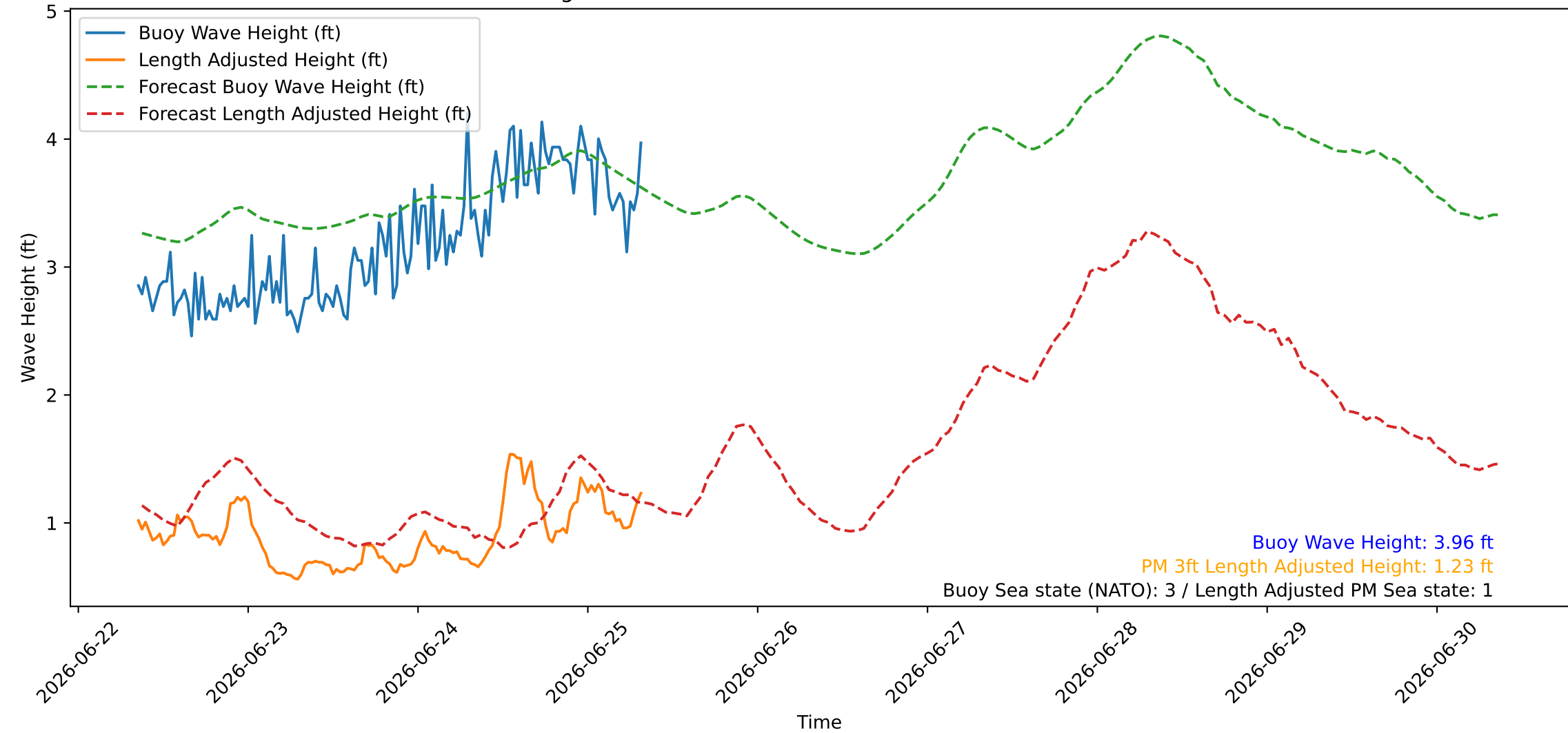
Wave Heights over Time for Green Beach at 2026-06-25 08:31:07
