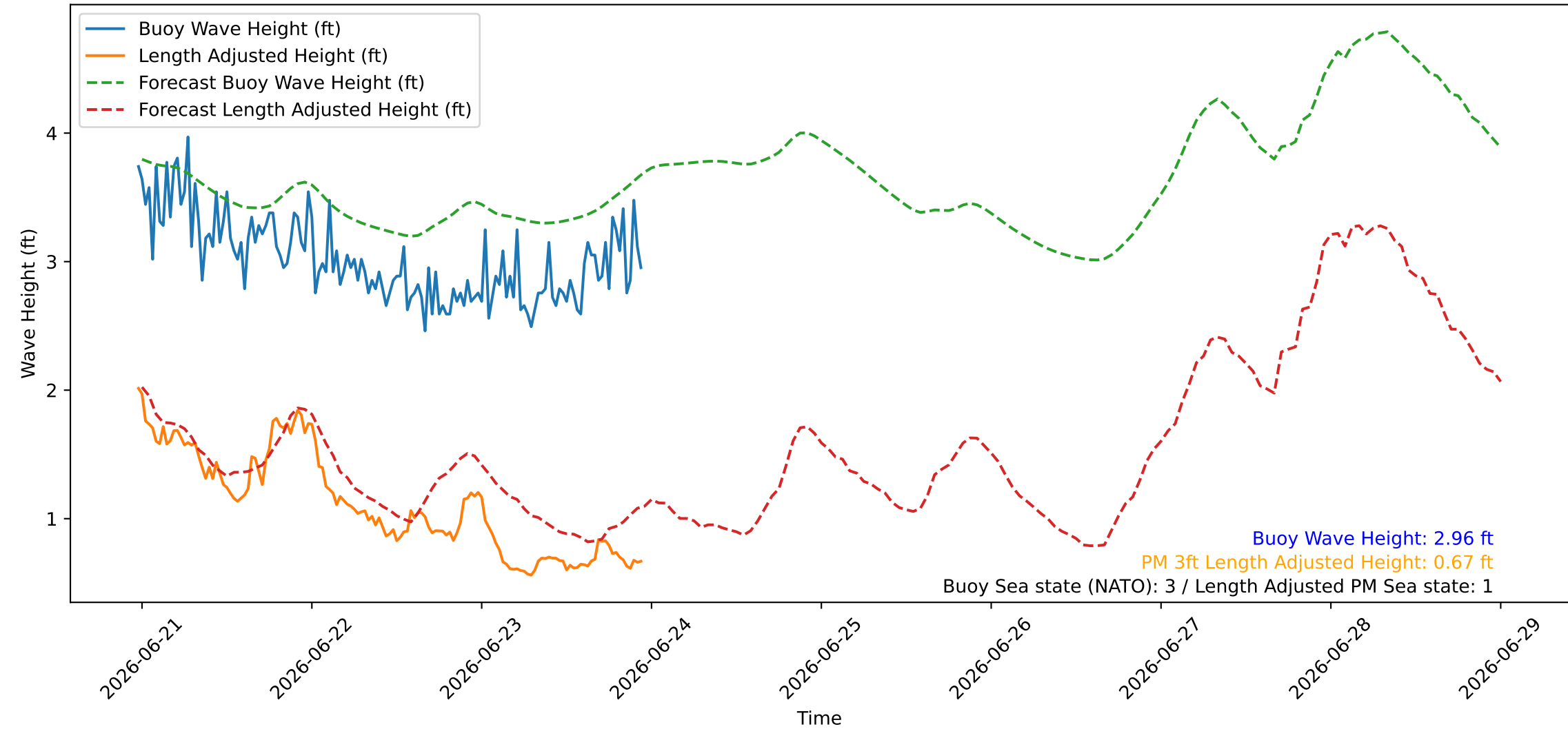
Wave Heights over Time for Green Beach at 2026-06-23 23:31:08
