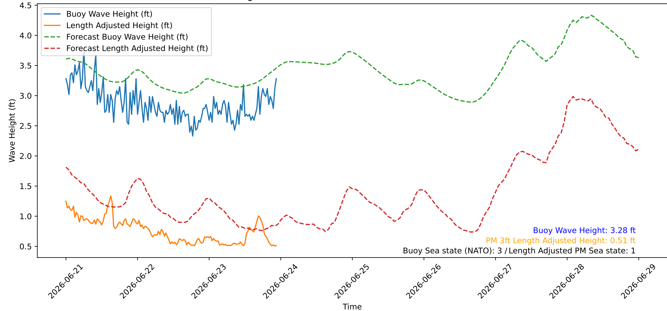
Wave Heights over Time for Red Beach at 2026-06-23 23:30:45
