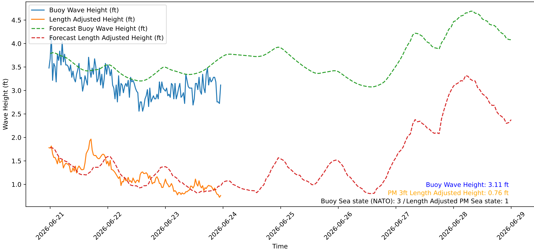
Wave Heights over Time for Oceanside Harbor at 2026-06-23 23:30:26
