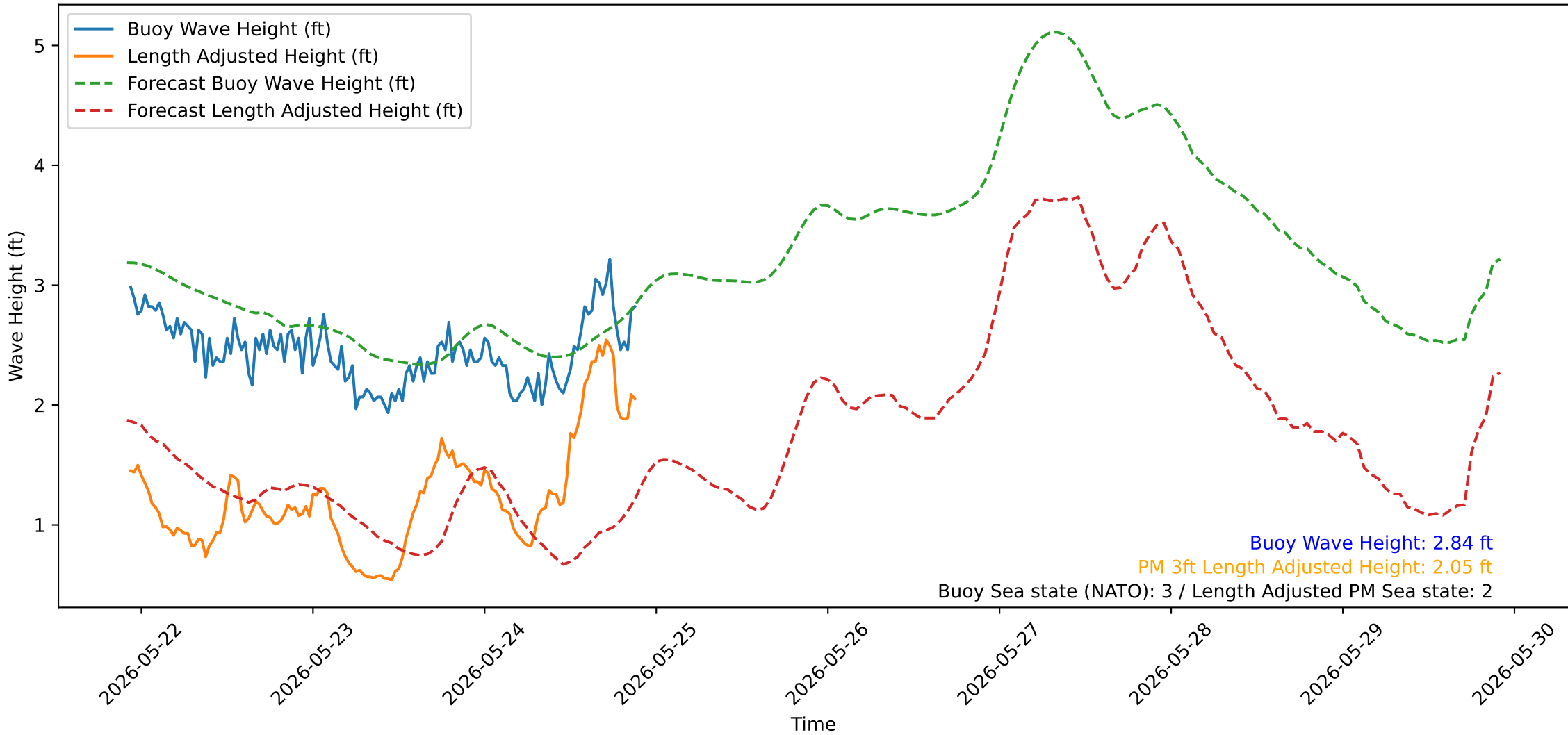
Wave Heights over Time for Red Beach at 2026-05-24 22:00:51
