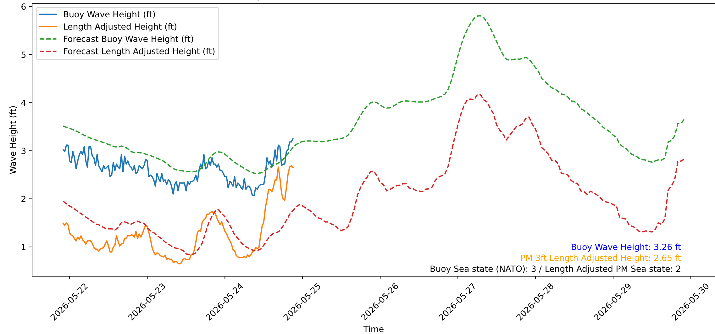
Wave Heights over Time for Green Beach at 2026-05-24 22:01:14
