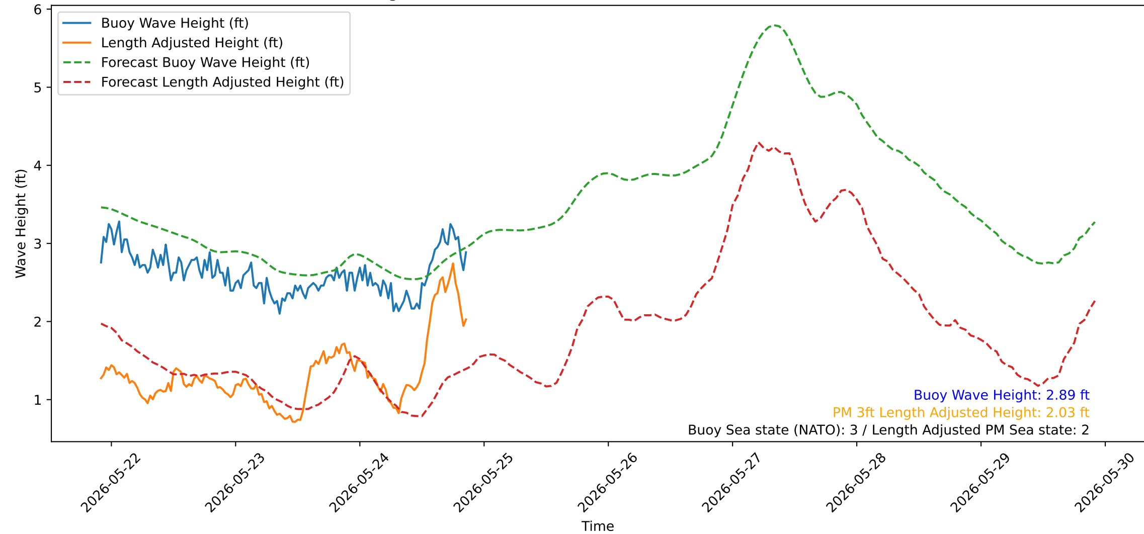
Wave Heights over Time for Oceanside Harbor at 2026-05-24 22:00:32
