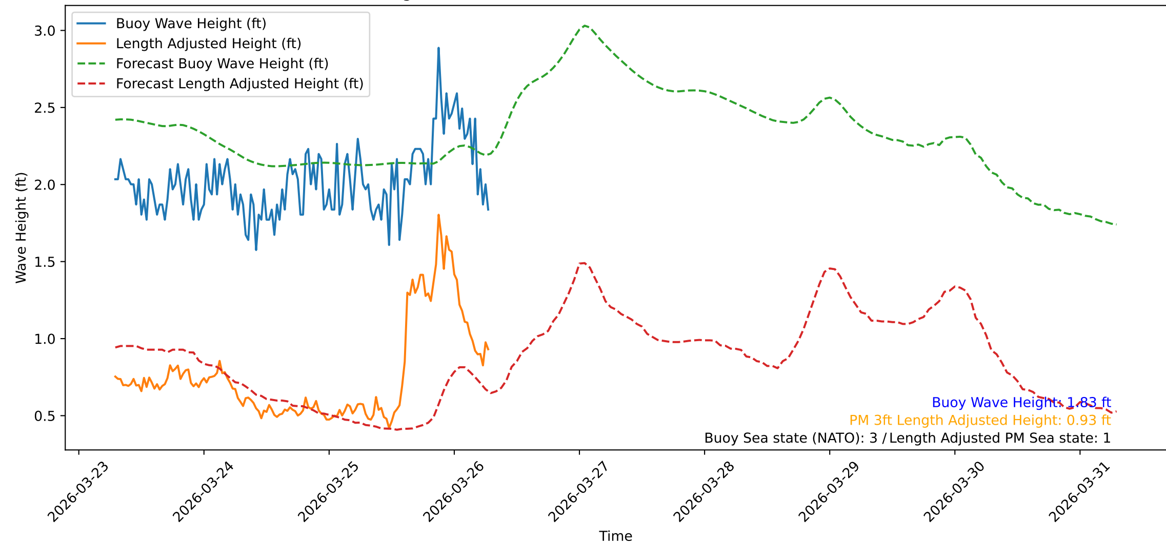
Wave Heights over Time for Oceanside Harbor at 2026-03-26 07:00:31
