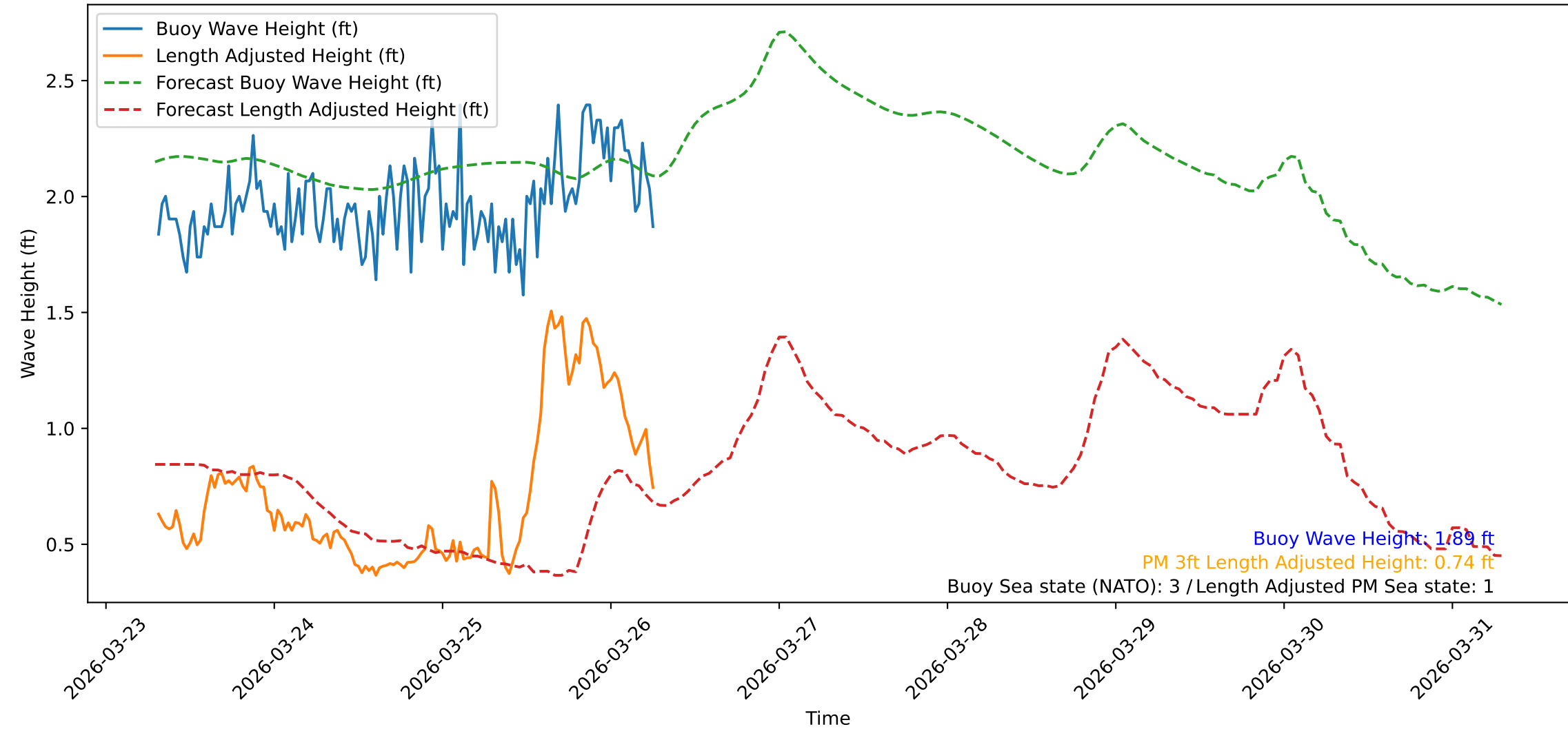
Wave Heights over Time for Red Beach at 2026-03-26 07:00:47
