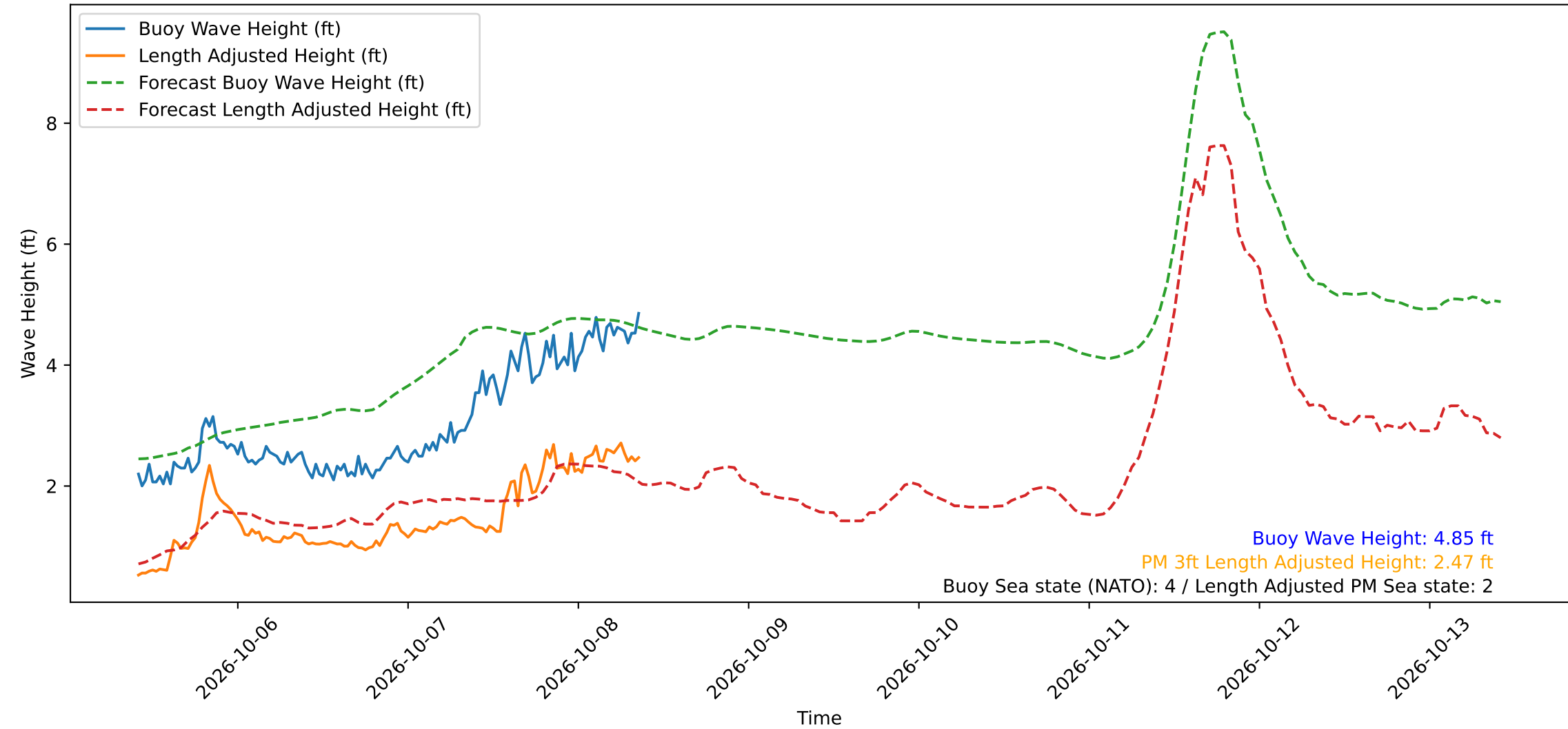
Wave Heights over Time for Green Beach at 2026-10-08 09:31:13
