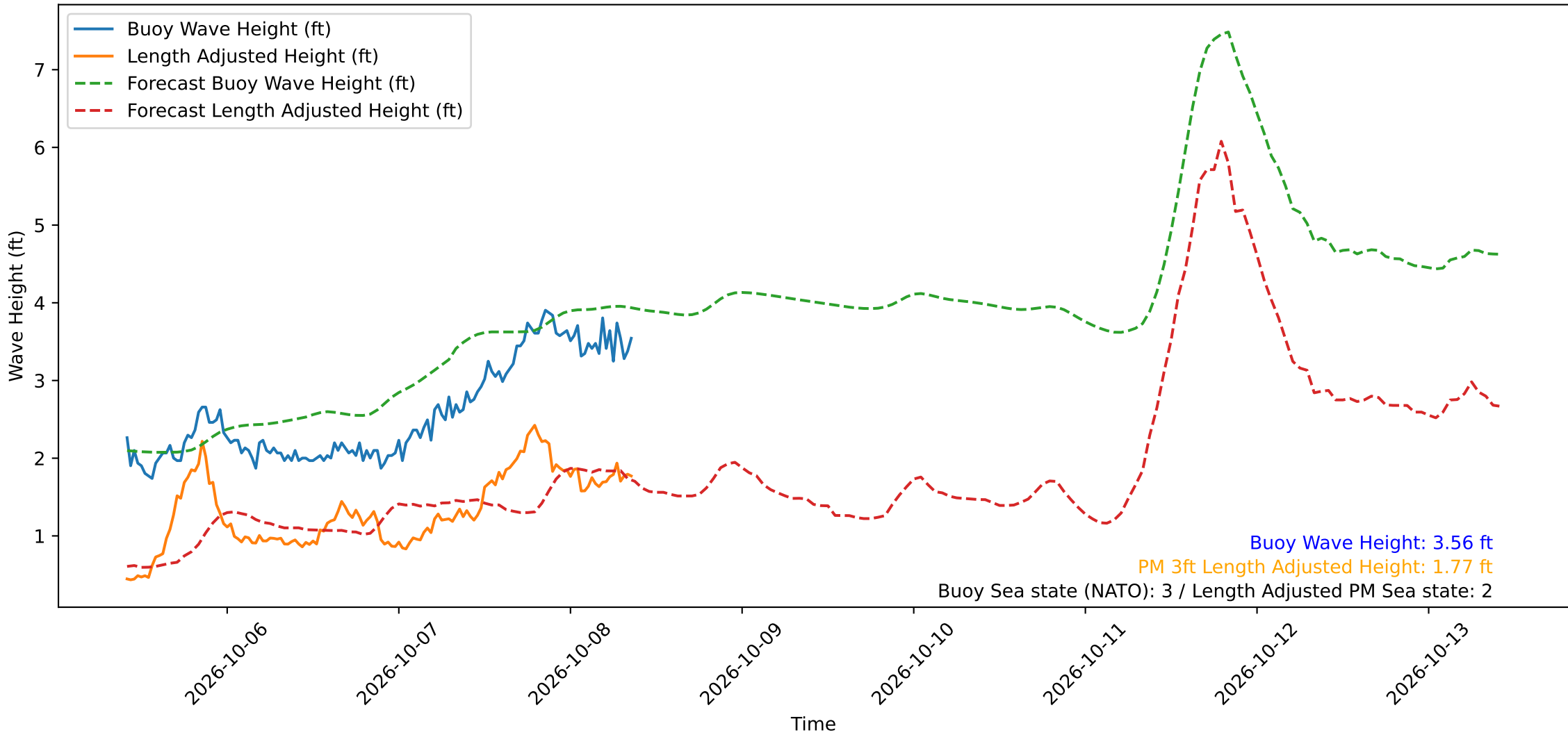
Wave Heights over Time for Red Beach at 2026-10-08 09:30:50
