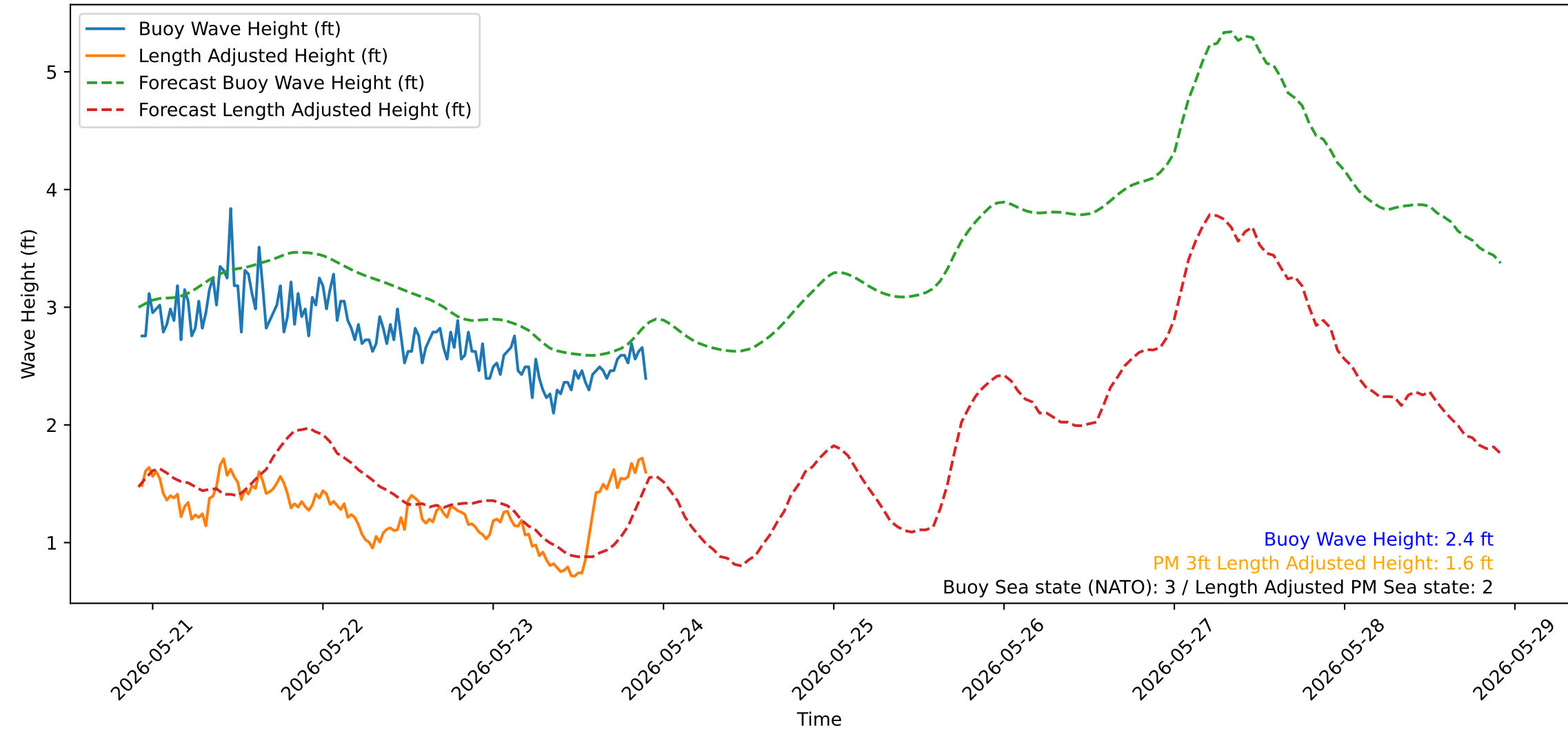
Wave Heights over Time for Oceanside Harbor at 2026-05-23 22:20:32
