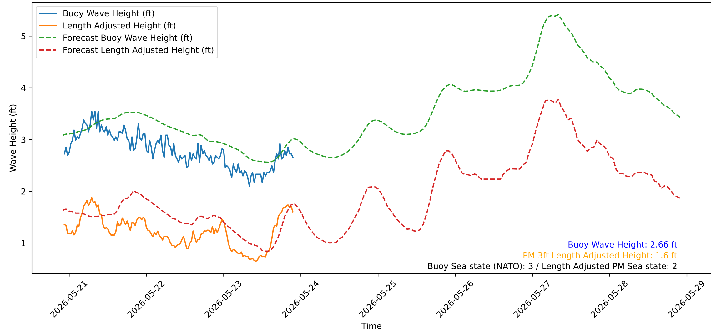
Wave Heights over Time for Green Beach at 2026-05-23 22:21:15
