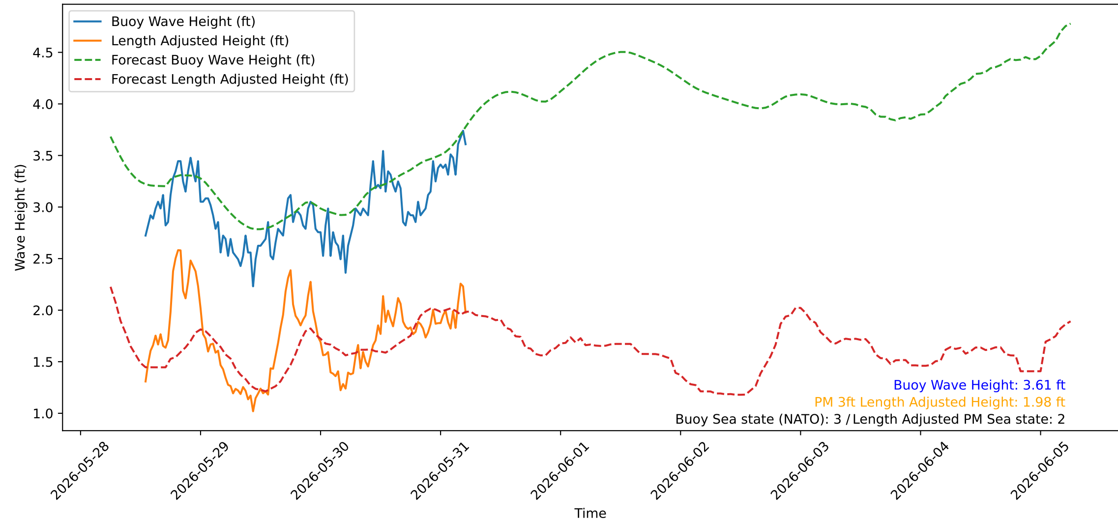
Wave Heights over Time for Oceanside Harbor at 2026-05-31 06:00:24
