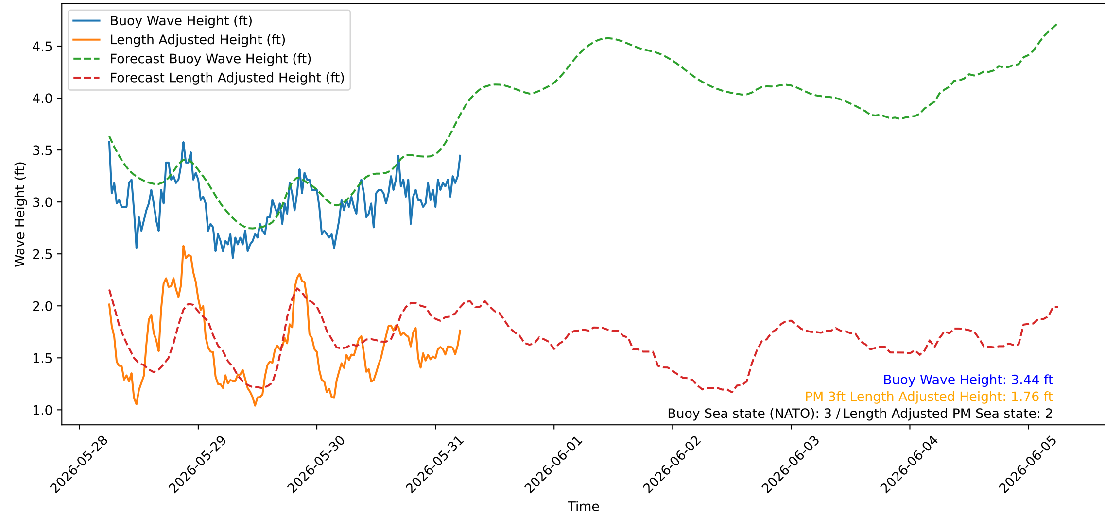
Wave Heights over Time for Green Beach at 2026-05-31 06:01:06
