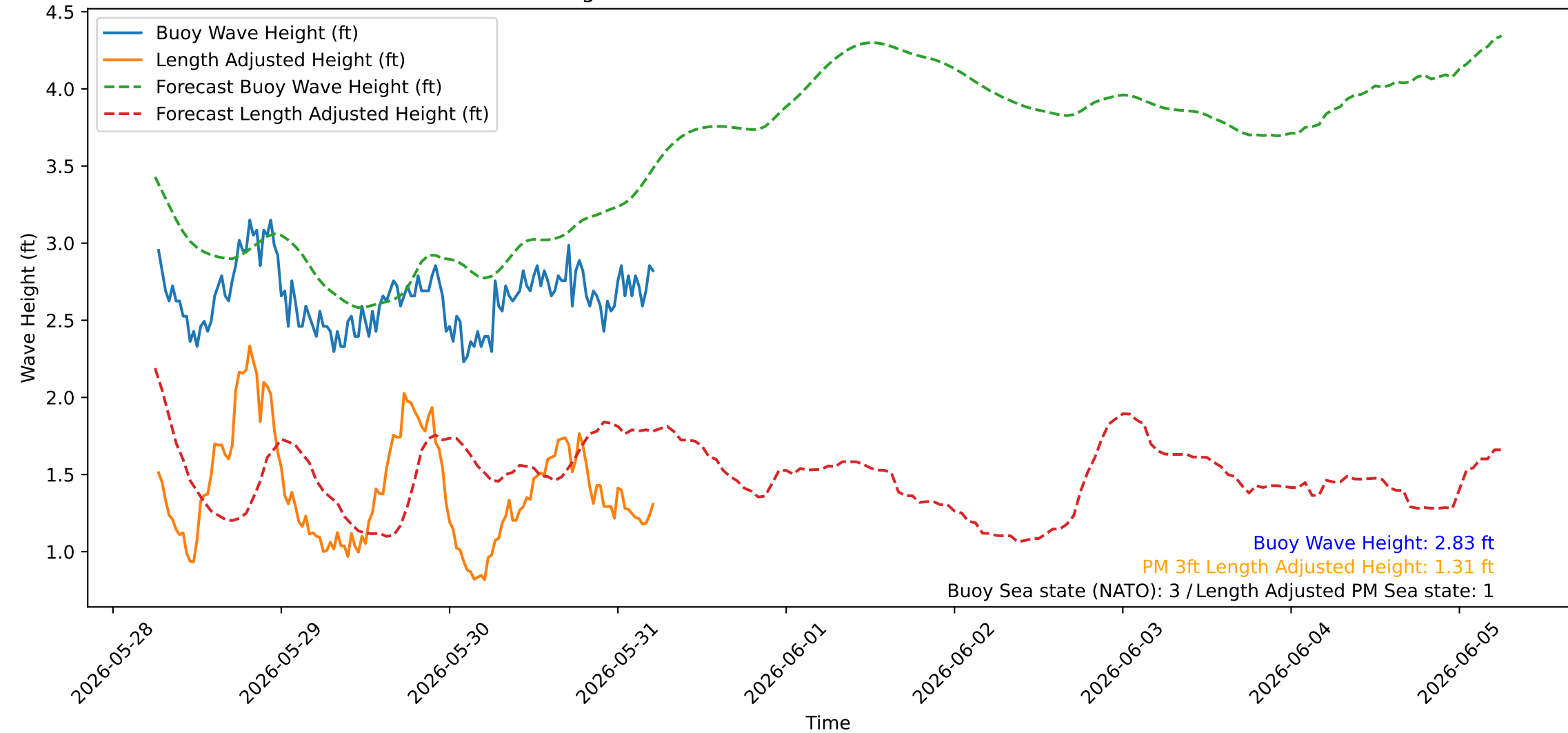
Wave Heights over Time for Red Beach at 2026-05-31 06:00:43
