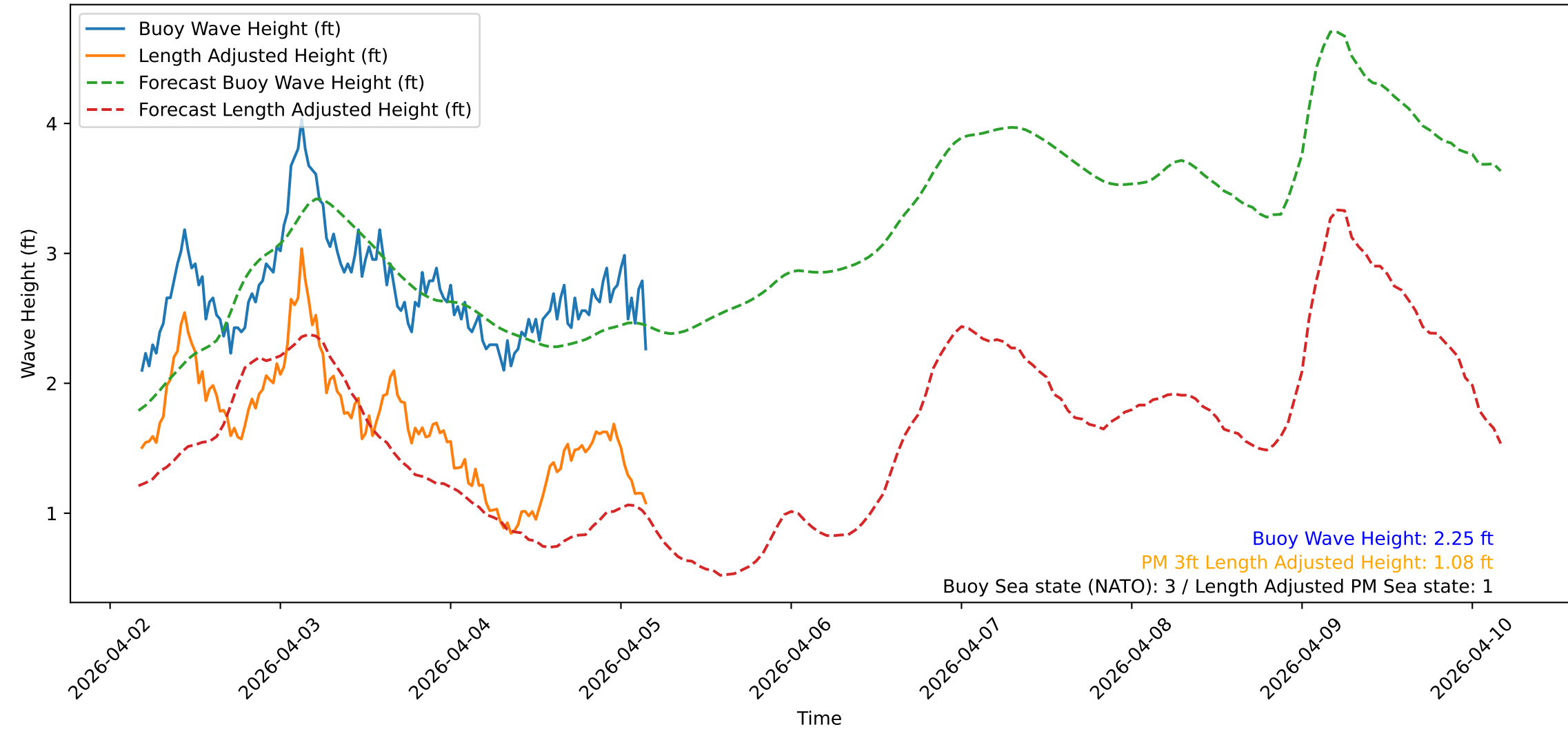
Wave Heights over Time for Oceanside Harbor at 2026-04-05 04:20:31
