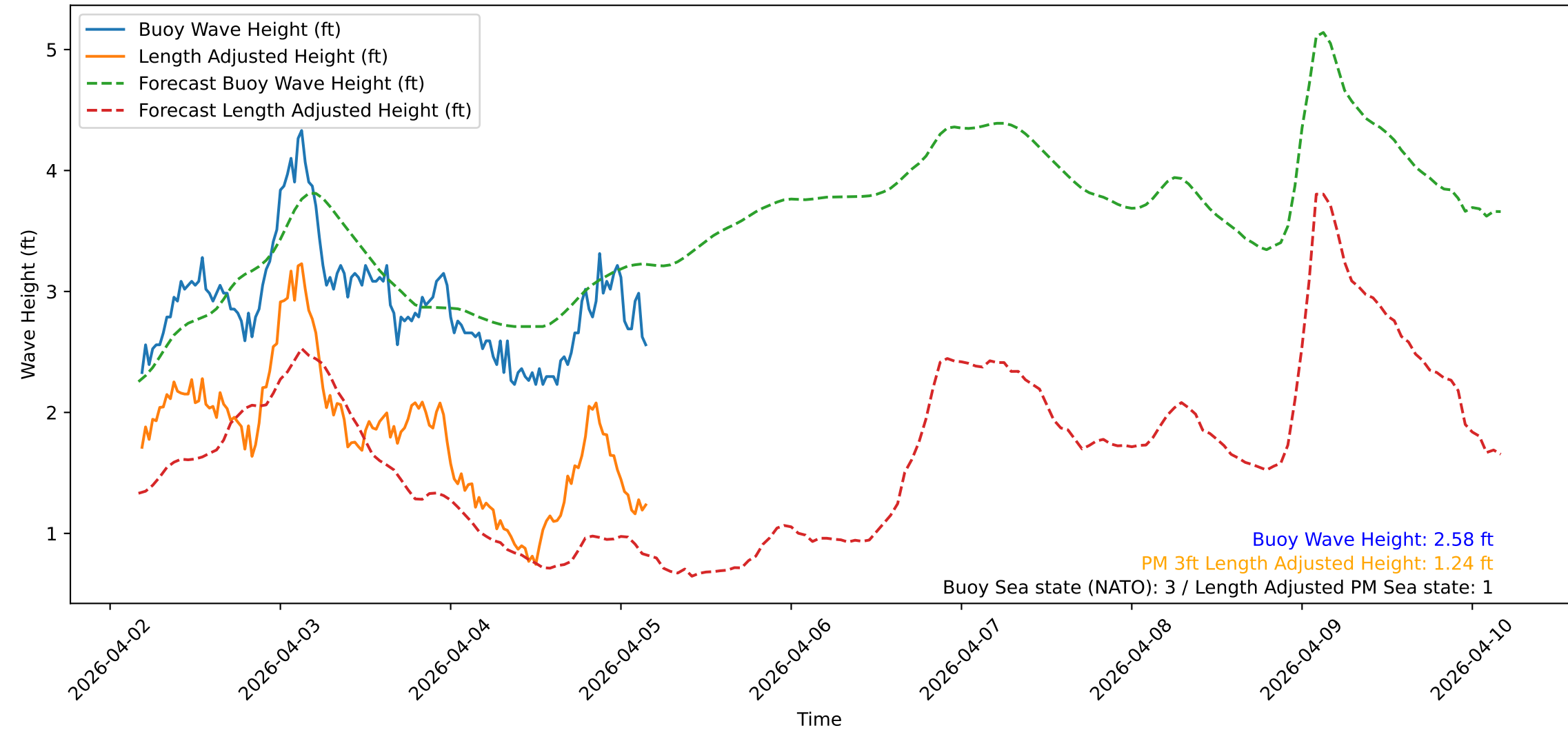
Wave Heights over Time for Green Beach at 2026-04-05 04:21:09
