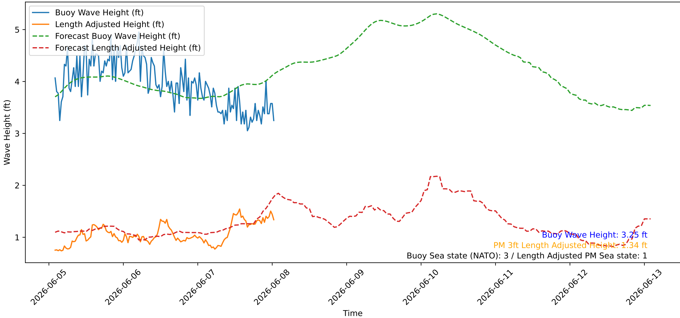
Wave Heights over Time for Red Beach at 2026-06-08 01:30:46
