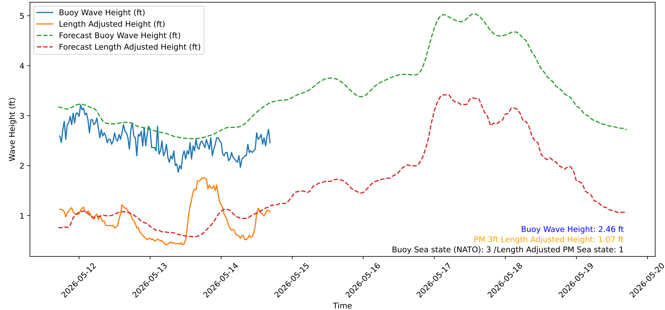
Wave Heights over Time for Red Beach at 2026-05-14 17:10:52
