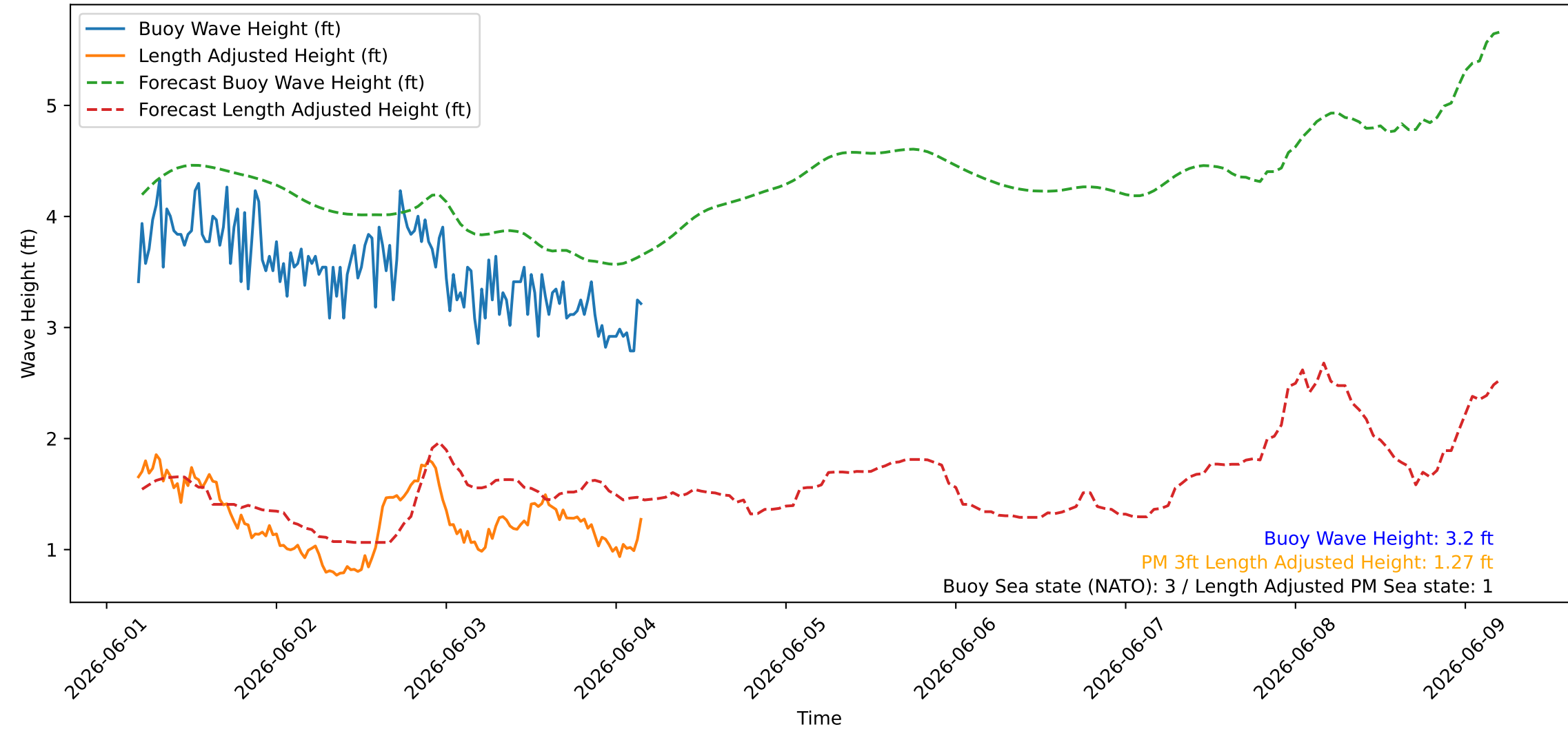
Wave Heights over Time for Green Beach at 2026-06-04 04:31:08
