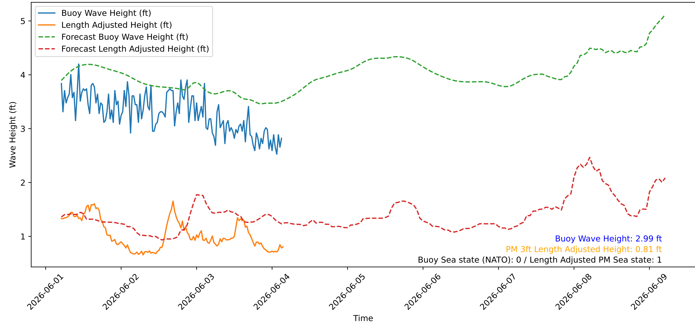
Wave Heights over Time for Red Beach at 2026-06-04 04:30:45
