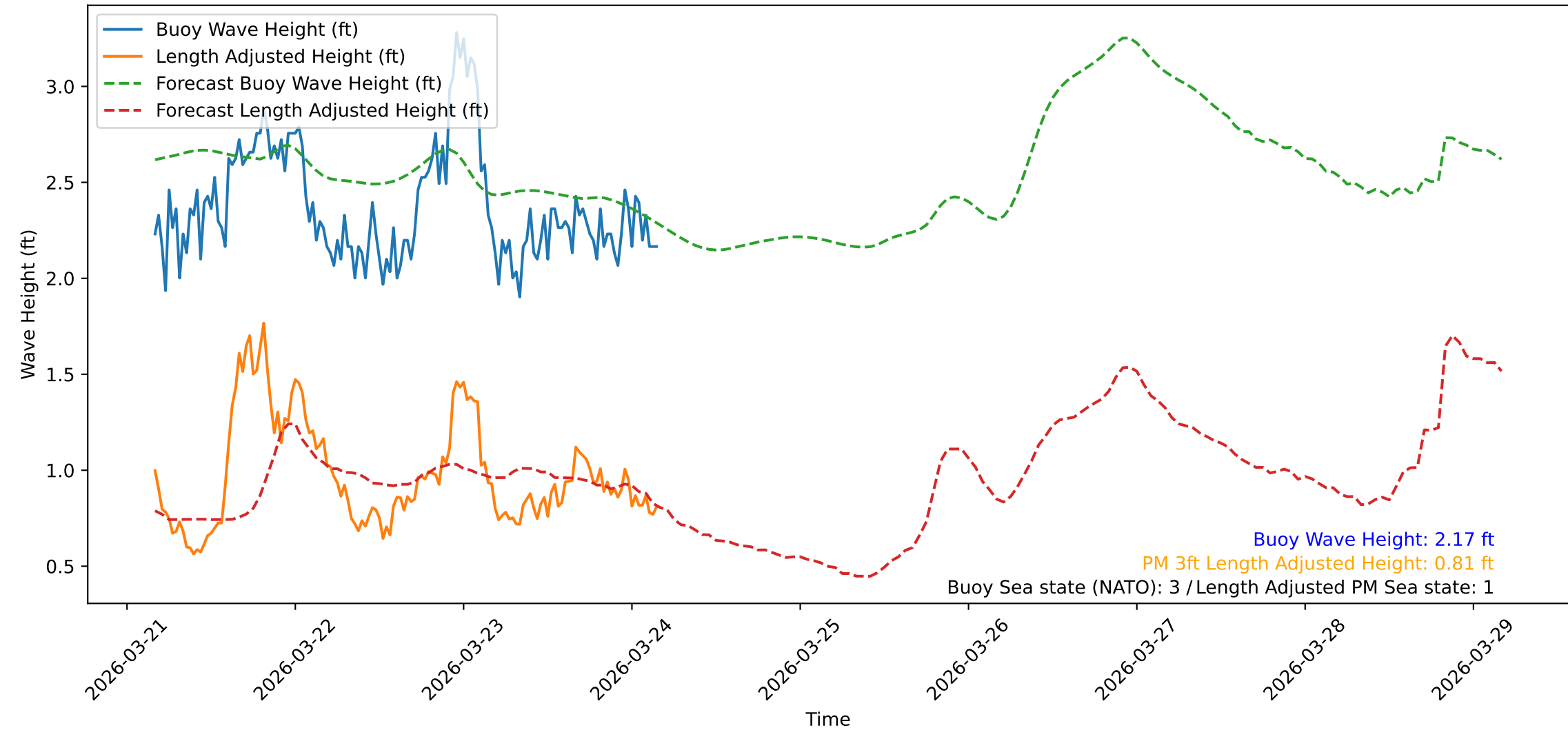
Wave Heights over Time for Green Beach at 2026-03-24 04:11:09
