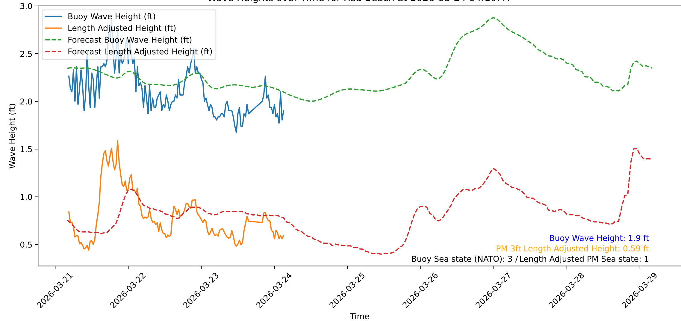
Wave Heights over Time for Red Beach at 2026-03-24 04:10:47
