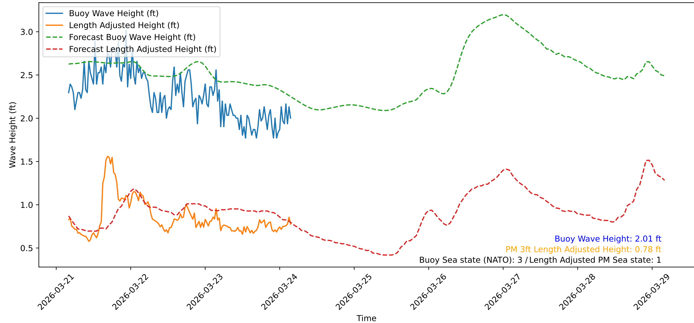
Wave Heights over Time for Oceanside Harbor at 2026-03-24 04:10:31
