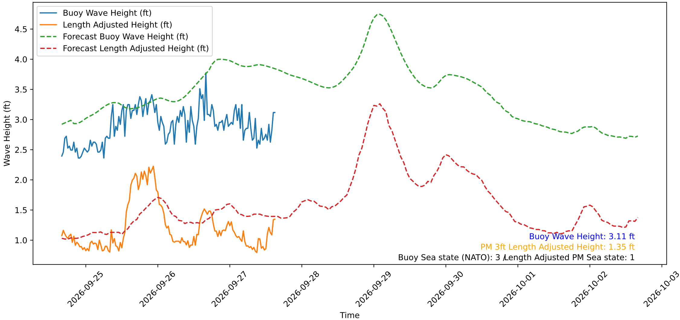
Wave Heights over Time for Oceanside Harbor at 2026-09-27 15:50:30
