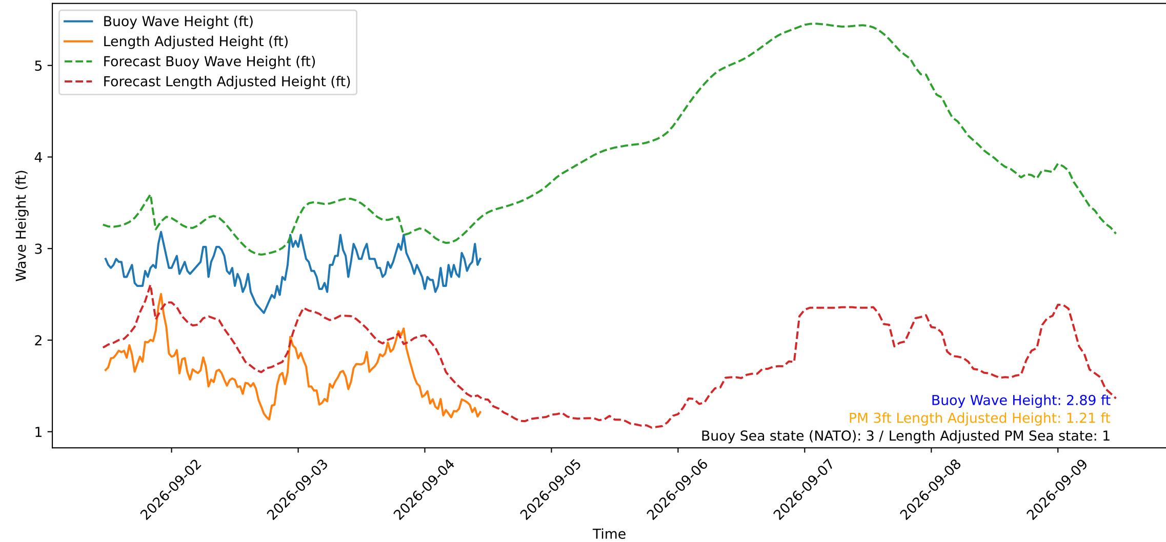
Wave Heights over Time for Red Beach at 2026-09-04 11:10:50
