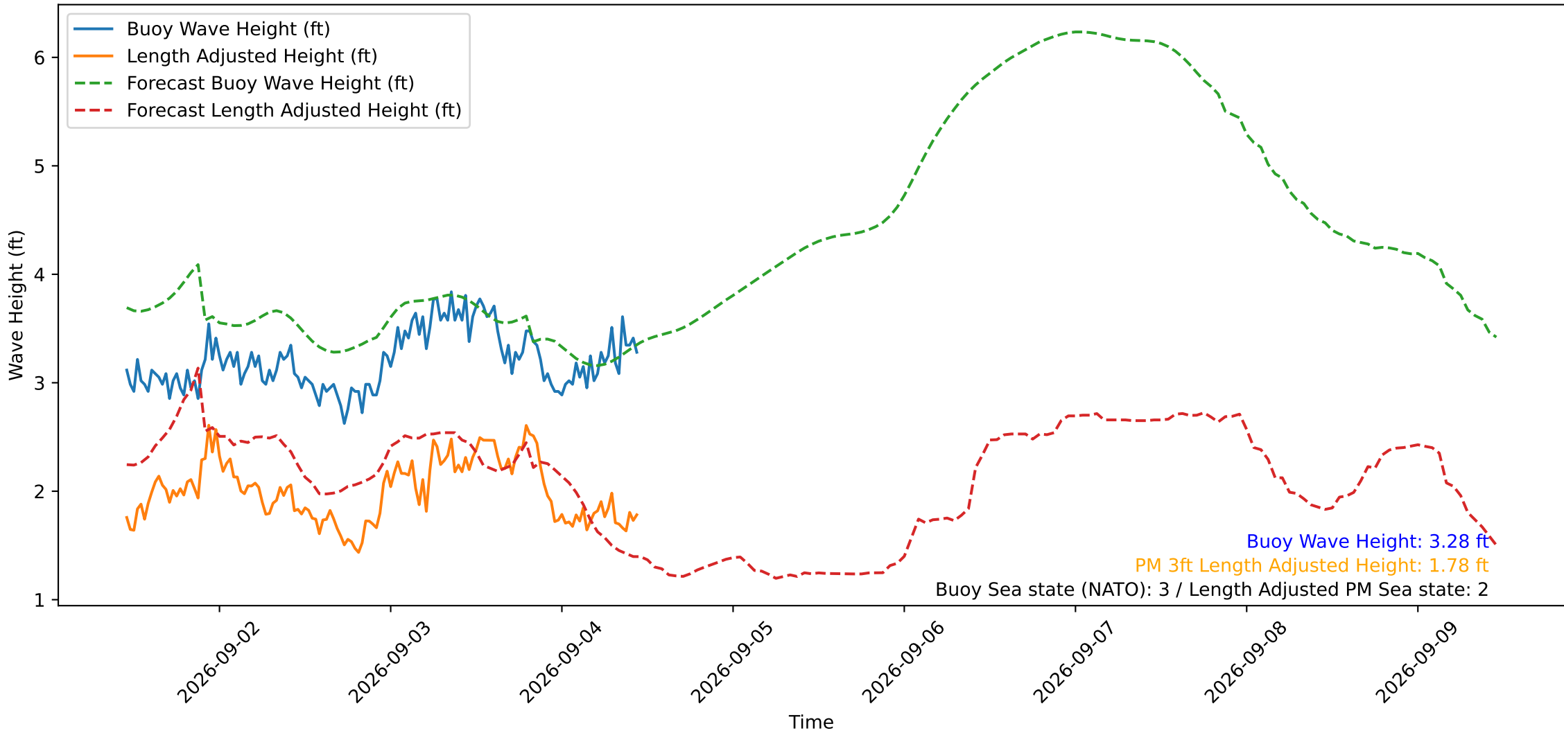
Wave Heights over Time for Oceanside Harbor at 2026-09-04 11:10:30
