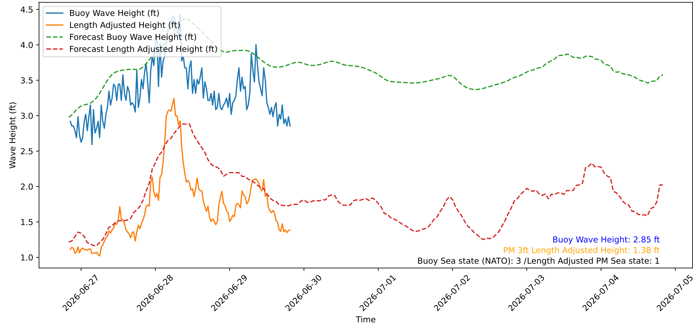
Wave Heights over Time for Oceanside Harbor at 2026-06-29 20:20:26
