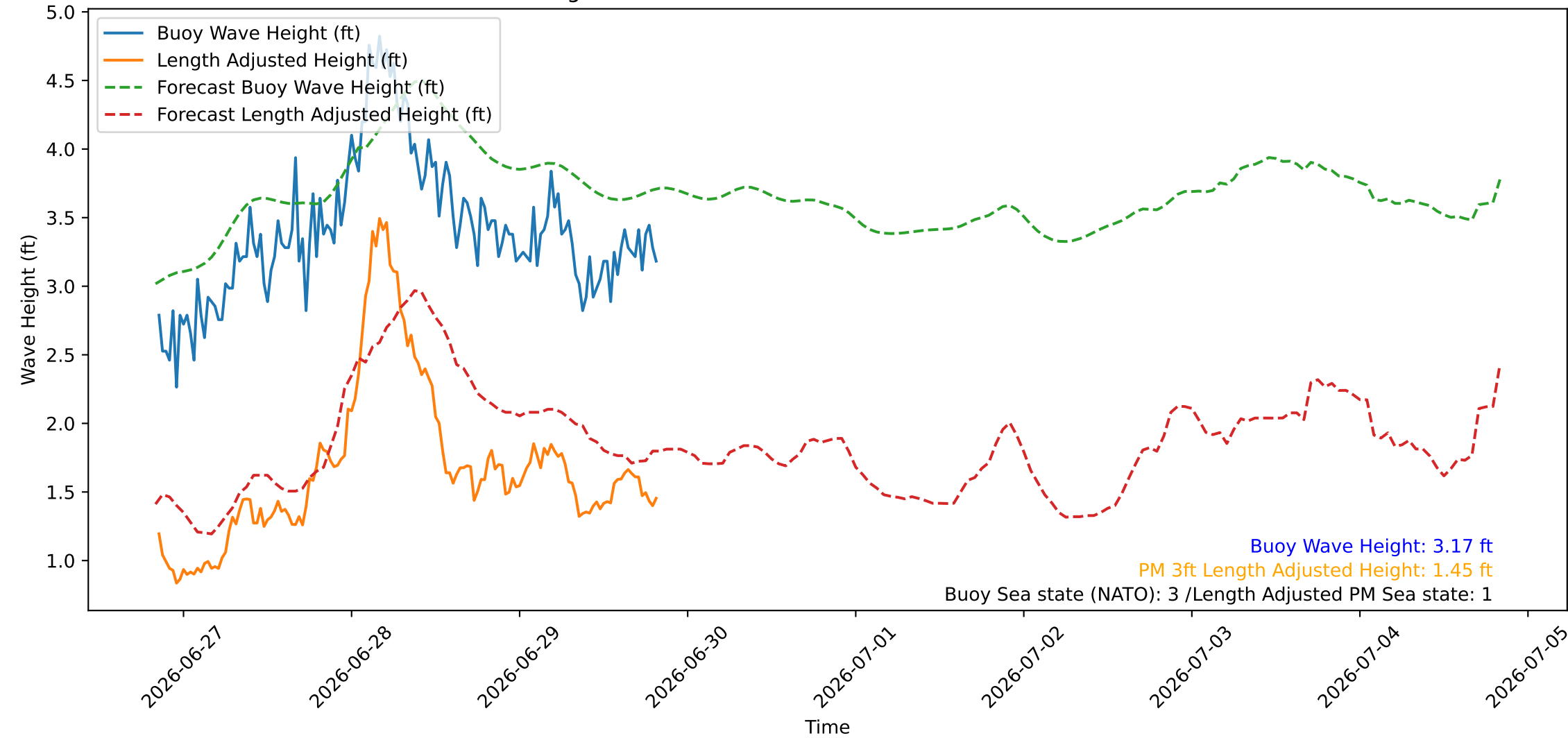
Wave Heights over Time for Green Beach at 2026-06-29 20:21:09
