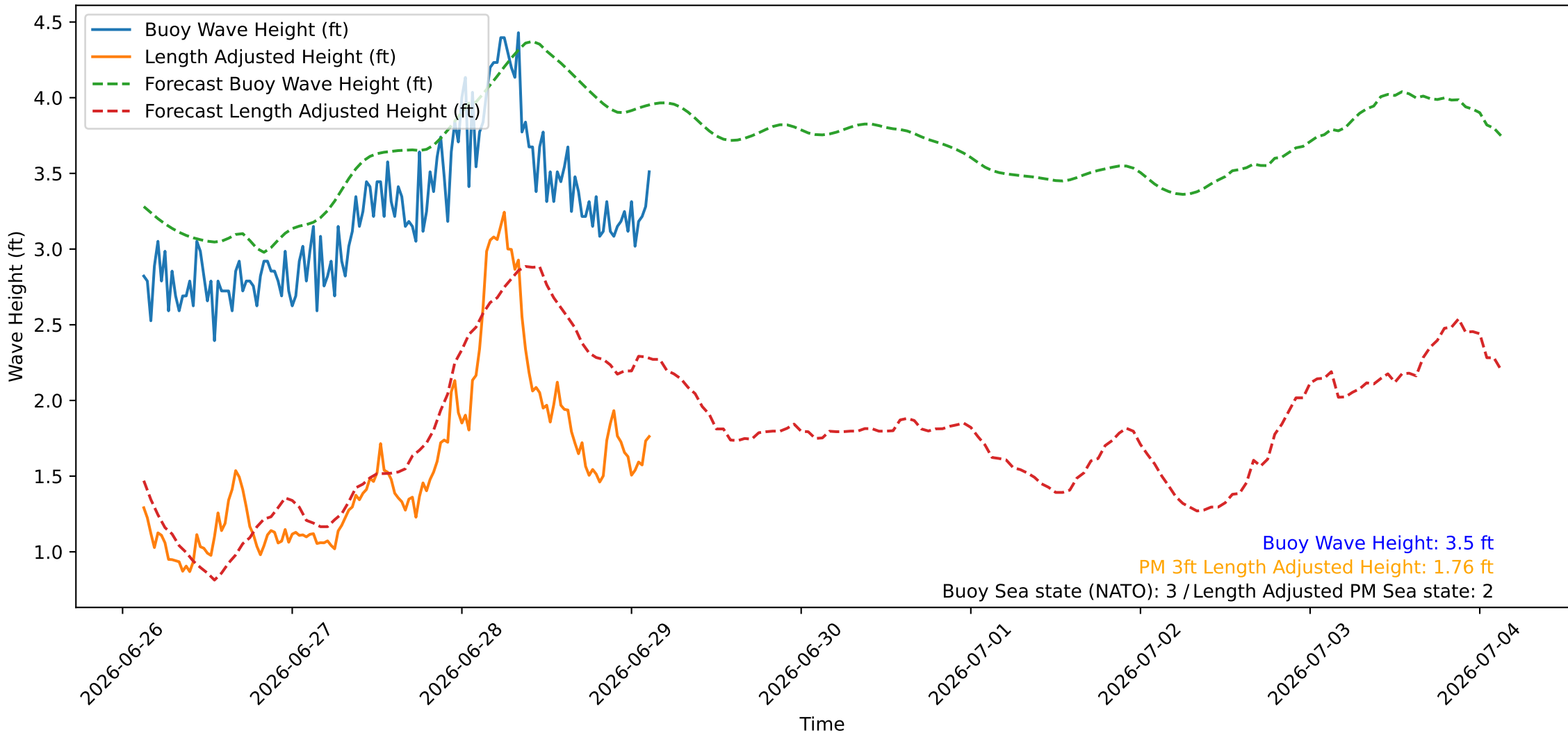
Wave Heights over Time for Oceanside Harbor at 2026-06-29 03:10:26
