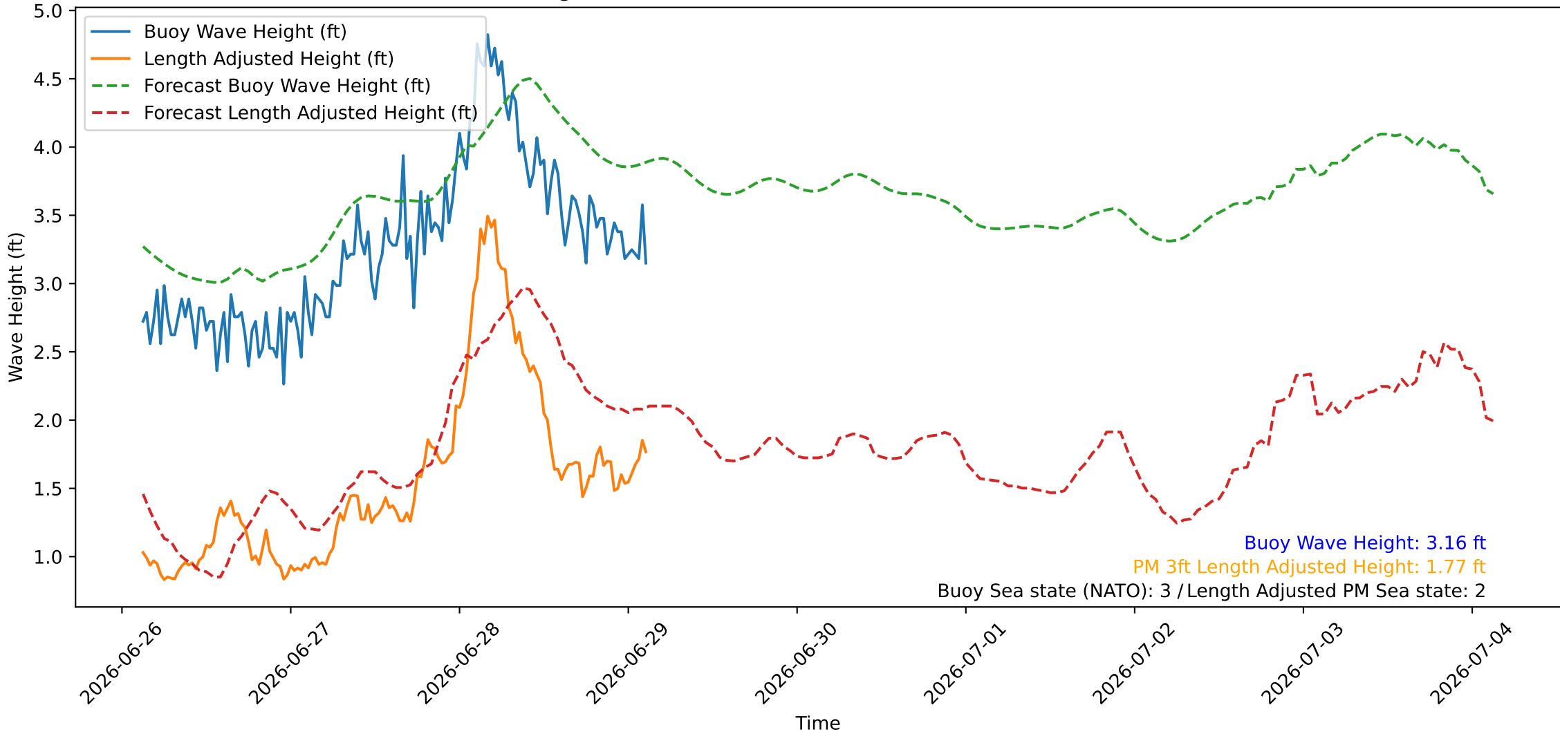
Wave Heights over Time for Green Beach at 2026-06-29 03:11:08
