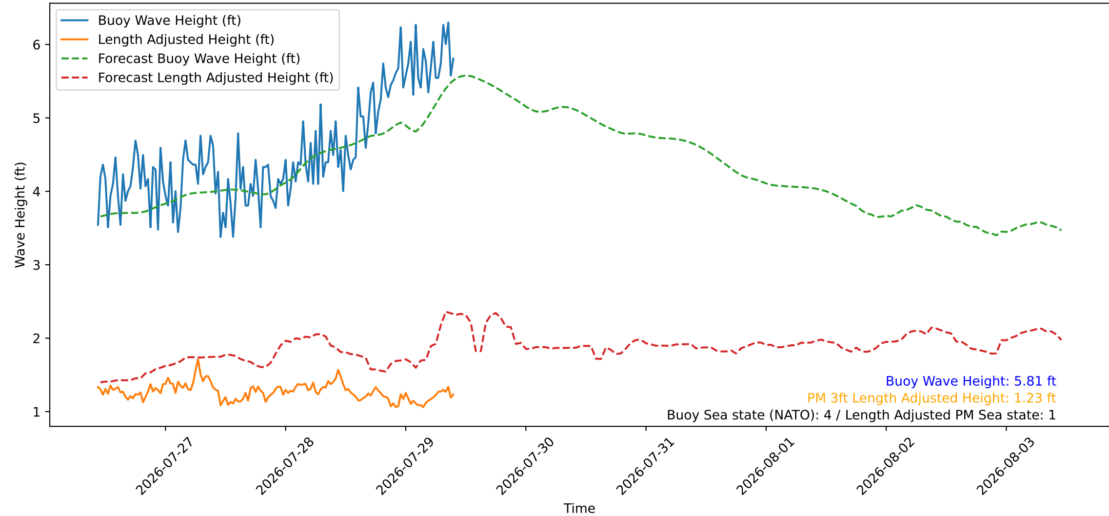
Wave Heights over Time for Green Beach at 2026-07-29 10:31:09
