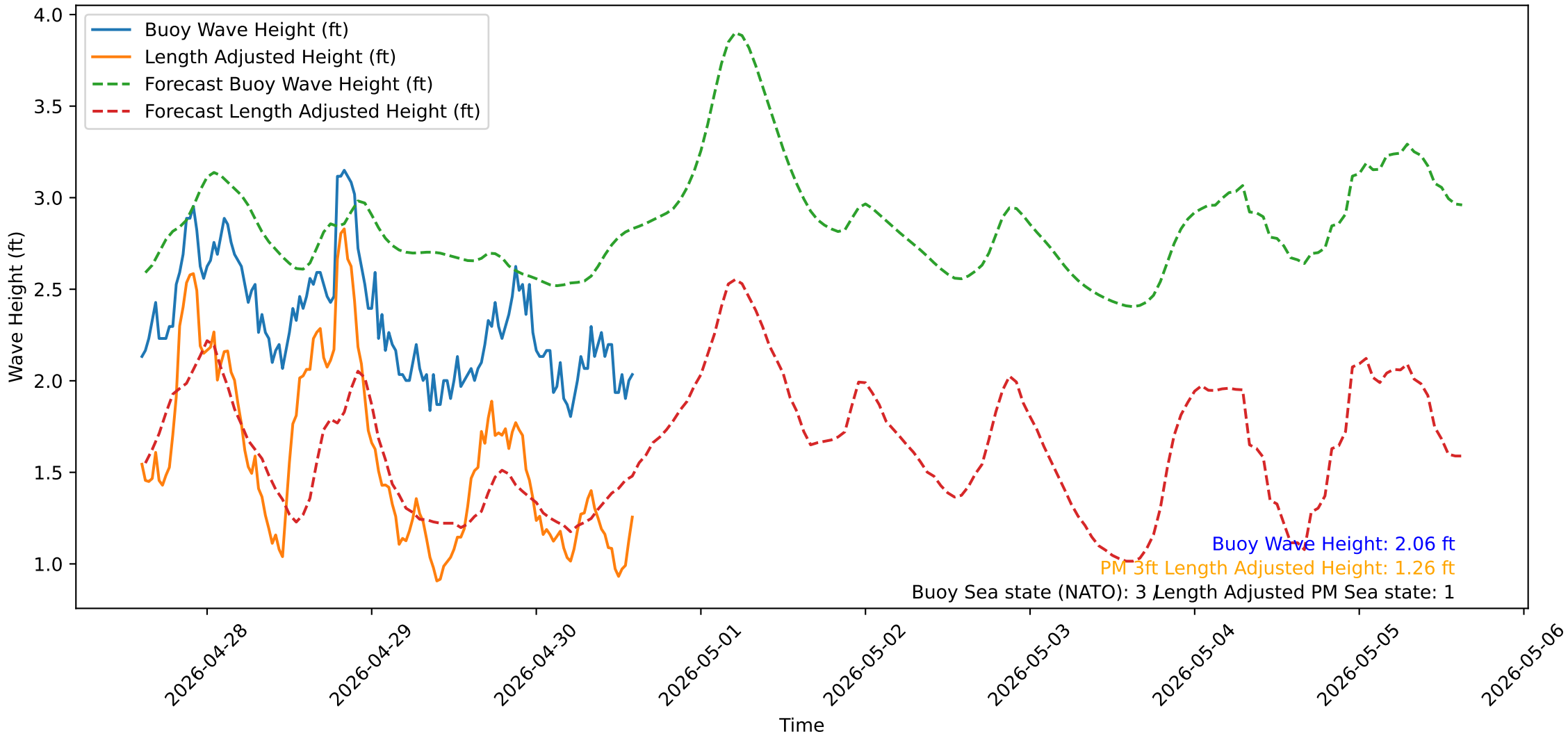
Wave Heights over Time for Green Beach at 2026-04-30 14:41:13
