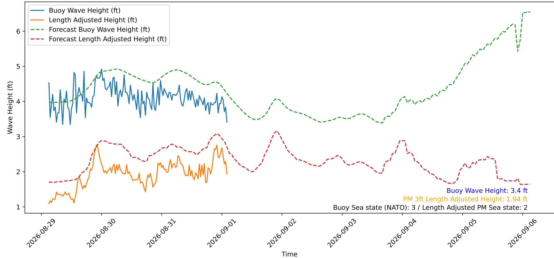
Wave Heights over Time for Green Beach at 2026-09-01 02:41:13
