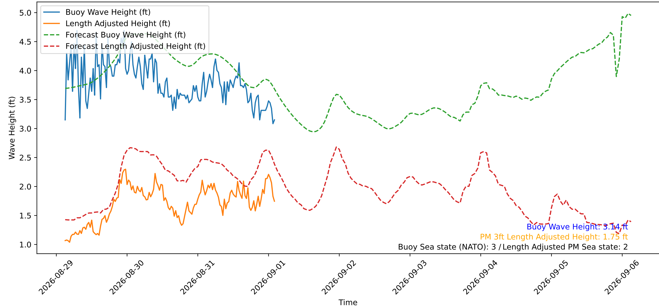
Wave Heights over Time for Red Beach at 2026-09-01 02:40:50
