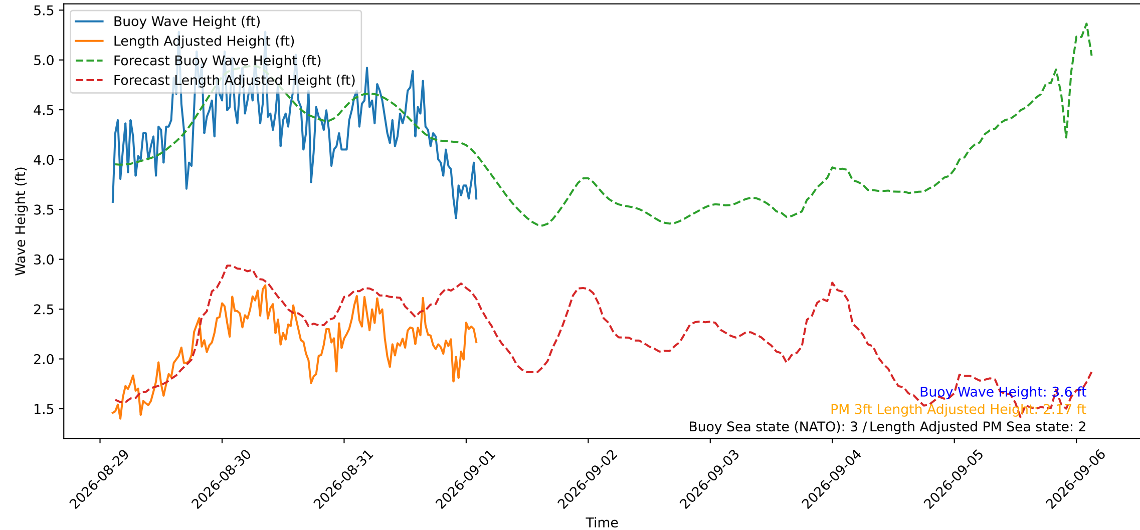
Wave Heights over Time for Oceanside Harbor at 2026-09-01 02:40:30
