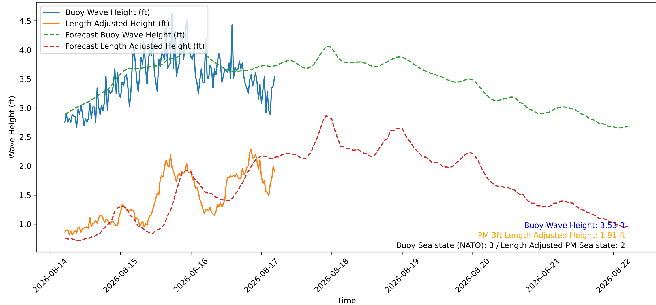
Wave Heights over Time for Oceanside Harbor at 2026-08-17 05:10:27
