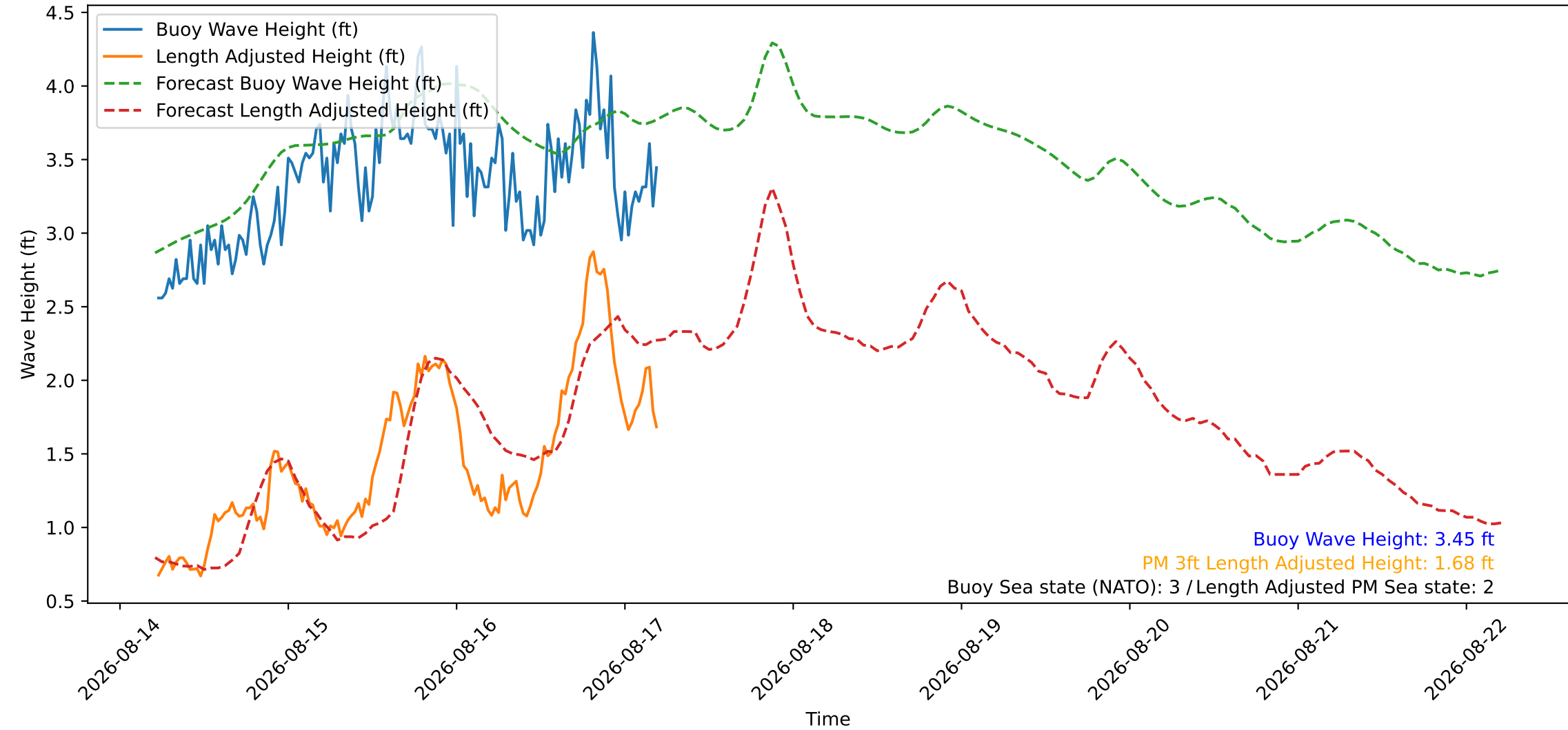
Wave Heights over Time for Green Beach at 2026-08-17 05:11:09
