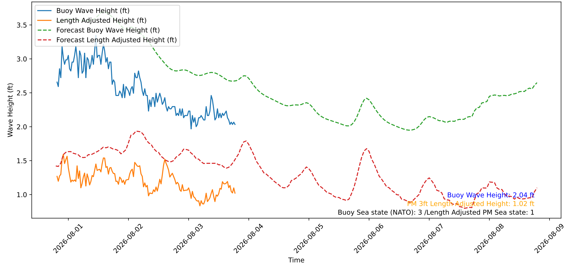
Wave Heights over Time for Red Beach at 2026-08-03 19:20:48
