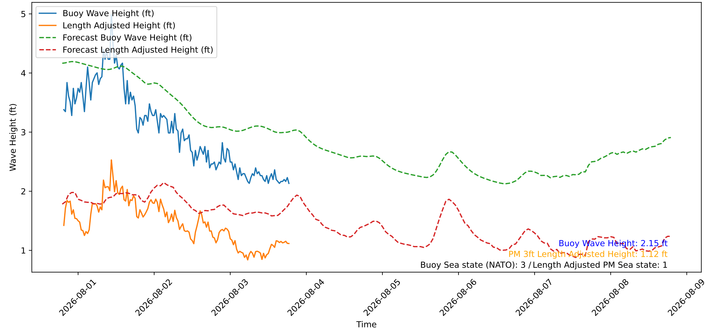
Wave Heights over Time for Green Beach at 2026-08-03 19:21:10
