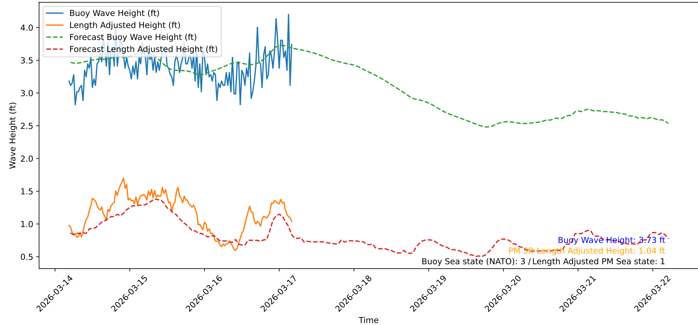
Wave Heights over Time for Green Beach at 2026-03-17 04:41:50
