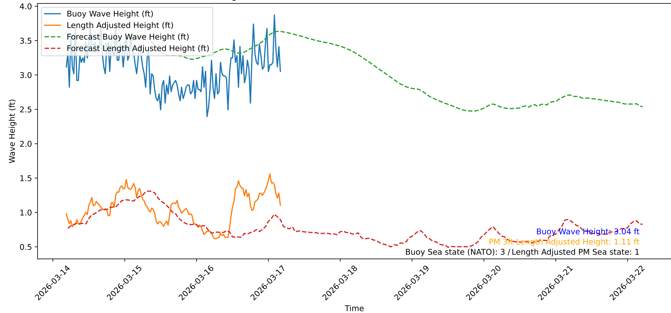
Wave Heights over Time for Oceanside Harbor at 2026-03-17 04:40:47
