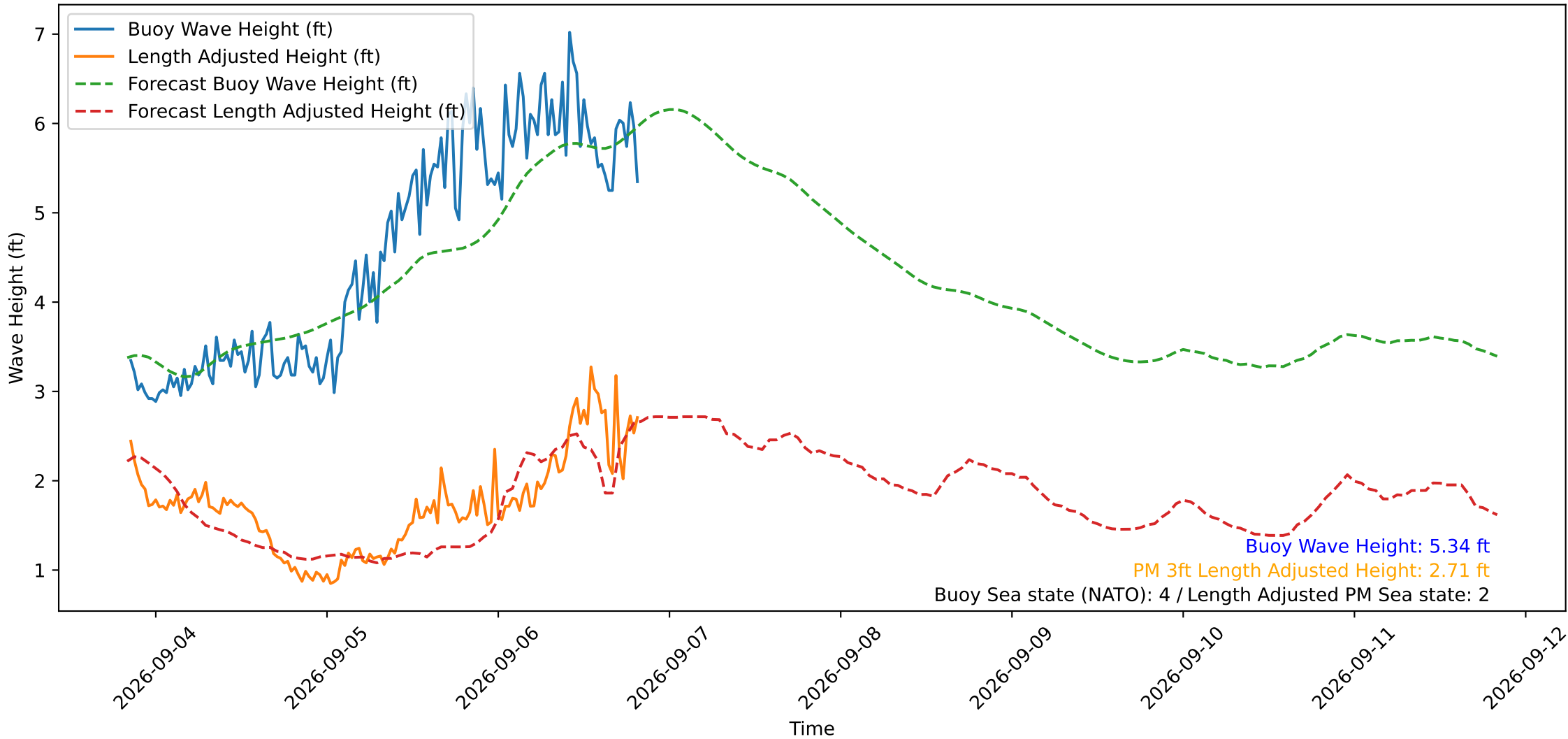
Wave Heights over Time for Oceanside Harbor at 2026-09-06 20:20:30
