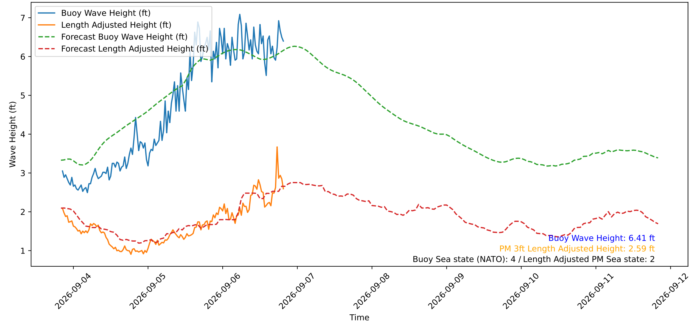
Wave Heights over Time for Green Beach at 2026-09-06 20:21:16
