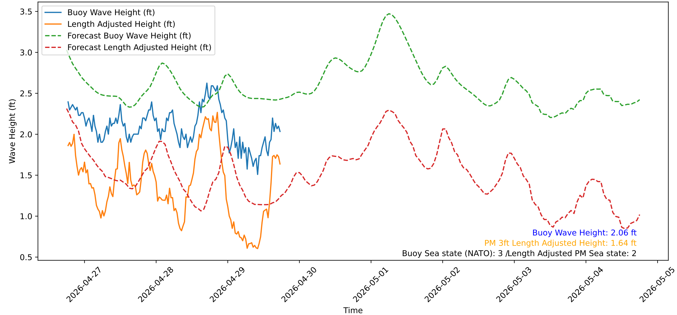
Wave Heights over Time for Red Beach at 2026-04-29 18:10:50
