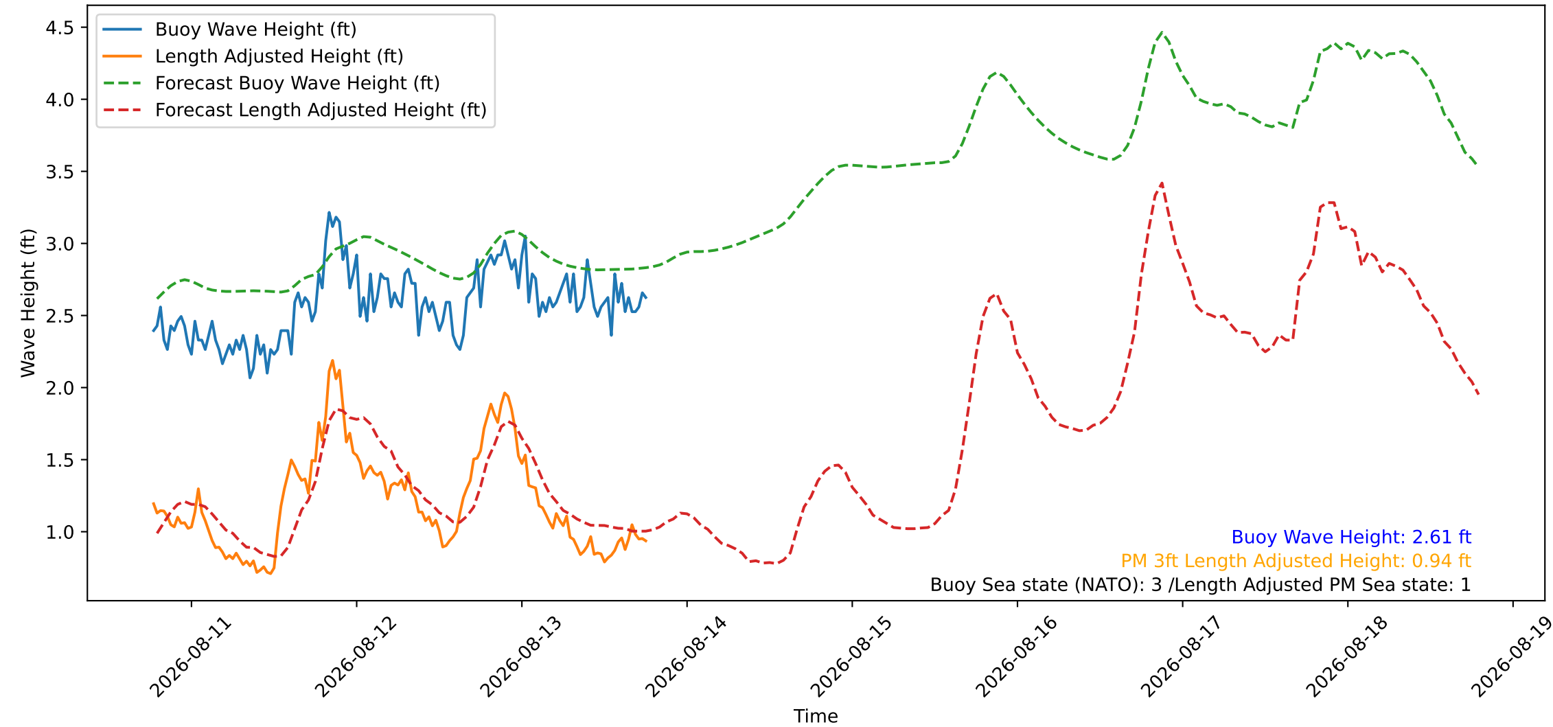
Wave Heights over Time for Green Beach at 2026-08-13 18:41:09
