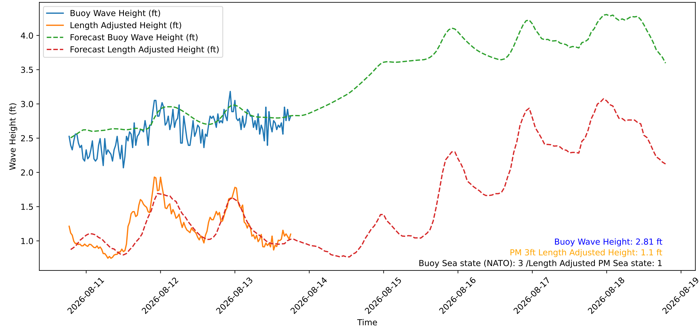
Wave Heights over Time for Oceanside Harbor at 2026-08-13 18:40:26
