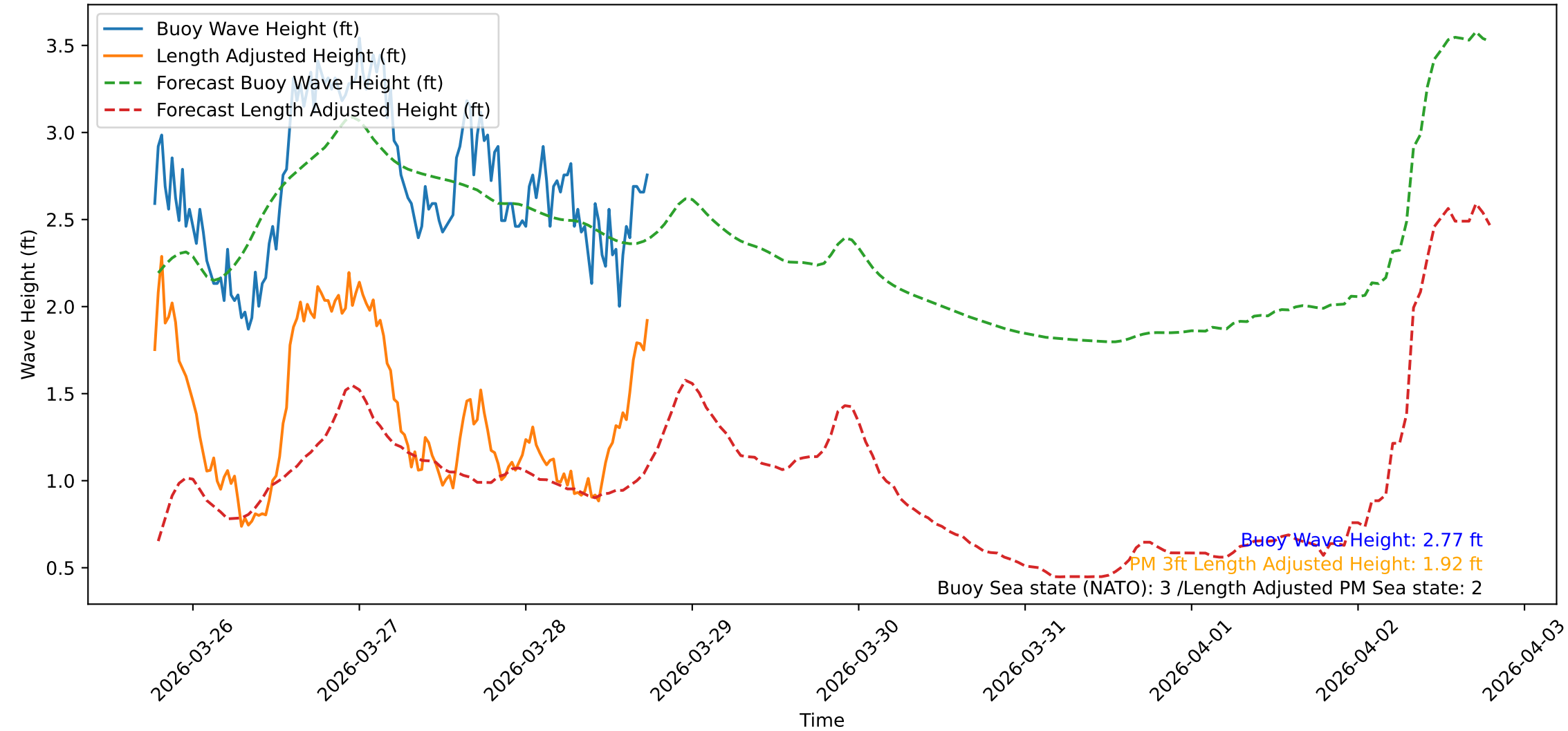
Wave Heights over Time for Green Beach at 2026-03-28 18:31:10
