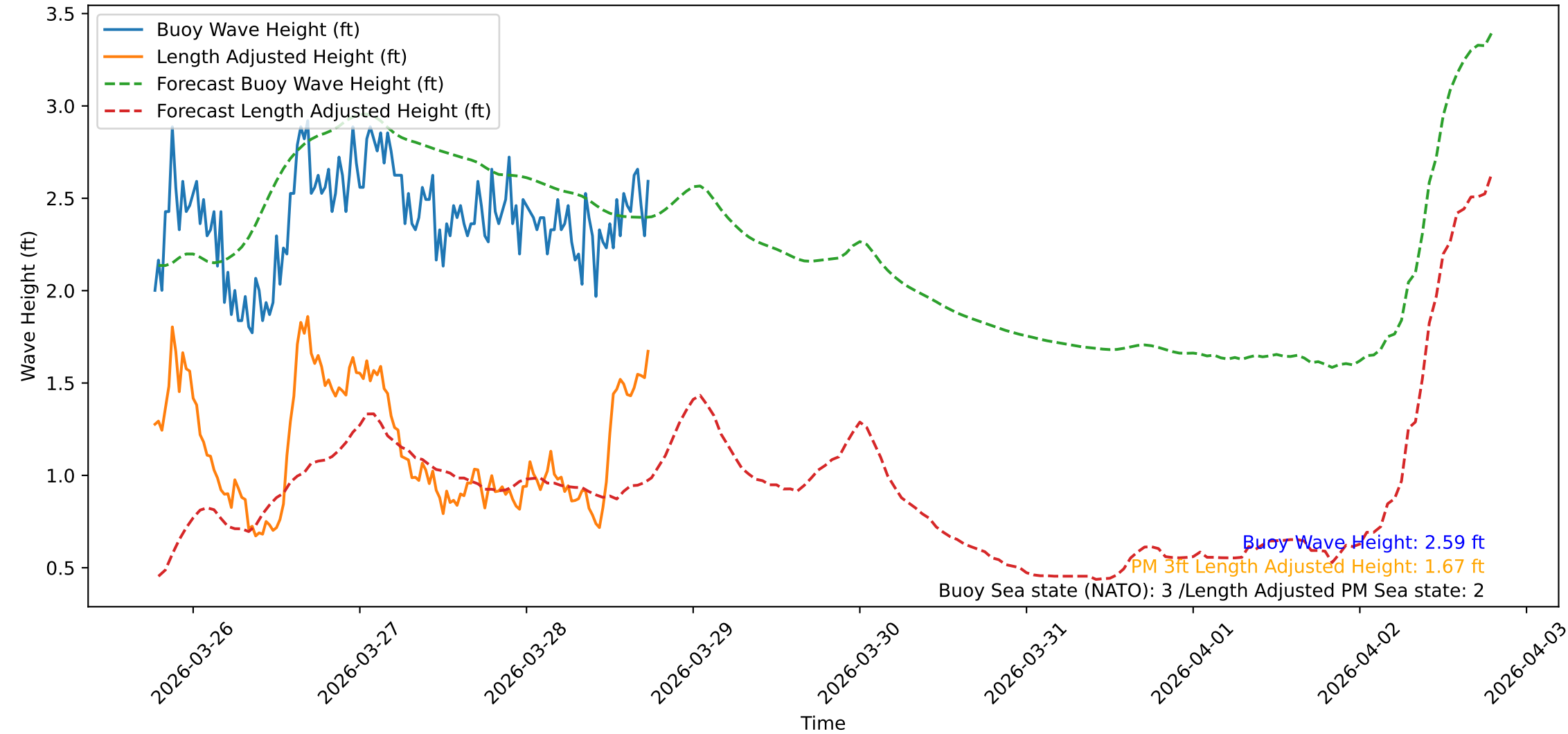
Wave Heights over Time for Oceanside Harbor at 2026-03-28 18:30:32
