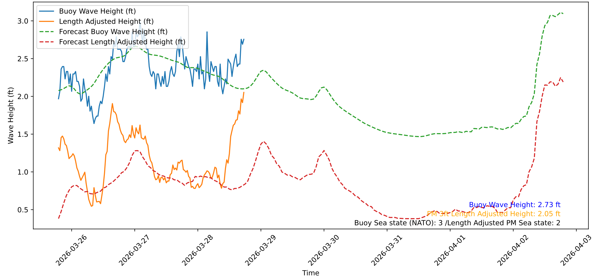
Wave Heights over Time for Red Beach at 2026-03-28 18:30:48
